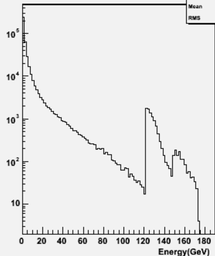
Particle Energy : w104002 aa_n3e3du_o
