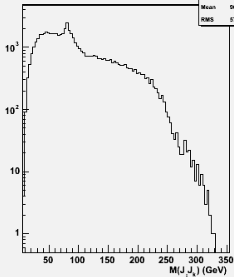
2jets mass(All comb)w104002 aa_n3e3du_o
