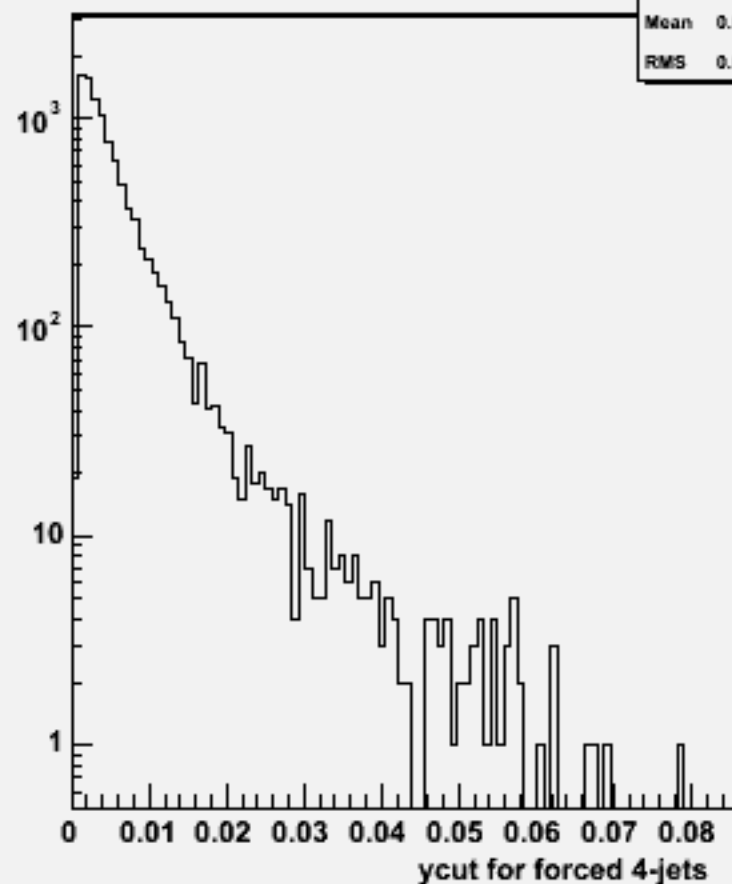
Ycut for 4-jets :w104002 aa_n3e3du_o
