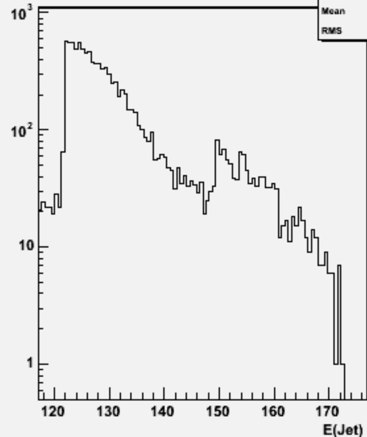
Jet energies(All jets)w104002 aa_n3e3du_o
