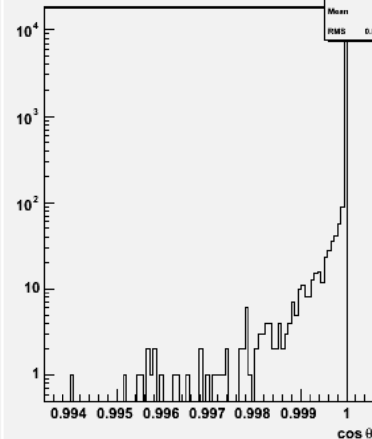
Jet cos \theta (All jets)w104002 aa_n3e3du_o
