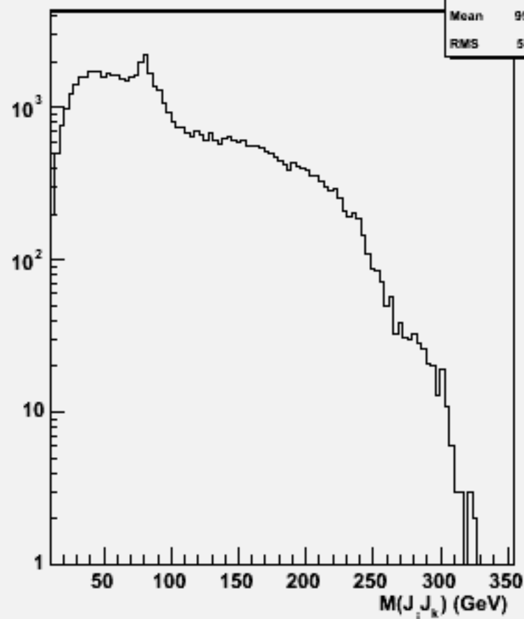
2jets mass(All comb)w104001 aa_n3e3du_o
