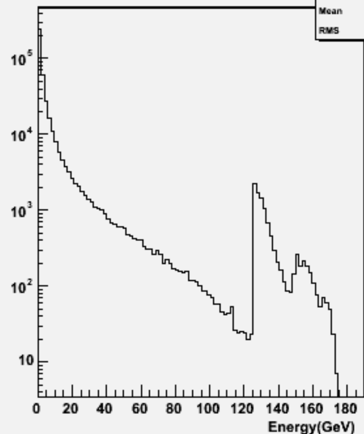
Particle Energy : w104001 aa_n3e3du_o
