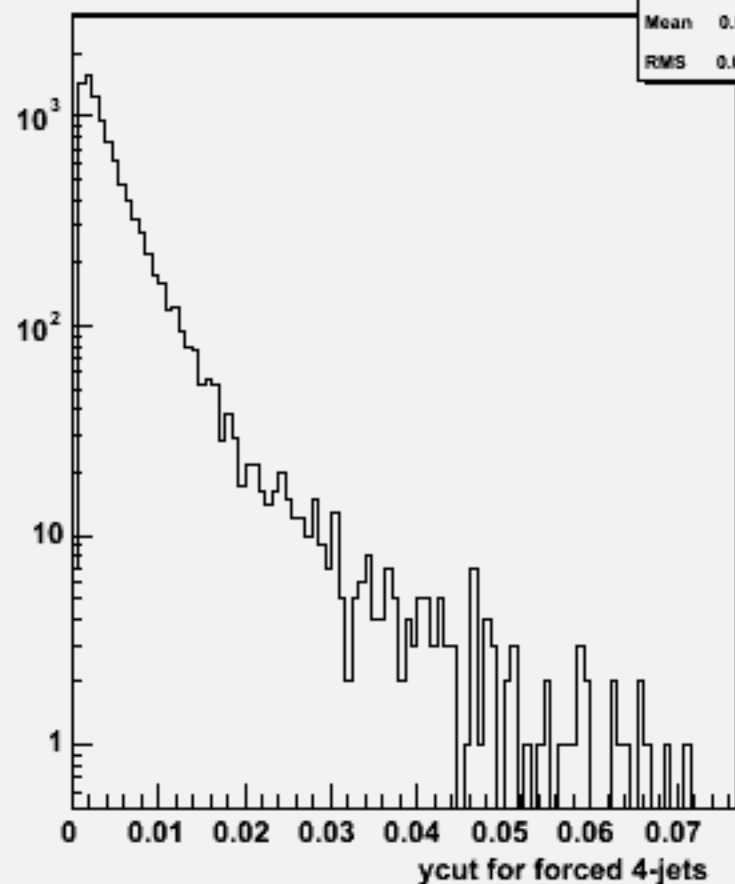
Ycut for 4-jets :w104001 aa_n3e3du_o
