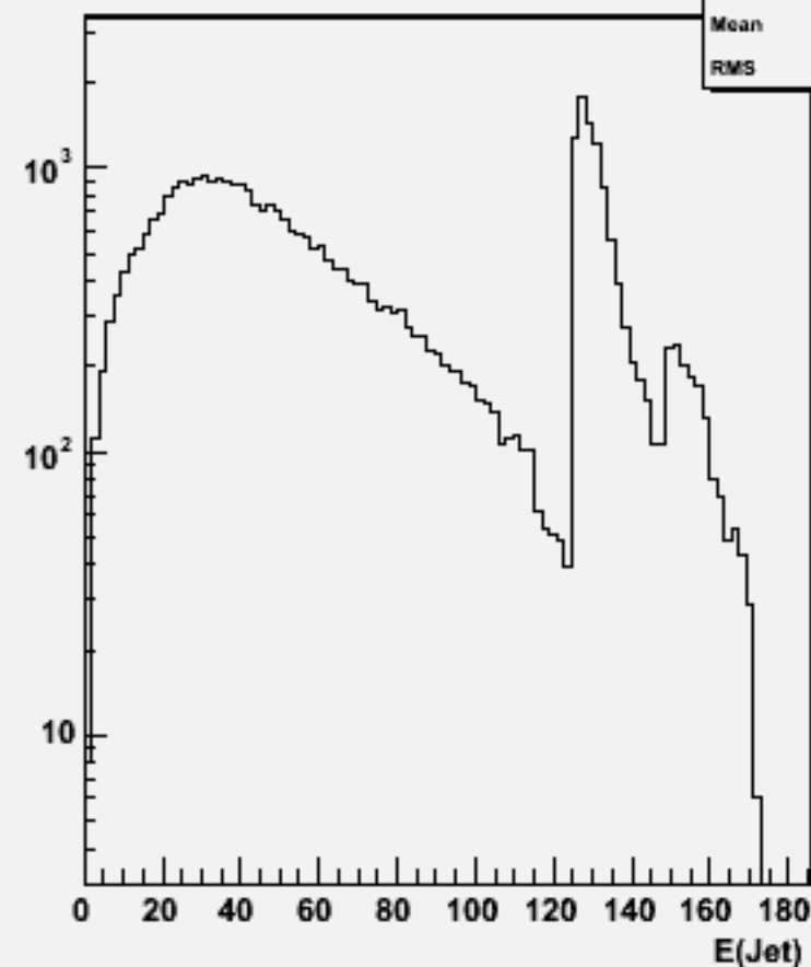
Jet energies(All jets)w104001 aa_n3e3du_o
