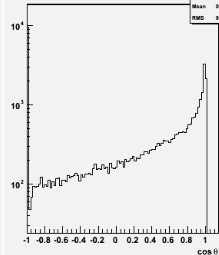
Jet cos \theta (All jets)w104001 aa_n3e3du_o
