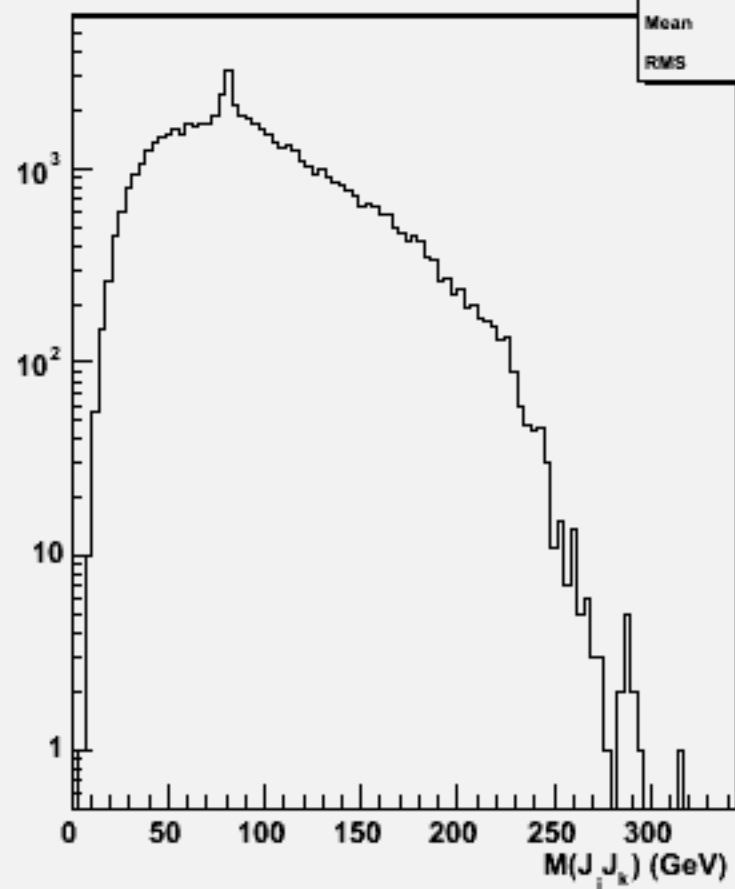
2jets mass(All comb)w104000 aa_n3e3du_o
