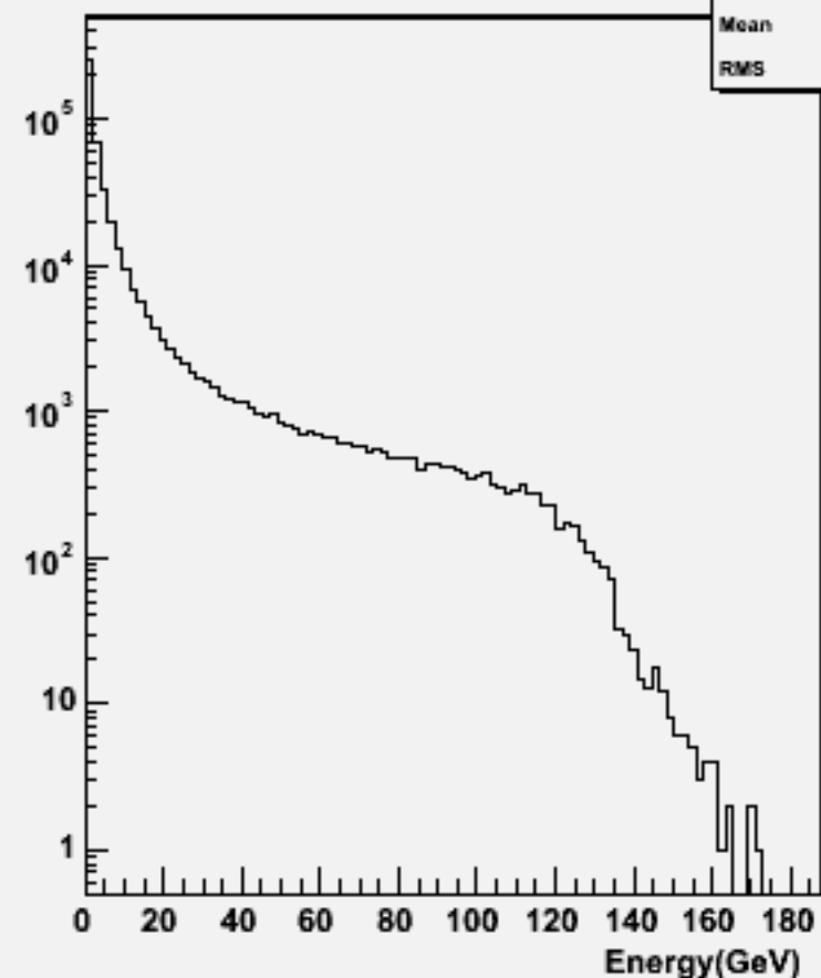
Particle Energy : w104000 aa_n3e3du_o
