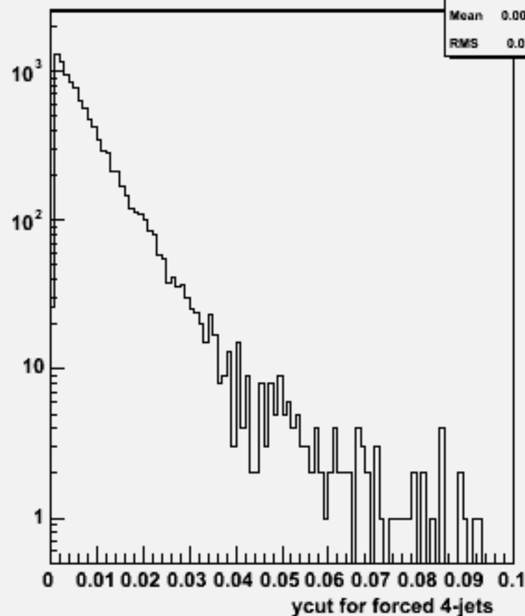
Ycut for 4-jets :w104000 aa_n3e3du_o
