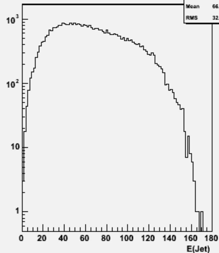
Jet energies(All jets)w104000 aa_n3e3du_o
