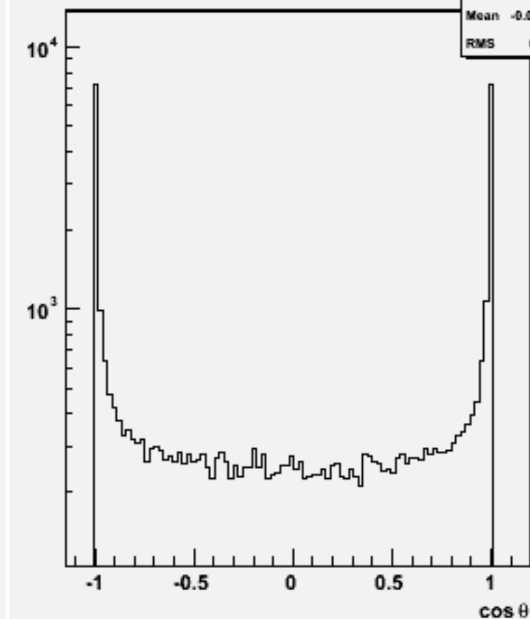
Jet cos \theta (All jets)w104000 aa_n3e3du_o
