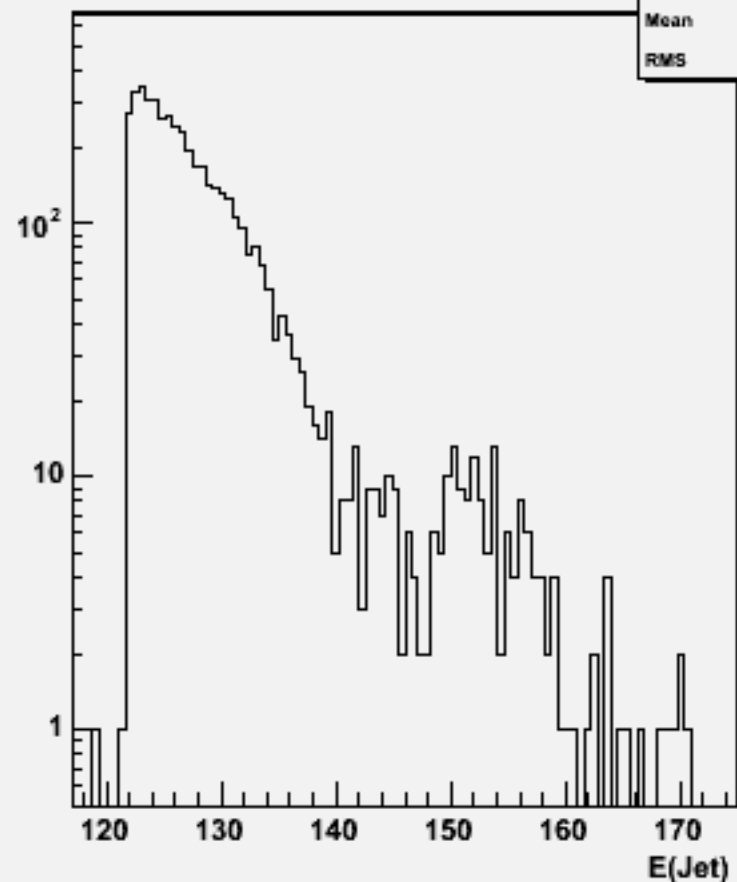
Jet energies(All jets)w103998 aa_n3e3e3n3_o
