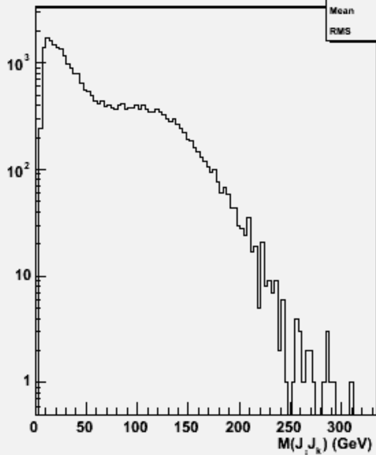
2jets mass(All comb)w103998 aa_n3e3e3n3_o
