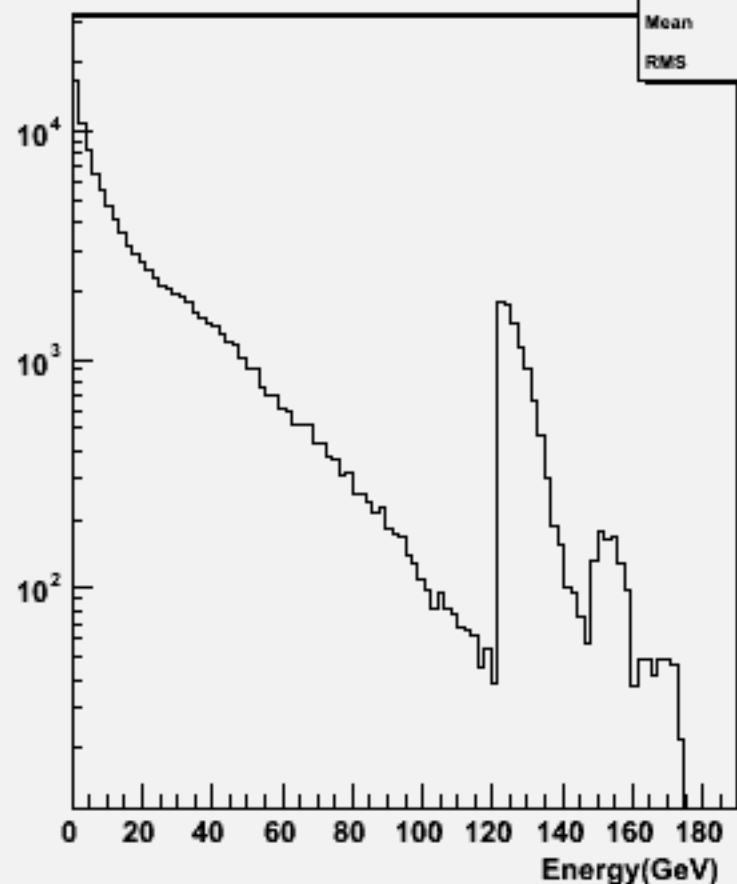
Particle Energy : w103998 aa_n3e3e3n3_o
