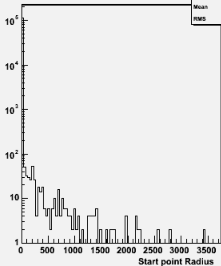
Start point R : w103998 aa_n3e3e3n3_o
