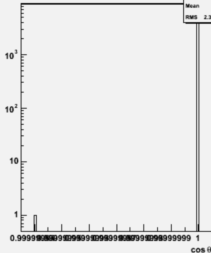
Jet cosθ (All jets)w103998 aa_n3e3e3n3_o
