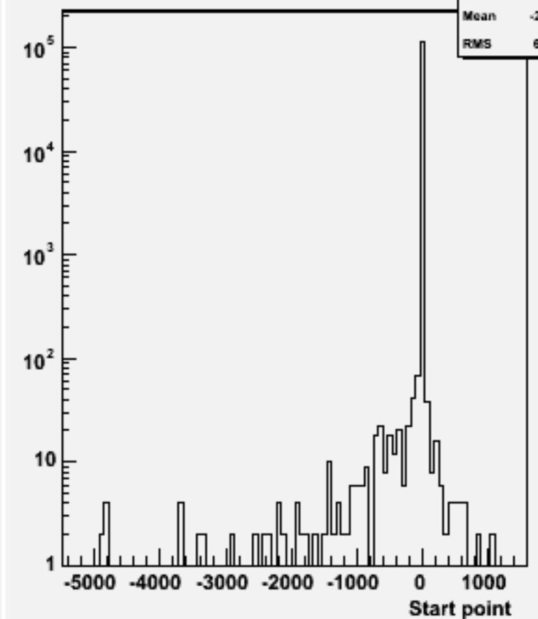
Start point Z : w103998 aa_n3e3e3n3_o
