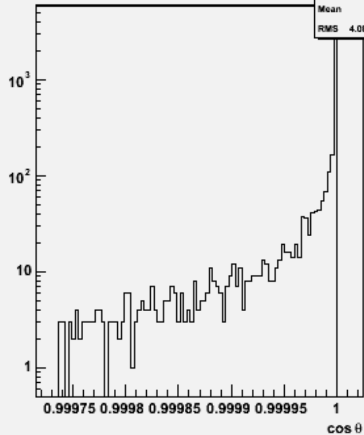
Jet cosθ (All jets)w103997 aa_n3e3e3n3_o
