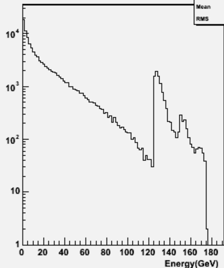
Start point R : w103997 aa_n3e3e3n3_o
