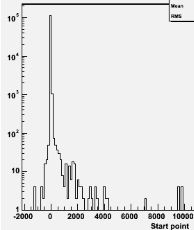
Start point Z : w103997 aa_n3e3e3n3_o
