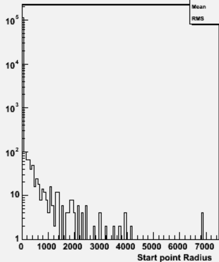
Start point R : w103997 aa_n3e3e3n3_o
