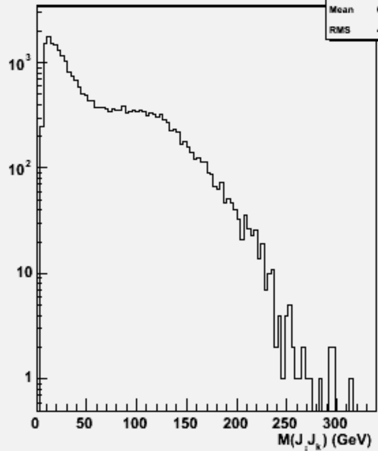
2jets mass(All comb)w103997 aa_n3e3e3n3_o
