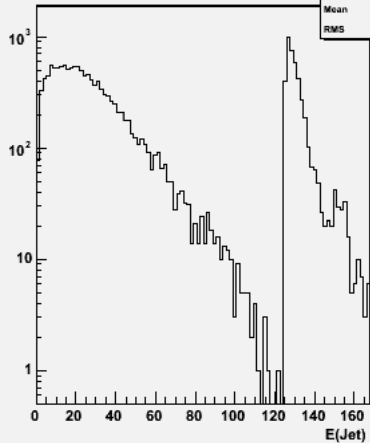
Jet energies(All jets)w103997 aa_n3e3e3n3_o
