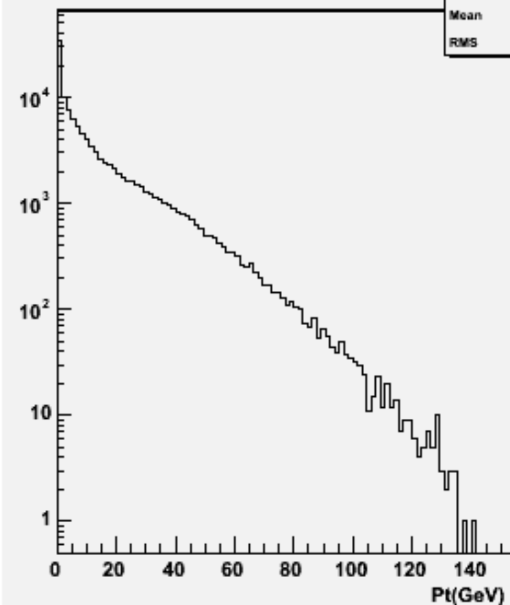
Start point Z : w103996 aa_n3e3e3n3_o
