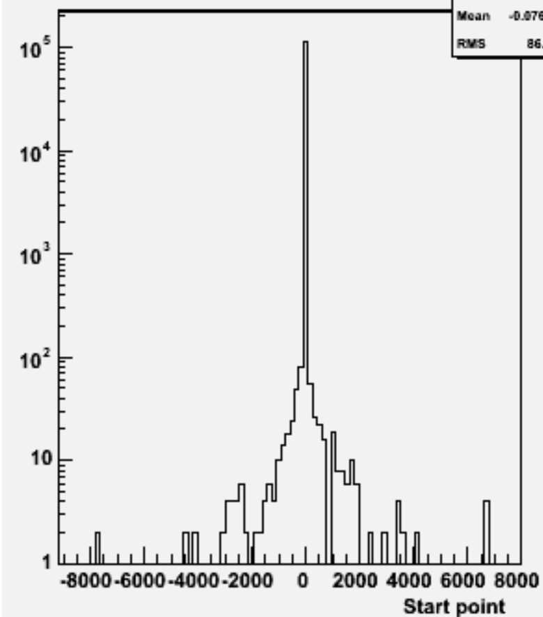
Start point Z : w103996 aa_n3e3e3n3_o
