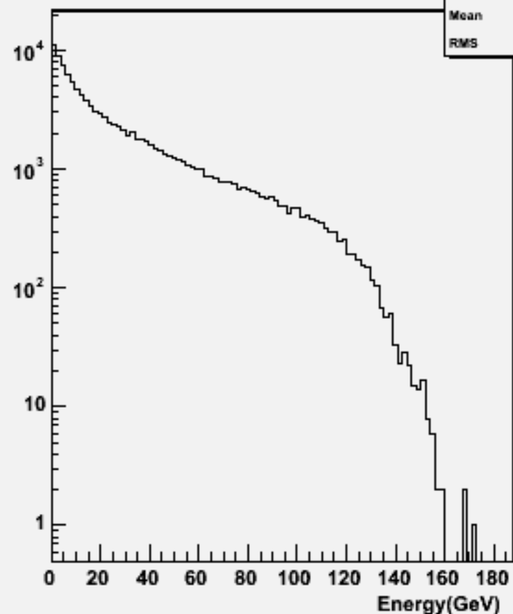
Start point R : w103996 aa_n3e3e3n3_o
