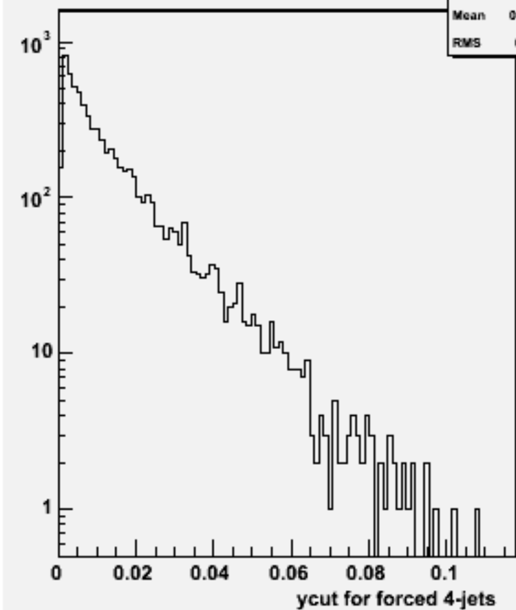
Ycut for 4-jets :w103996 aa_n3e3e3n3_o
