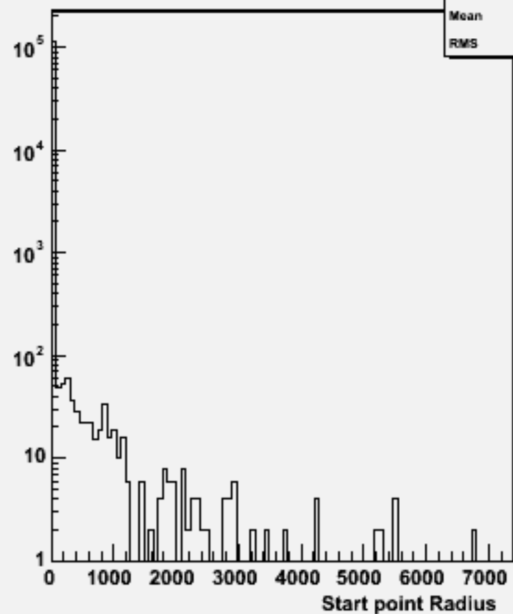
Start point R : w103996 aa_n3e3e3n3_o
