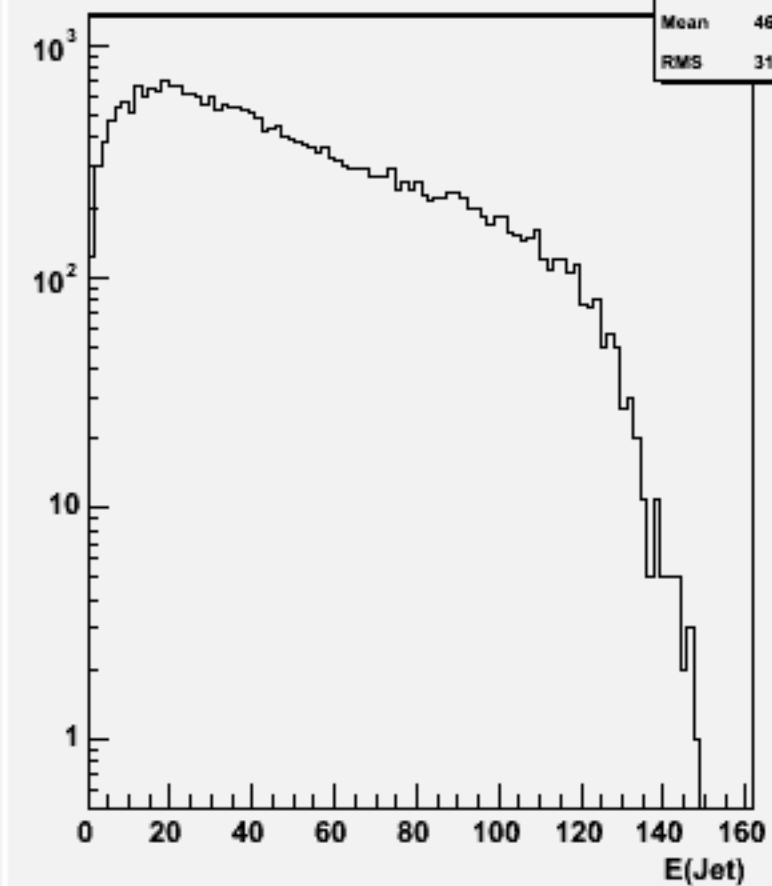
Jet energies(All jets)w103996 aa_n3e3e3n3_o
