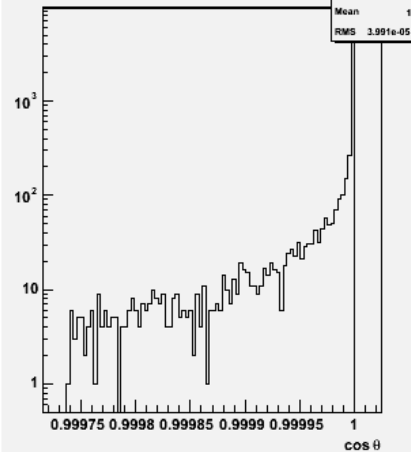
Jet cosθ (All jets)w103996 aa_n3e3e3n3_o
