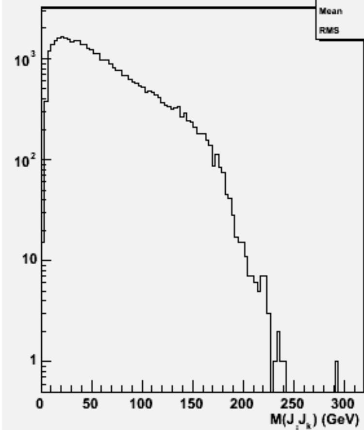
2jets mass(All comb)w103996 aa_n3e3e3n3_o
