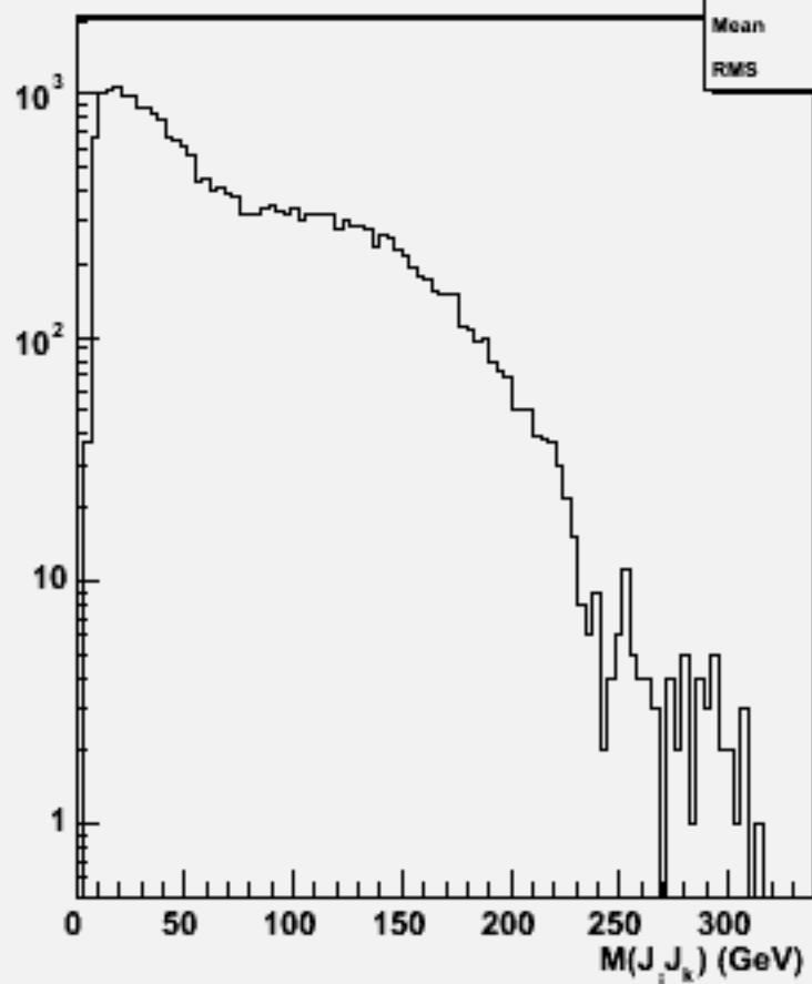
2jets mass(All comb)w103994 aa_n3e3e2n2_o
