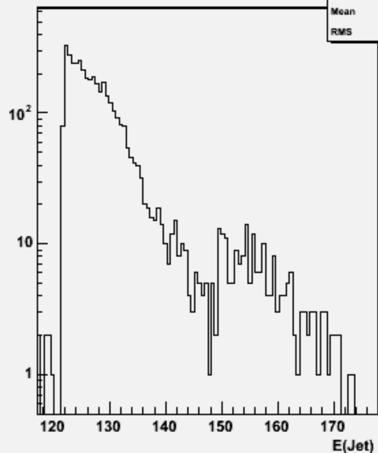
Jet energies(All jets)w103994 aa_n3e3e2n2_o
