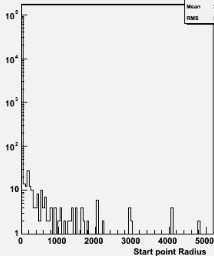
Start point R : w103994 aa_n3e3e2n2_o
