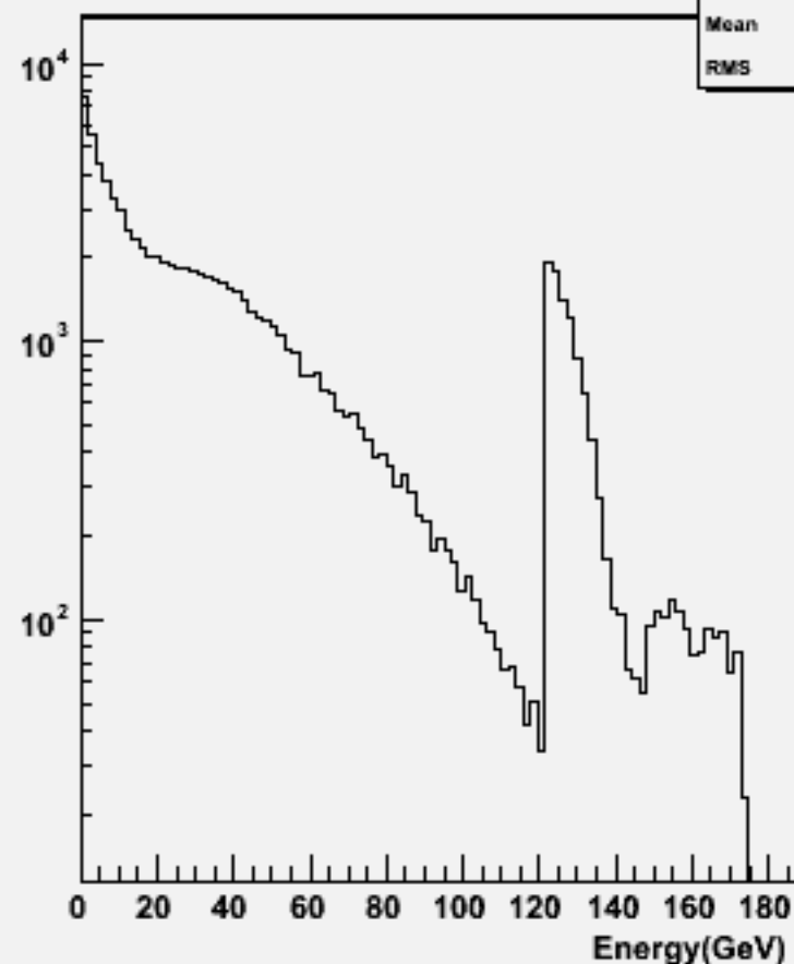
Start point R : w103994 aa_n3e3e2n2_o
