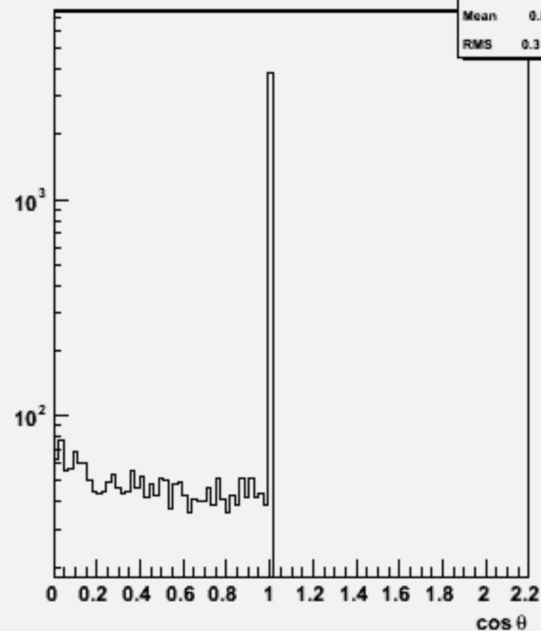
Jet cosθ (All jets)w103994 aa_n3e3e2n2_o
