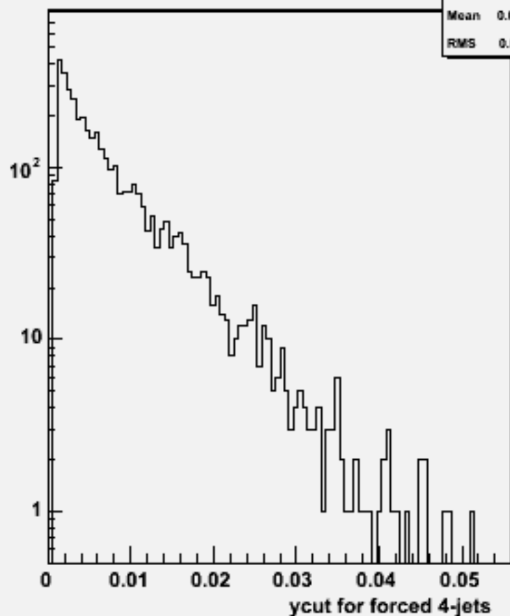
Ycut for 4-jets :w103994 aa_n3e3e2n2_o
