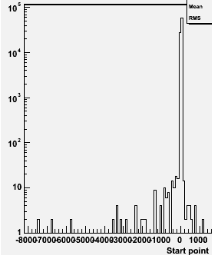
Start point Z : w103994 aa_n3e3e2n2_o
