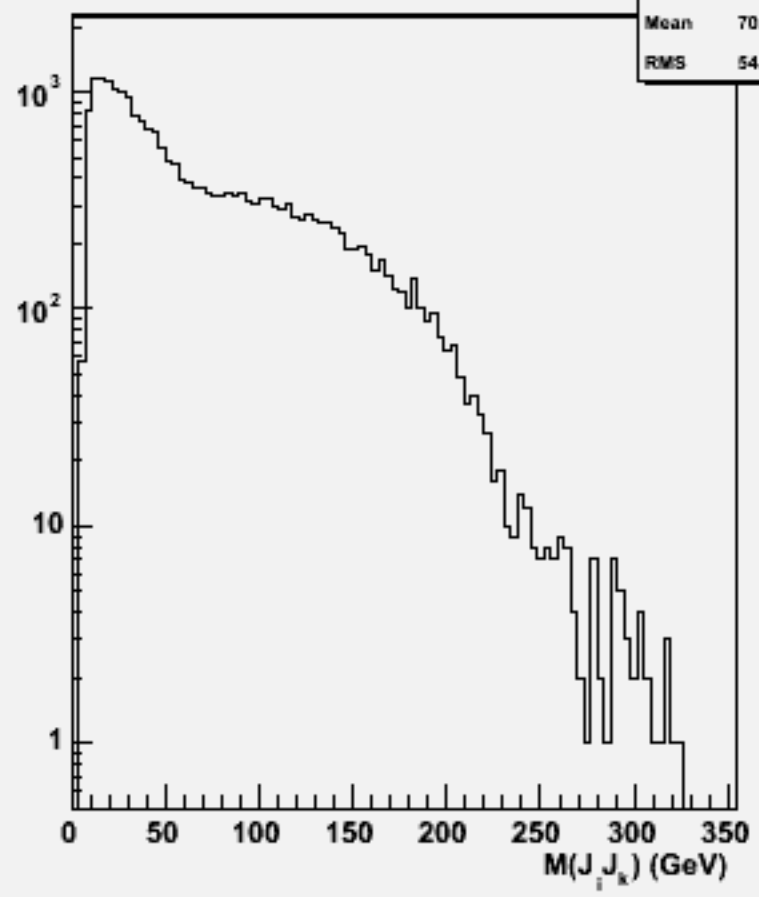
2jets mass(All comb)w103993 aa_n3e3e2n2_o
