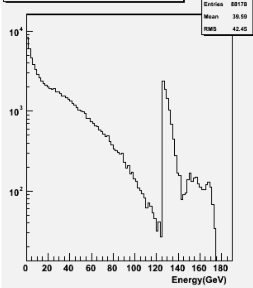
Particle Energy : w103993 aa_n3e3e2n2_o
