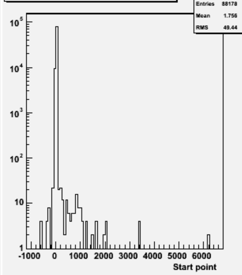
Start point Z : w103993 aa_n3e3e2n2_o
