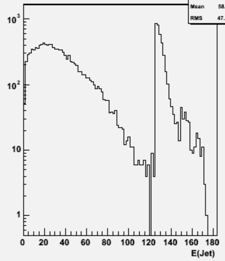
Jet energies(All jets)w103993 aa_n3e3e2n2_o
