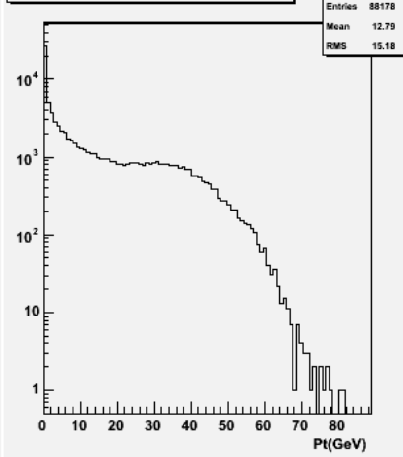
Particle Pt : w103993 aa_n3e3e2n2_o
