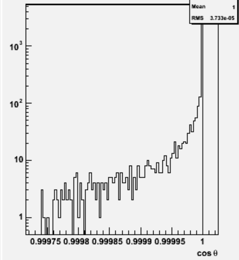
Jet cosθ (All jets)w103993 aa_n3e3e2n2_o
