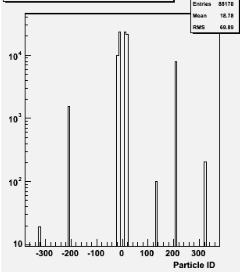
Particle ID : w103993 aa_n3e3e2n2_o
