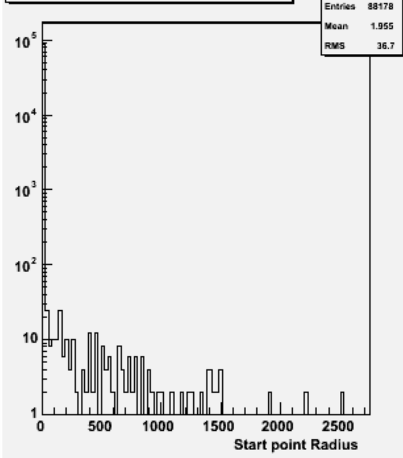
Start point R : w103993 aa_n3e3e2n2_o
