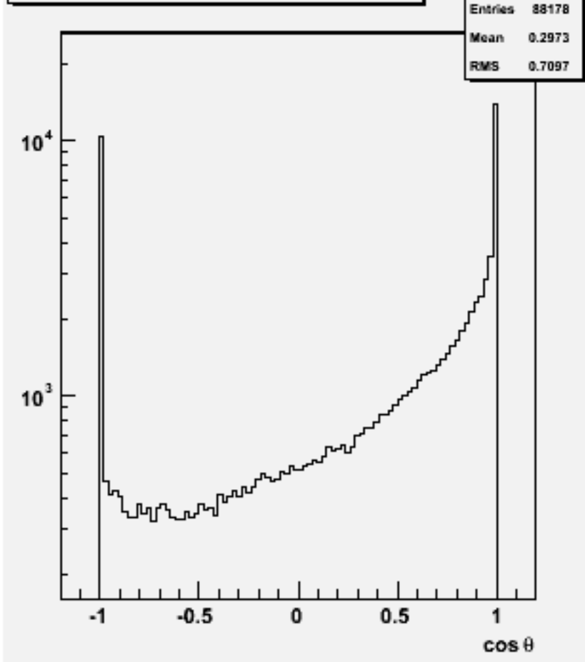
Particle cos \theta : w103993 aa_n3e3e2n2_o
