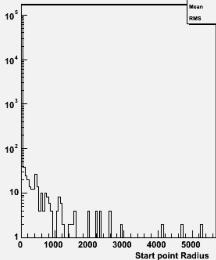
Start point R : w103990 aa_n3e3e1n1_o
