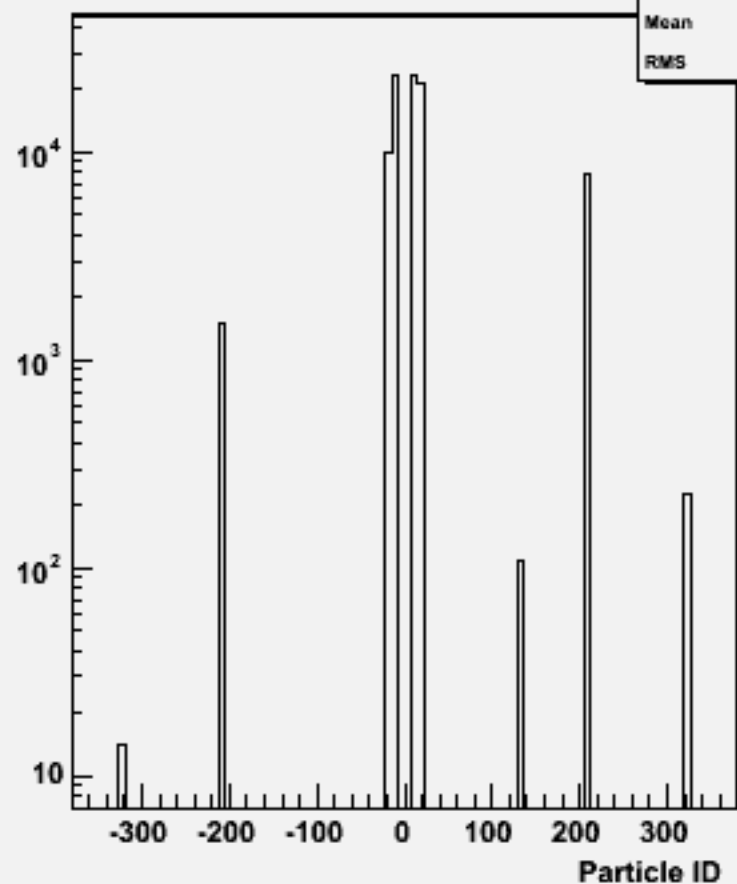
Particle ID : w103990 aa_n3e3e1n1_o
