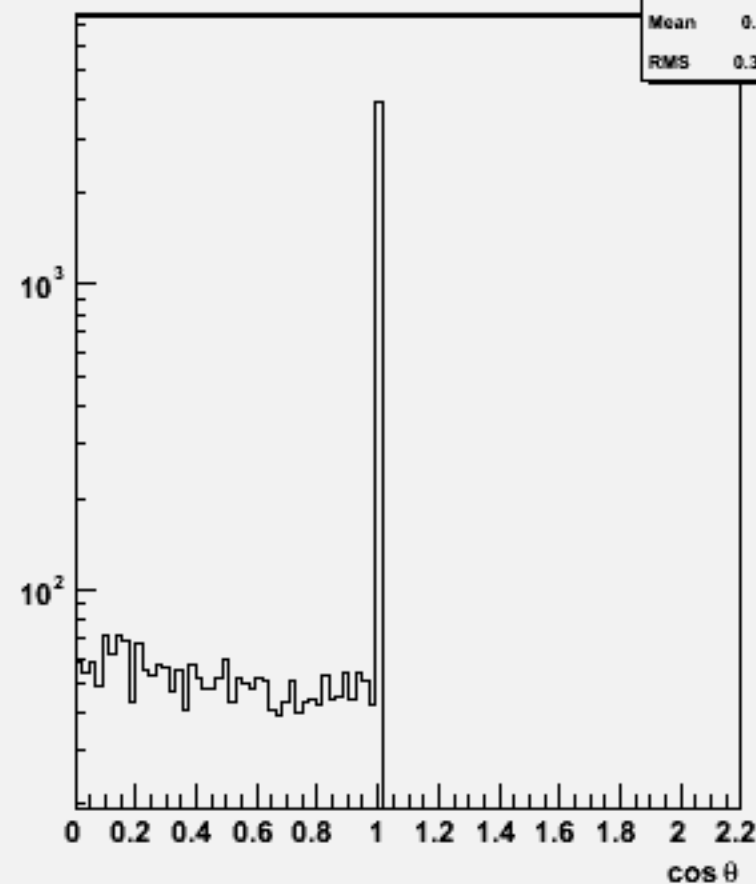
Jet cos \theta (All jets)w103990 aa_n3e3e1n1_o
