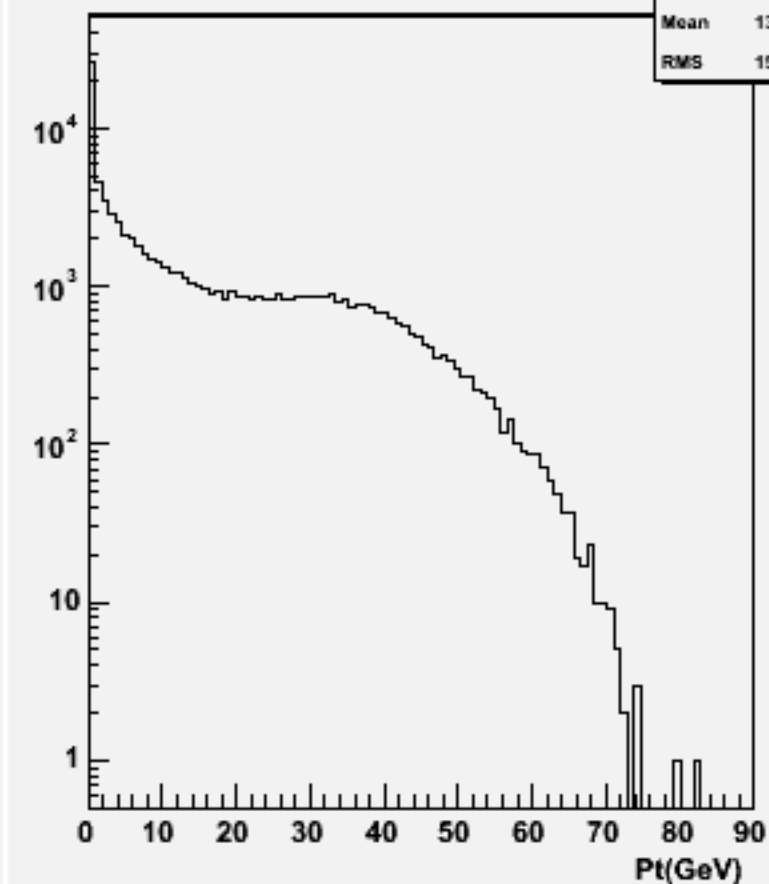
Particle Pt : w103990 aa_n3e3e1n1_o
