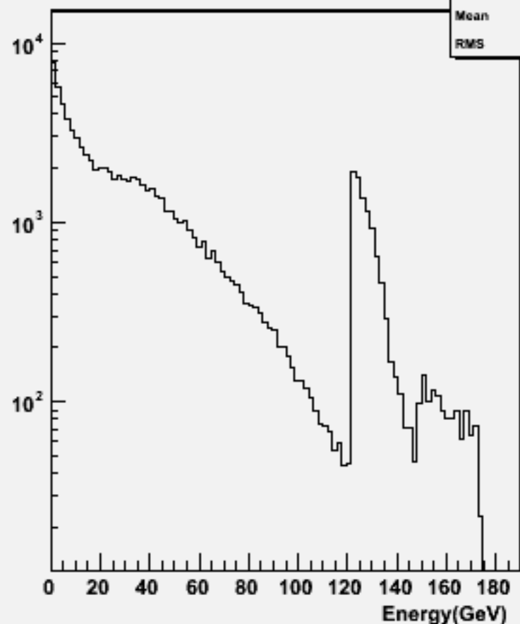
Particle Energy : w103990 aa_n3e3e1n1_o
