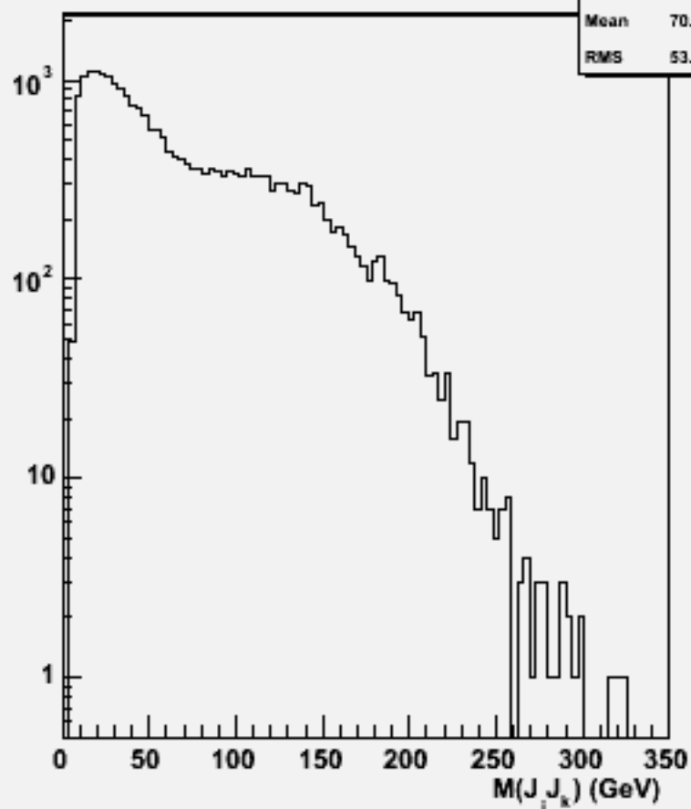
2jets mass(All comb)w103990 aa_n3e3e1n1_o
