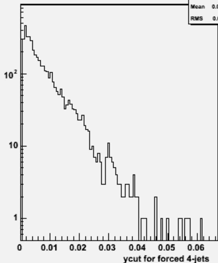
Ycut for 4-jets :w103990 aa_n3e3e1n1_o
