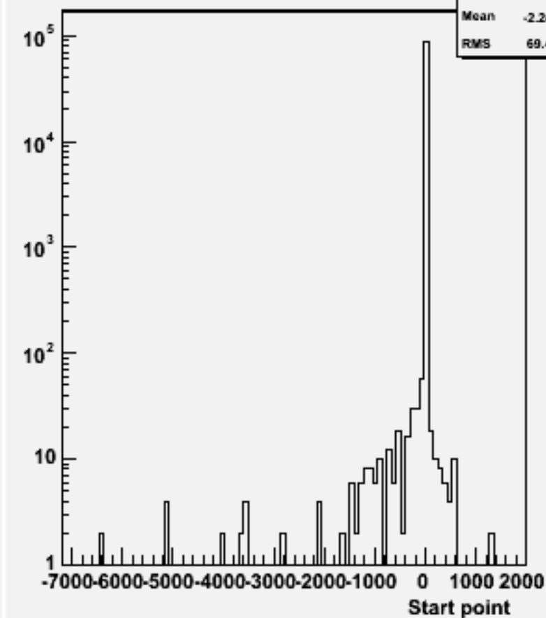
Start point Z : w103990 aa_n3e3e1n1_o
