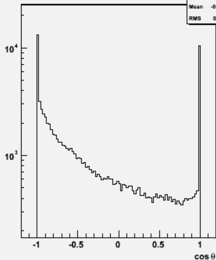
Particle cos \theta : w103990 aa_n3e3e1n1_o
