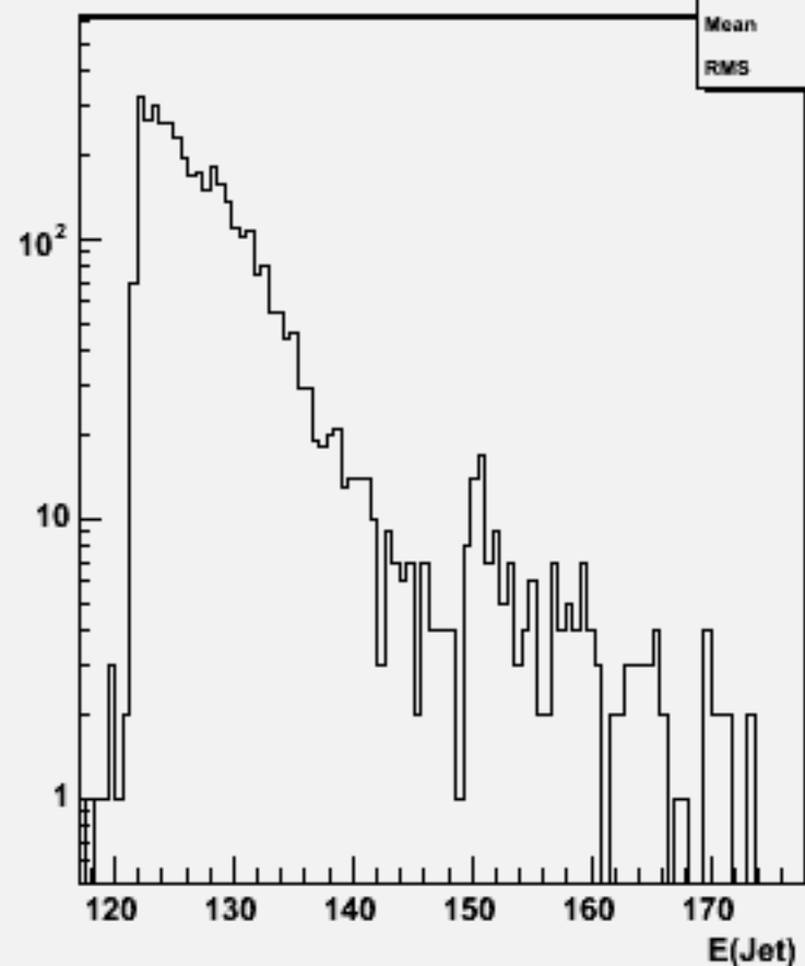
Jet energies(All jets)w103990 aa_n3e3e1n1_o
