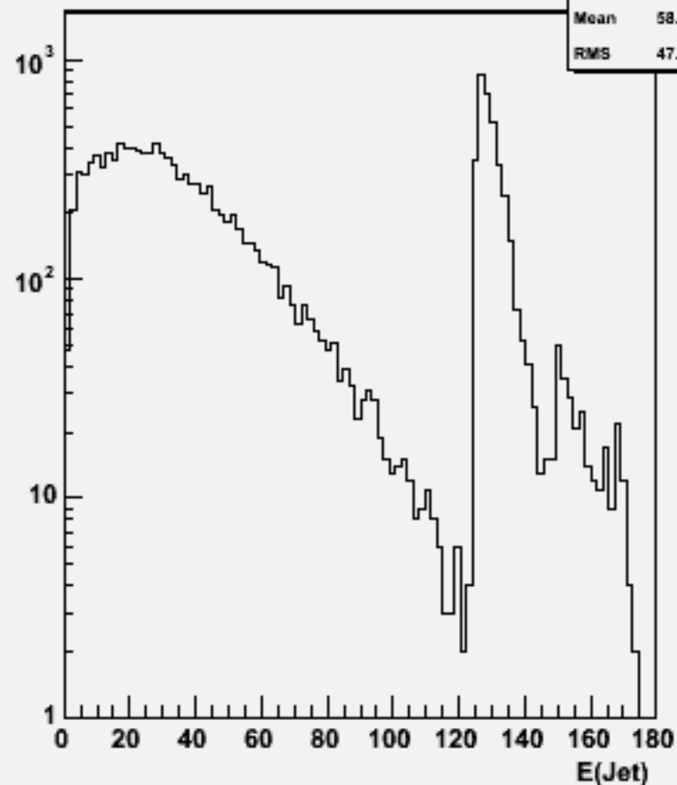
Jet energies(All jets)w103989 aa_n3e3e1n1_o
