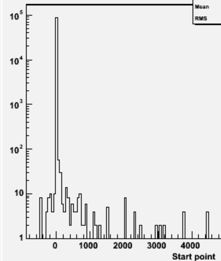
Start point Z : w103989 aa_n3e3e1n1_o
