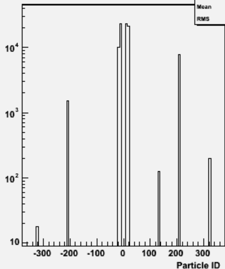
Particle ID : w103989 aa_n3e3e1n1_o
