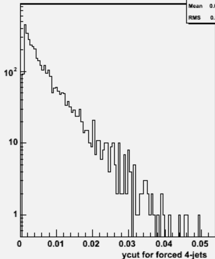
Ycut for 4-jets :w103989 aa_n3e3e1n1_o
