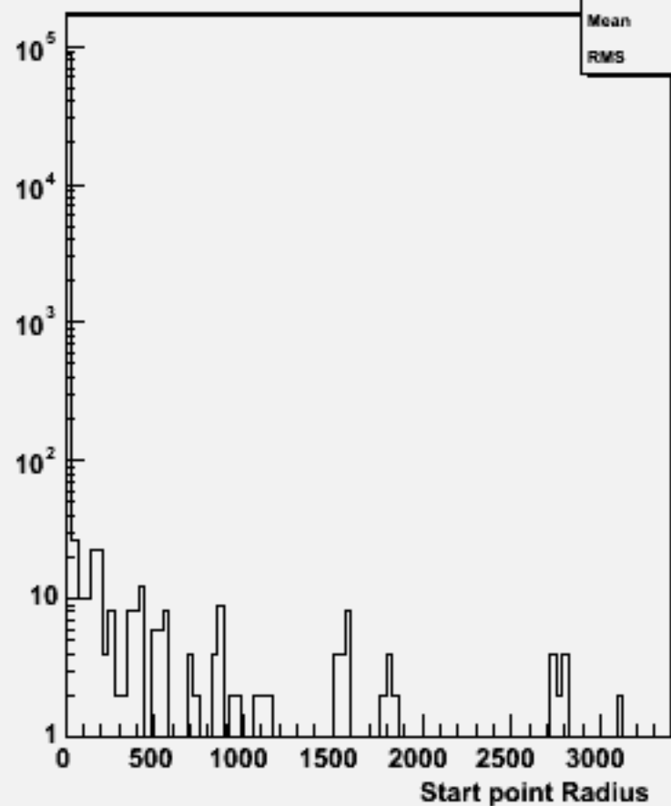
Start point R : w103989 aa_n3e3e1n1_o
