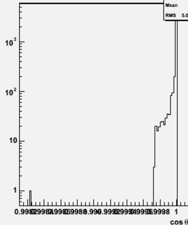
Jet cosθ (All jets)w103989 aa_n3e3e1n1_o
