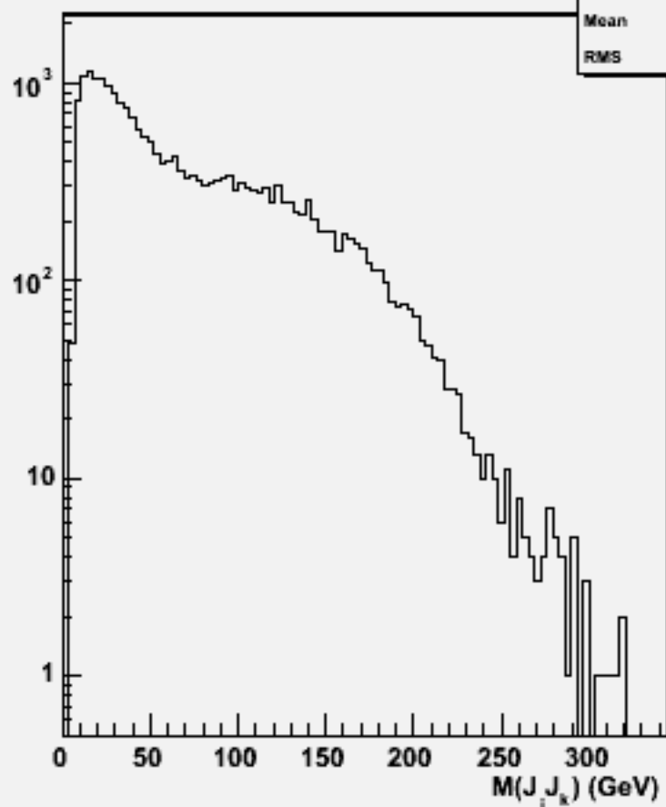
2jets mass(All comb)w103989 aa_n3e3e1n1_o
