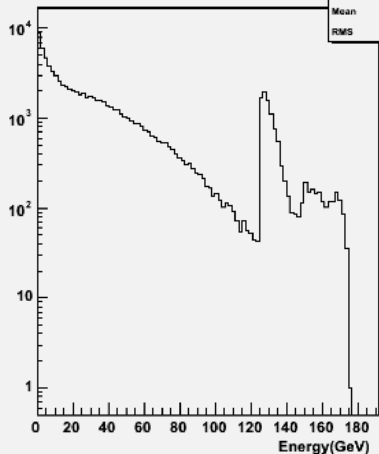
Particle Energy : w103989 aa_n3e3e1n1_o
