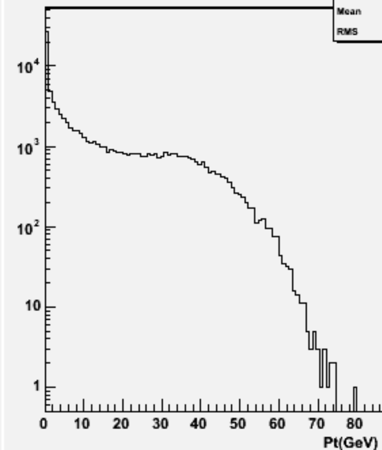
Particle Pt : w103989 aa_n3e3e1n1_o
