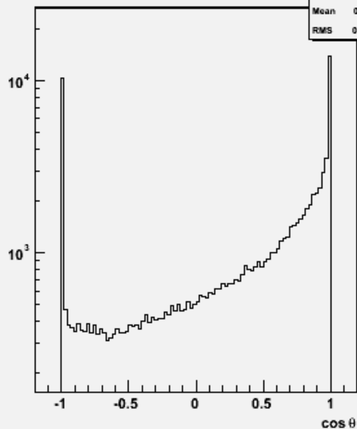
Particle cos \theta : w103989 aa_n3e3e1n1_o
