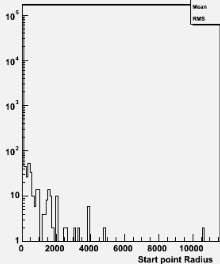
Start point R : w103988 aa_n3e3e1n1_o
