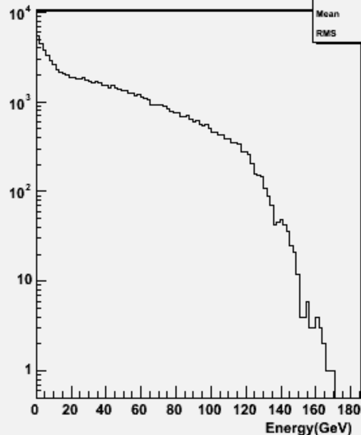
Particle Energy : w103988 aa_n3e3e1n1_o
