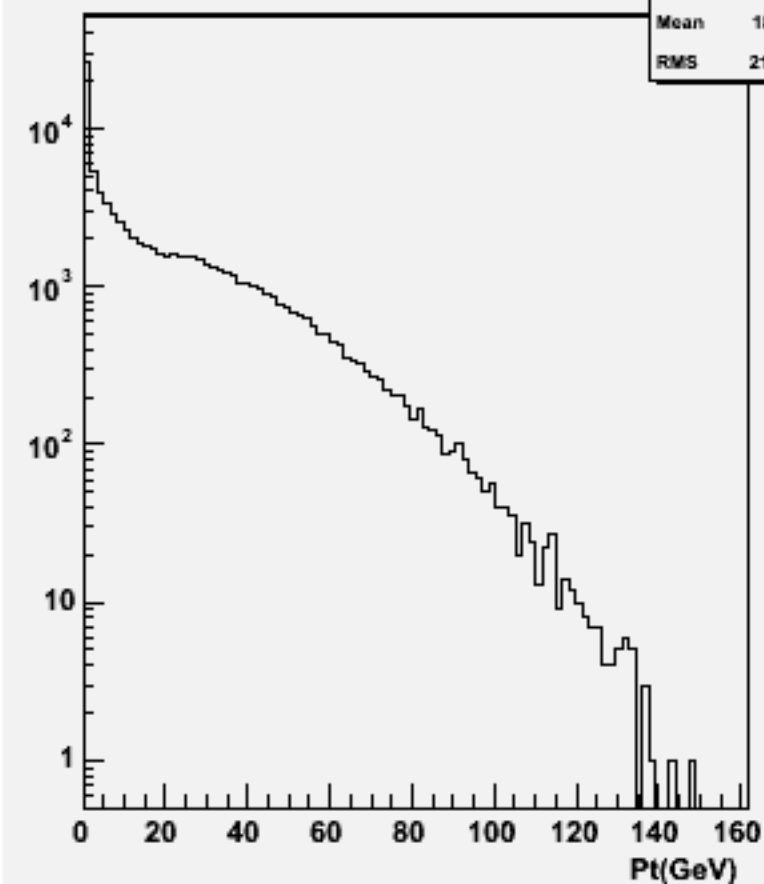
Particle Pt : w103988 aa_n3e3e1n1_o
