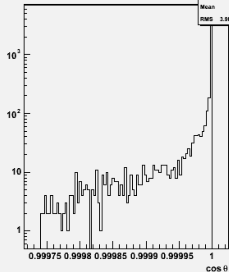
Jet cosθ (All jets)w103988 aa_n3e3e1n1_o
