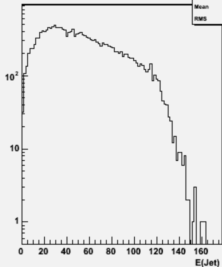
Jet energies(All jets)w103988 aa_n3e3e1n1_o
