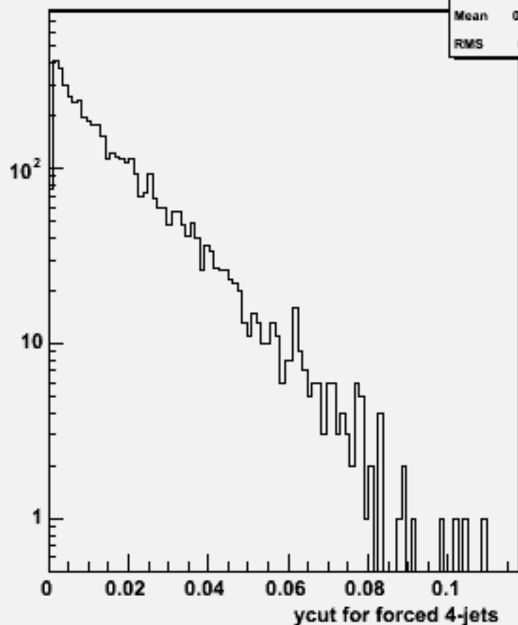
Ycut for 4-jets :w103988 aa_n3e3e1n1_o
