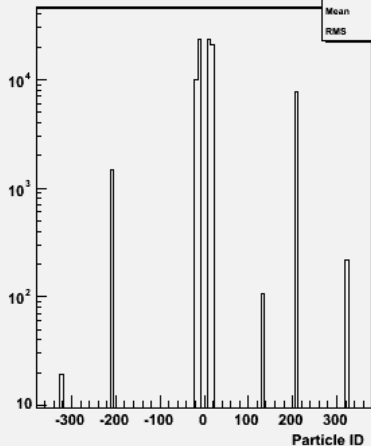
Particle ID : w103988 aa_n3e3e1n1_o
