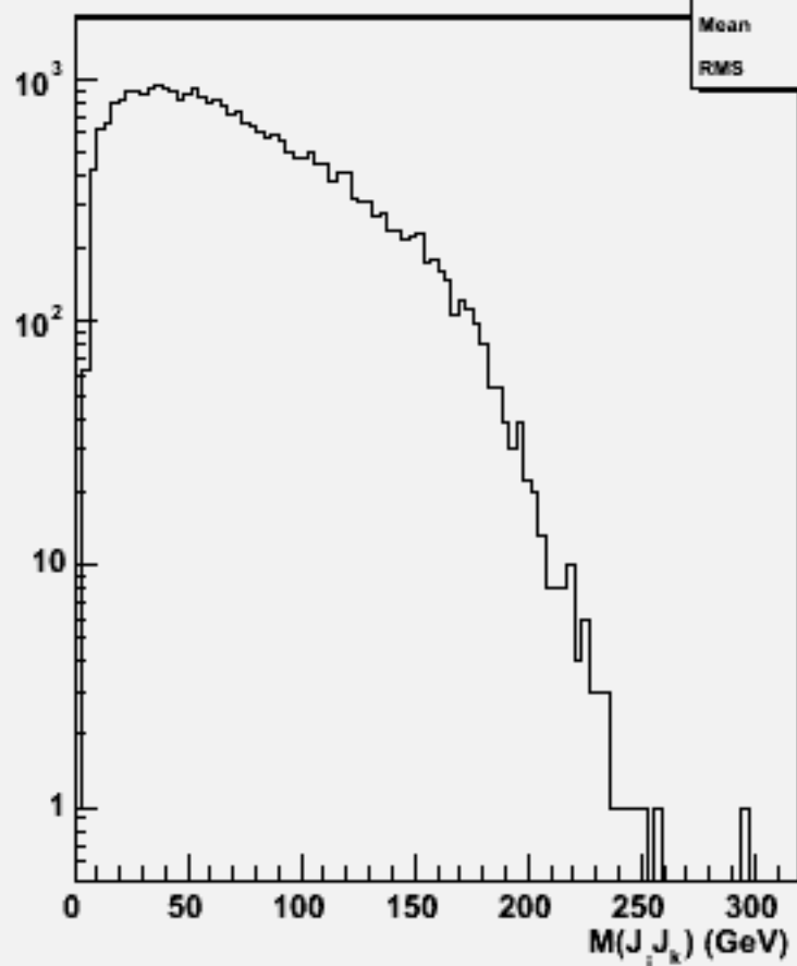
2jets mass(All comb)w103988 aa_n3e3e1n1_o
