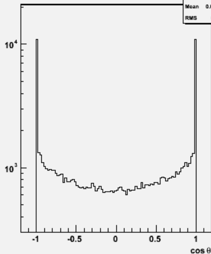
Particle cos \theta : w103988 aa_n3e3e1n1_o
