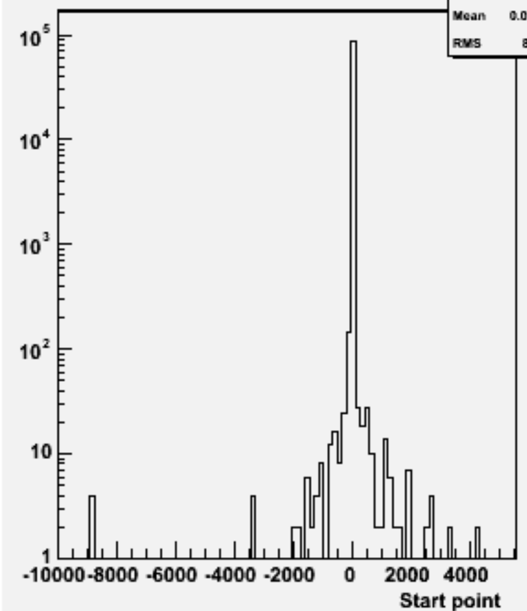
Start point Z : w103988 aa_n3e3e1n1_o
