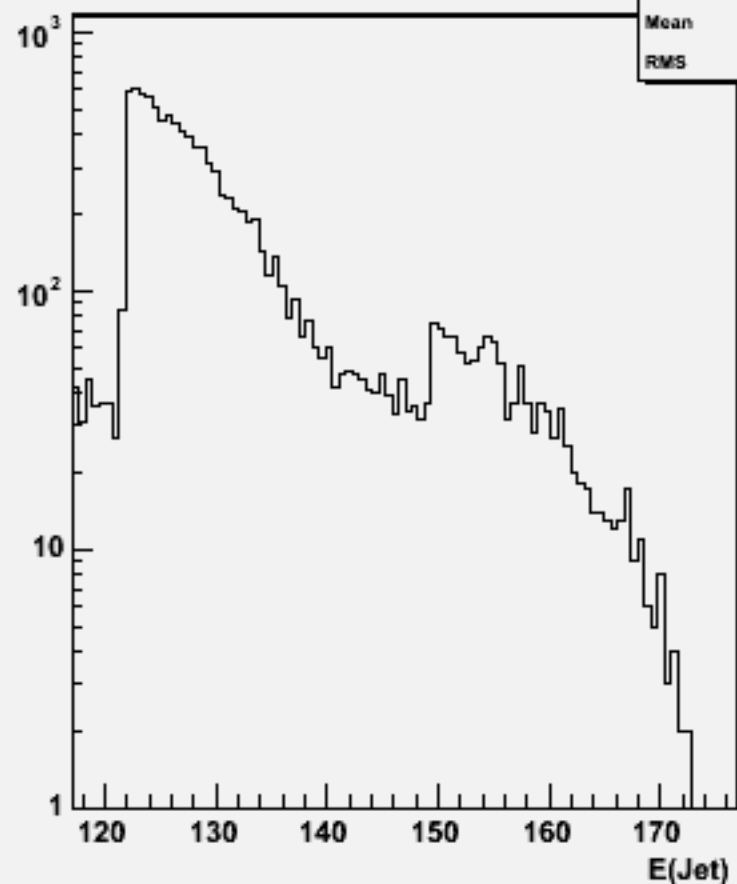
Jet energies(All jets)w103986 aa_n2e2sc_o
