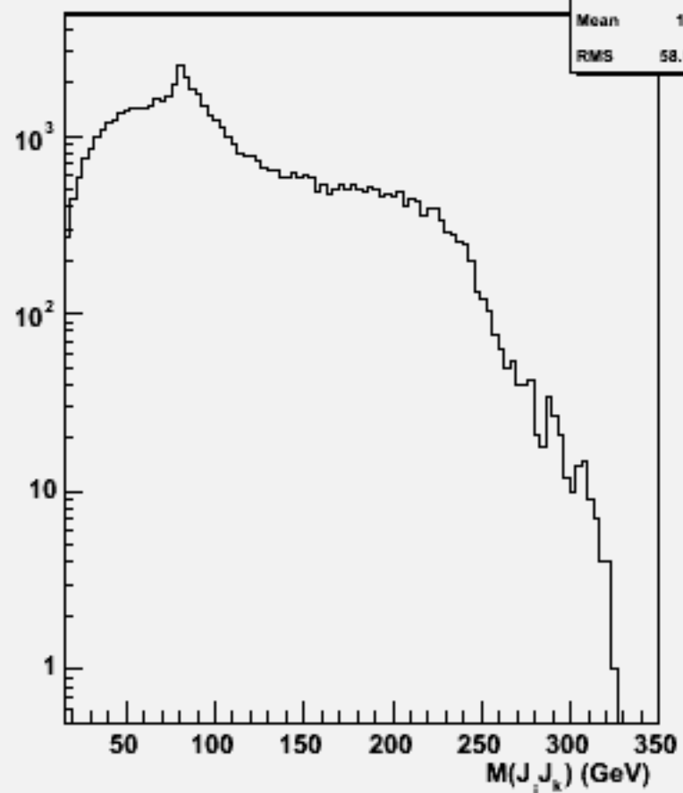
2jets mass(All comb)w103986 aa_n2e2sc_o
