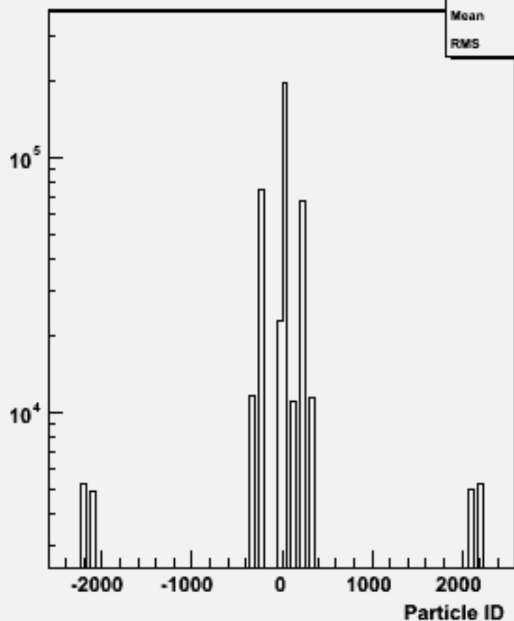
Particle ID : w103986 aa_n2e2sc_o
