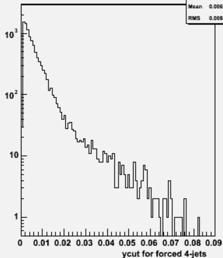
Ycut for 4-jets :w103986 aa_n2e2sc_o
