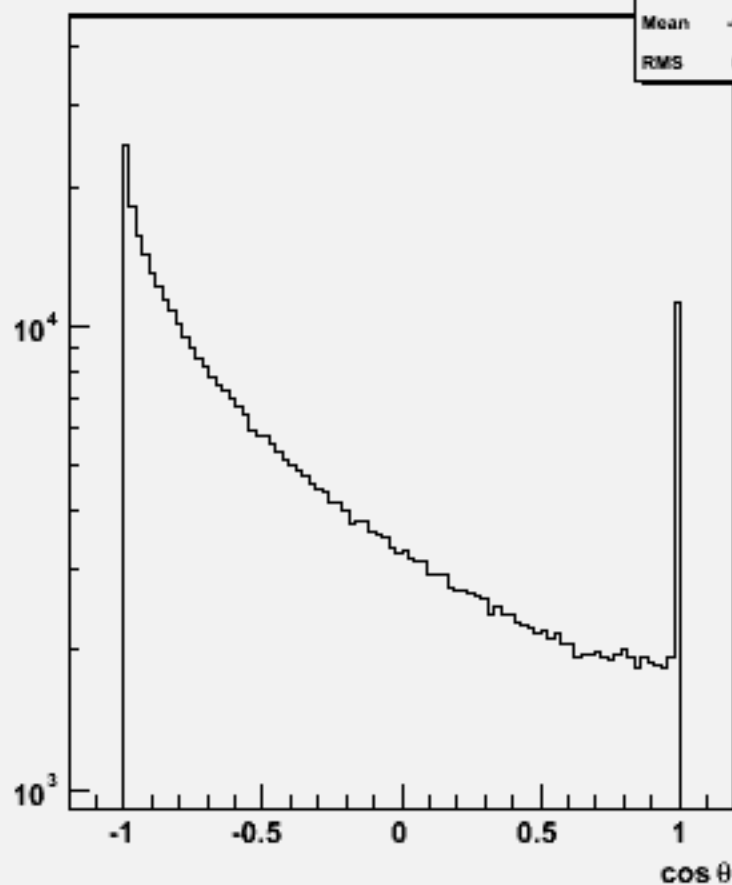
Particle cos \theta : w103986 aa_n2e2sc_o
