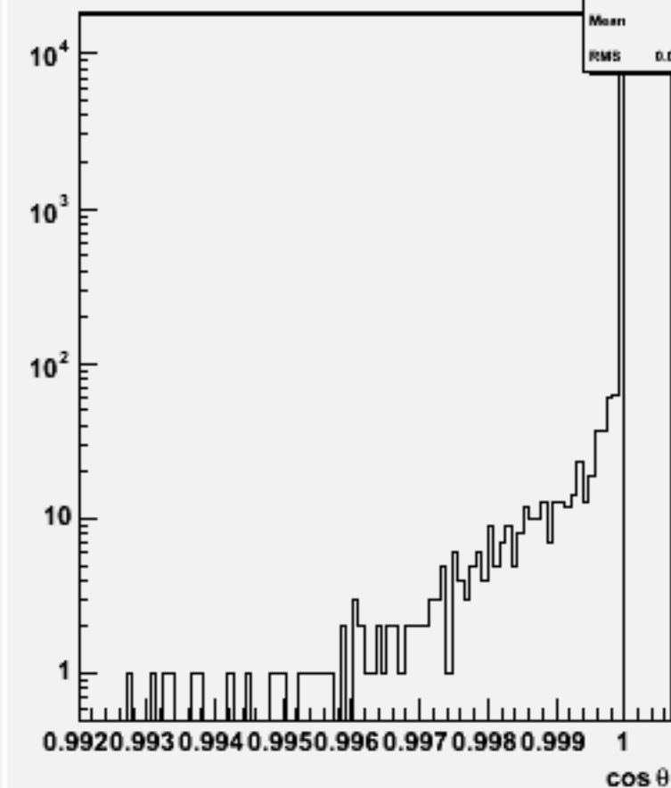
Jet cos \theta (All jets)w103986 aa_n2e2sc_o
