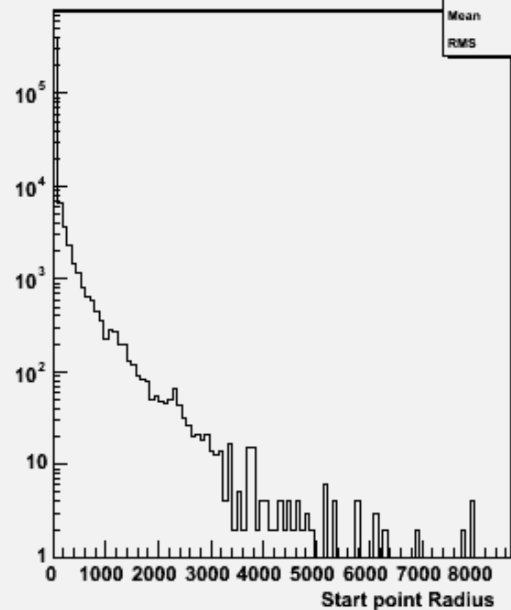
Start point R : w103986 aa_n2e2sc_o
