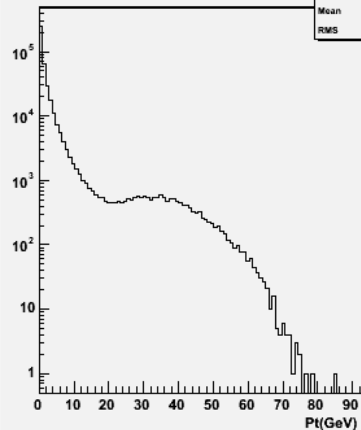
Particle Pt : w103986 aa_n2e2sc_o
