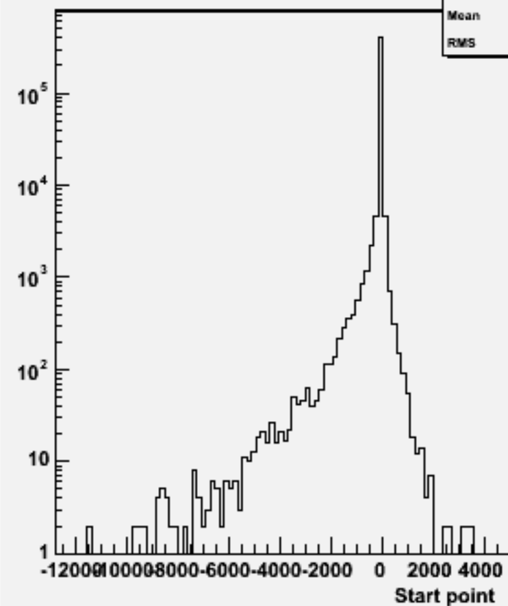
Start point Z : w103986 aa_n2e2sc_o
