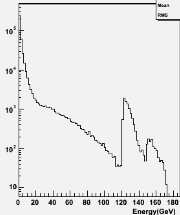
Particle Energy : w103986 aa_n2e2sc_o
