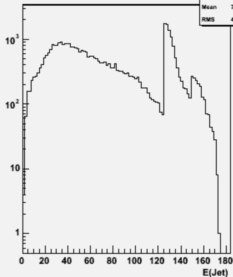
Jet energies(All jets)w103985 aa_n2e2sc_o
