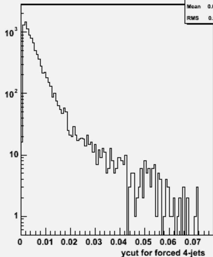
Ycut for 4-jets :w103985 aa_n2e2sc_o
