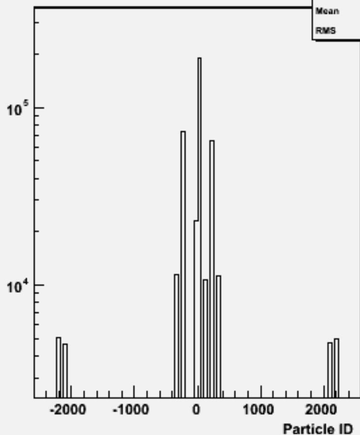
Particle ID : w103985 aa_n2e2sc_o
