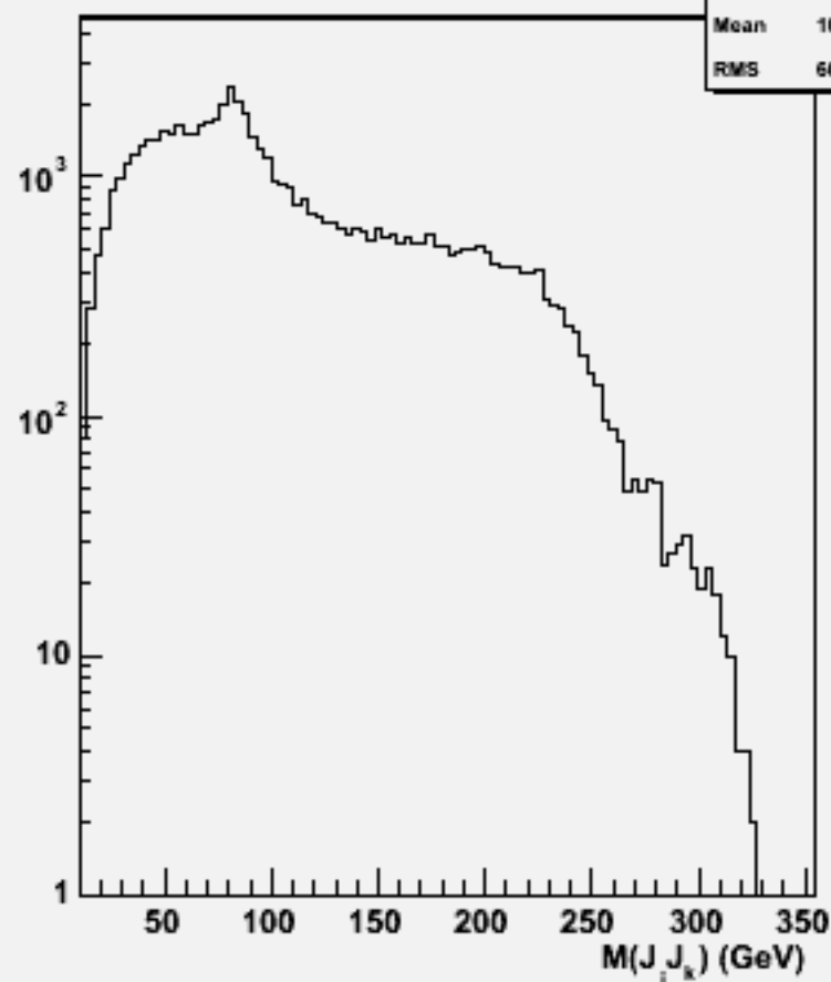
2jets mass(All comb)w103985 aa_n2e2sc_o
