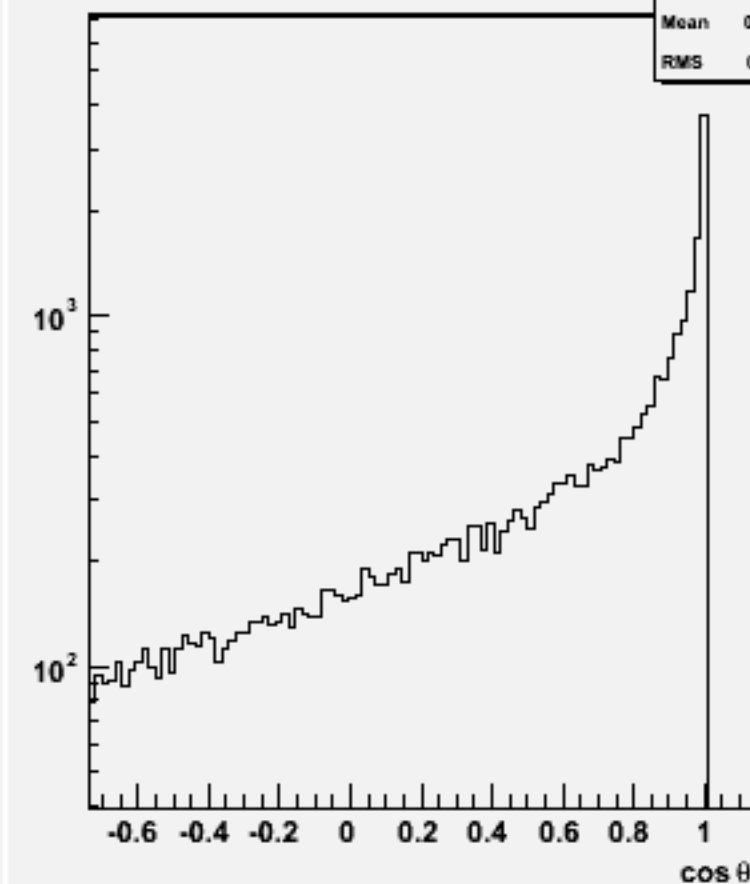
Jet cos \theta (All jets)w103985 aa_n2e2sc_o
