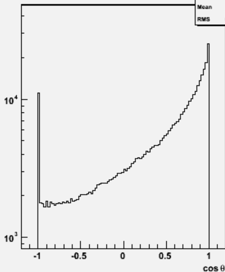
Particle cos \theta : w103985 aa_n2e2sc_o
