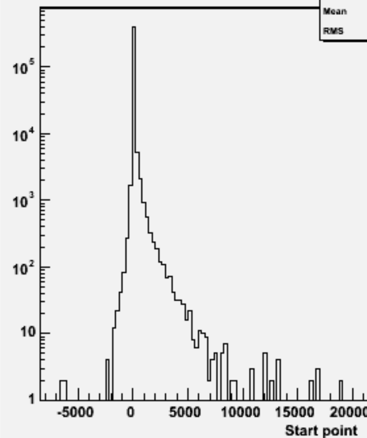
Start point Z : w103985 aa_n2e2sc_o
