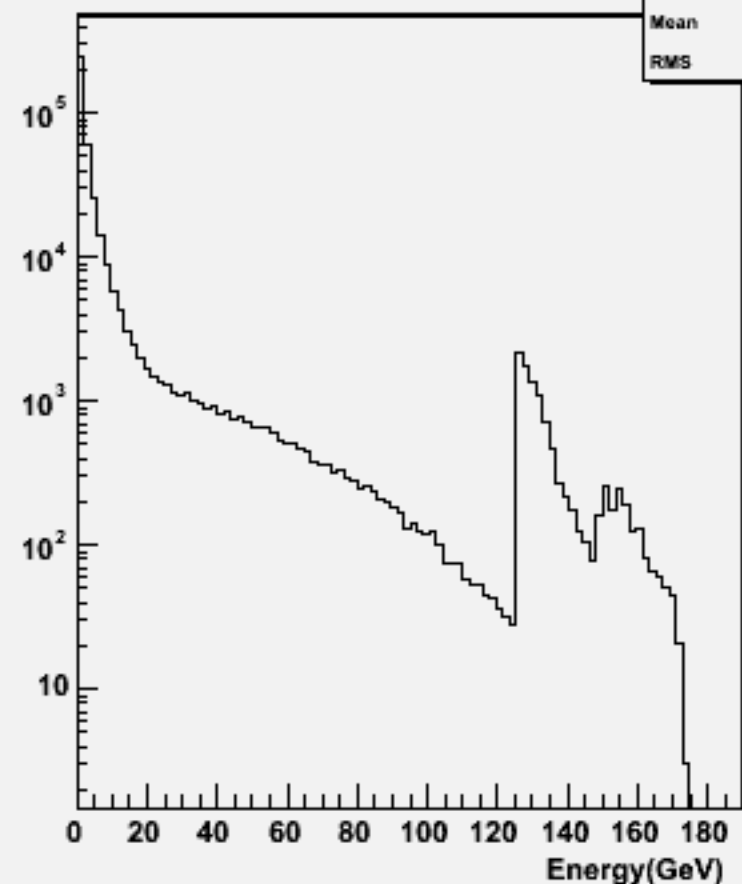
Particle Energy : w103985 aa_n2e2sc_o
