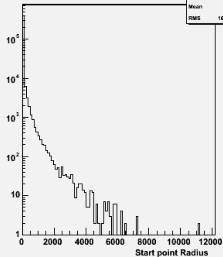
Start point R : w103985 aa_n2e2sc_o
