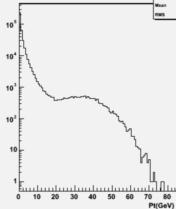
Particle Pt : w103985 aa_n2e2sc_o
