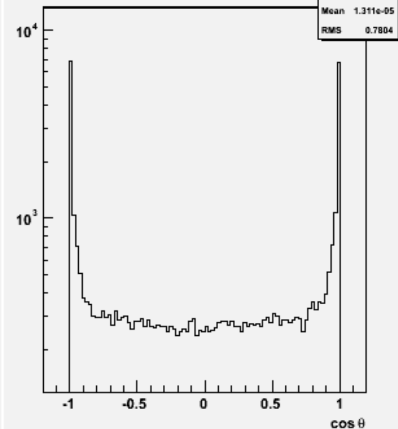
Jet cos \theta (All jets)w103984 aa_n2e2sc_o
