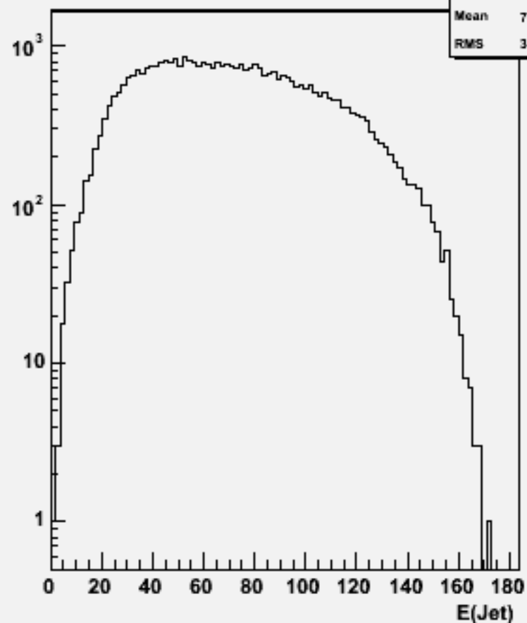
Jet energies(All jets)w103984 aa_n2e2sc_o
