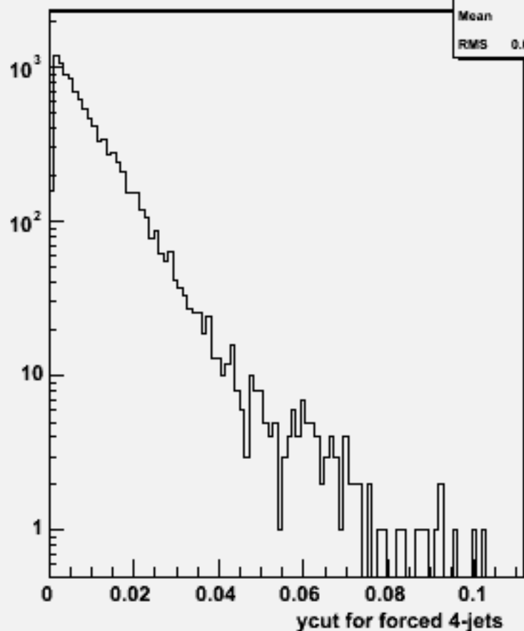
Ycut for 4-jets :w103984 aa_n2e2sc_o
