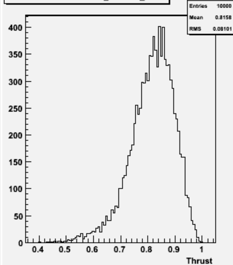
Thrust w103984 aa_n2e2sc_o
