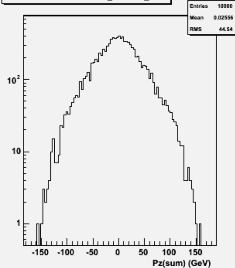
Pz Sum: w103984 aa_n2e2sc_o
