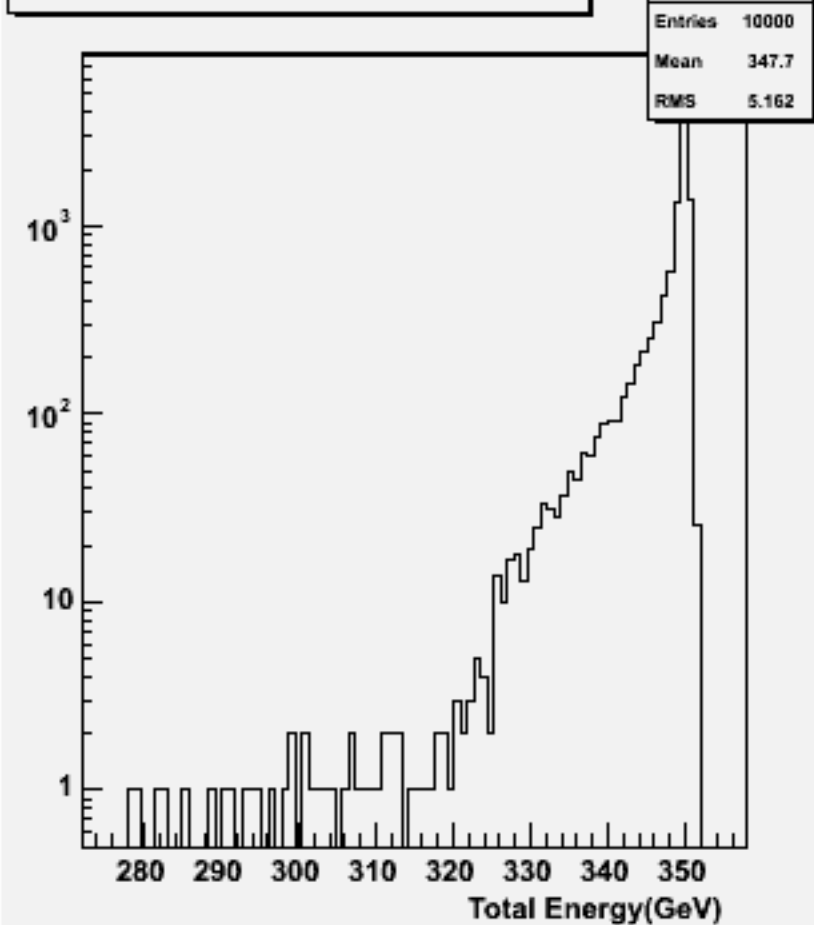
Total Energy (inc. \nu ): w103984 aa_n2e2sc_o
