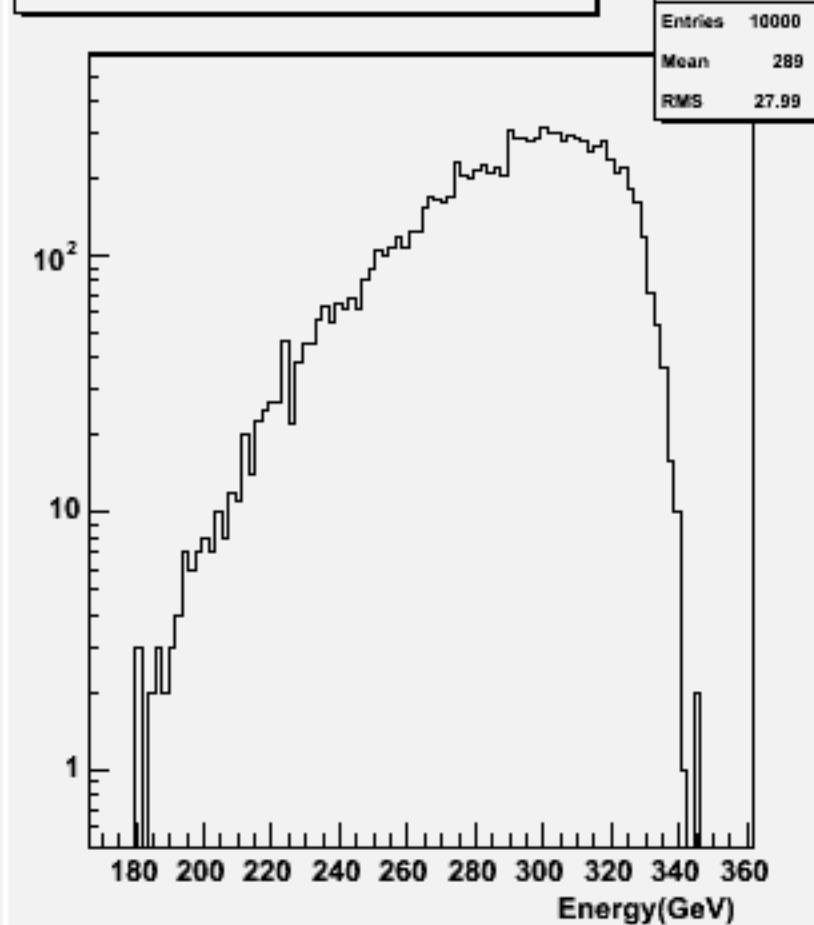
Total Energy (w/o \nu ): w103984 aa_n2e2sc_o
