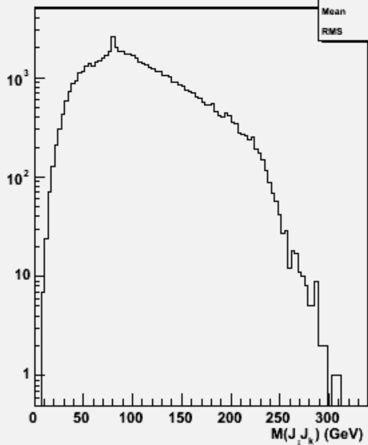
2jets mass(All comb)w103984 aa_n2e2sc_o
