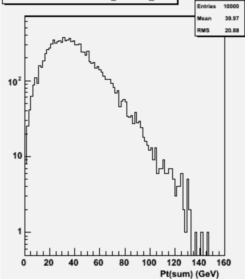
Pt Sum: w103984 aa_n2e2sc_o
