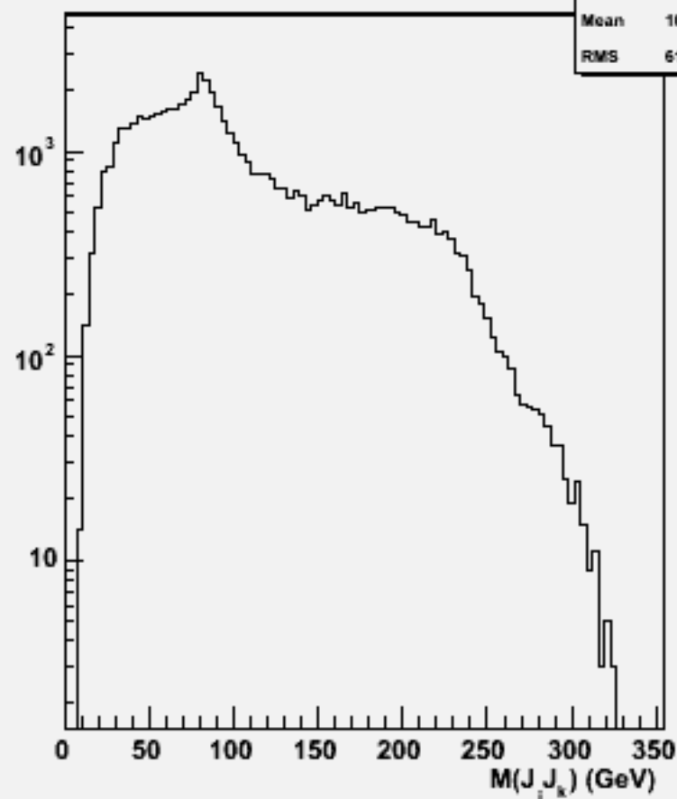
2jets mass(All comb)w103981 aa_n2e2du_o
