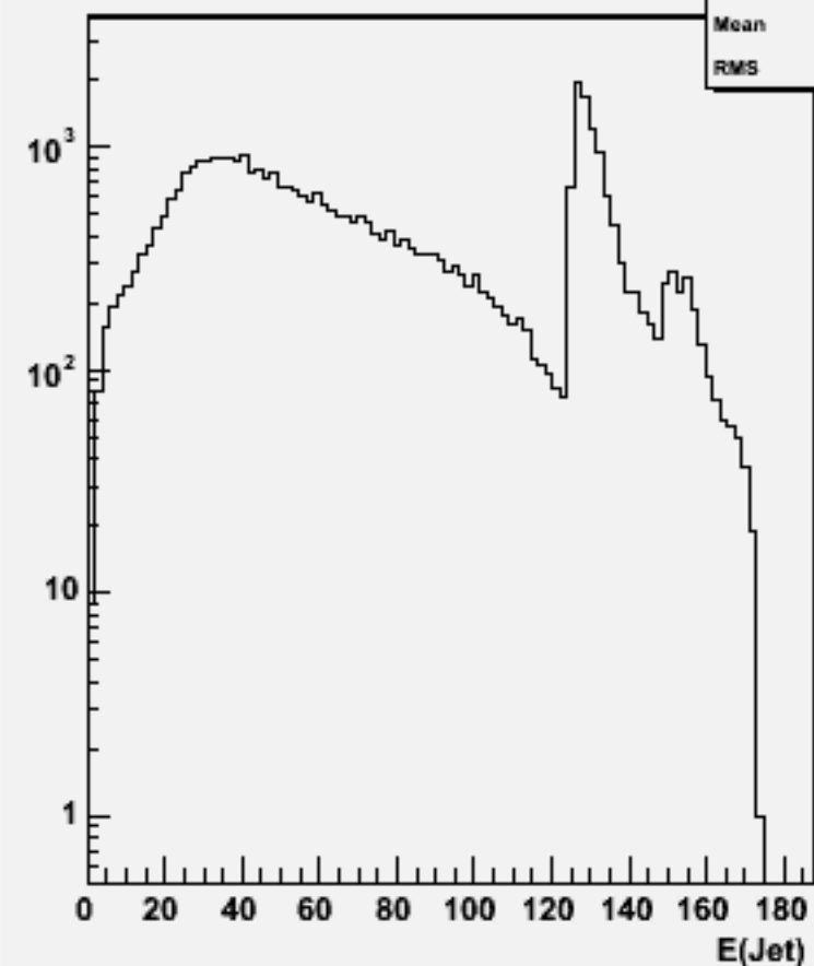
Jet energies(All jets)w103981 aa_n2e2du_o
