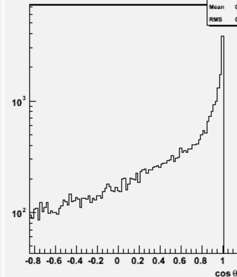
Jet cos \theta (All jets)w103981 aa_n2e2du_o
