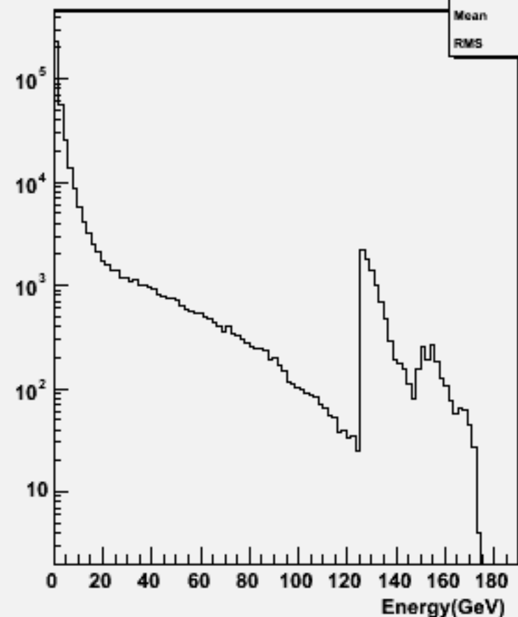
Particle Energy : w103981 aa_n2e2du_o
