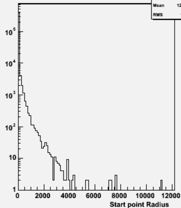
Start point R : w103981 aa_n2e2du_o
