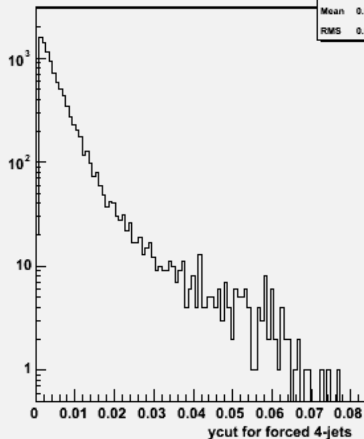
Ycut for 4-jets :w103981 aa_n2e2du_o
