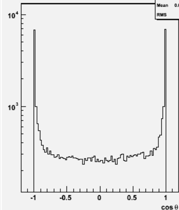
Jet cos \theta (All jets)w103980 aa_n2e2du_o
