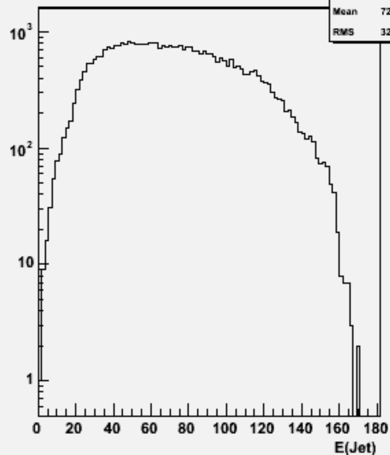
Jet energies(All jets)w103980 aa_n2e2du_o
