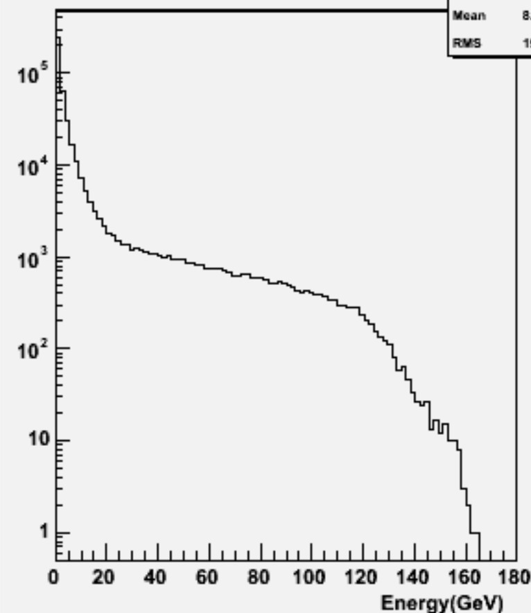
Particle Energy : w103980 aa_n2e2du_o
