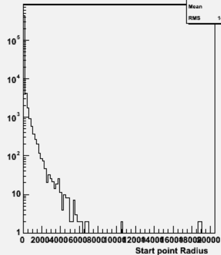
Start point R : w103980 aa_n2e2du_o
