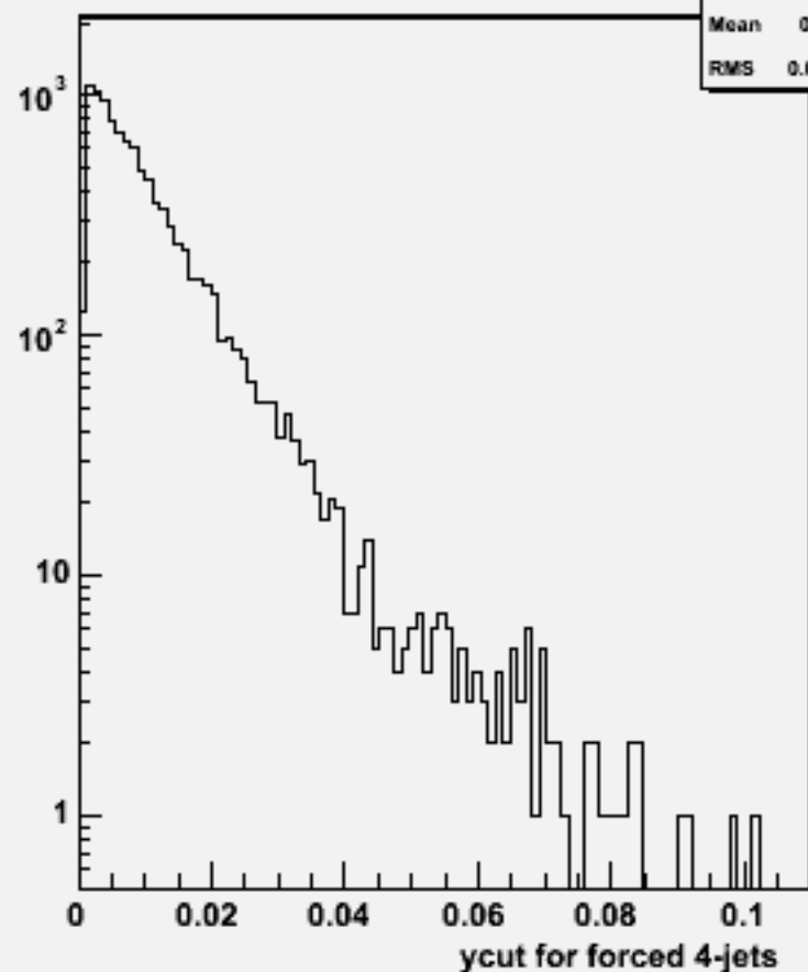
Ycut for 4-jets :w103980 aa_n2e2du_o
