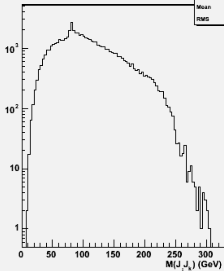
2jets mass(All comb)w103980 aa_n2e2du_o
