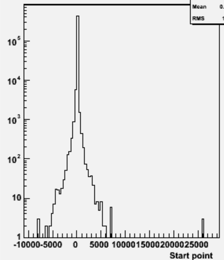
Start point Z : w103980 aa_n2e2du_o
