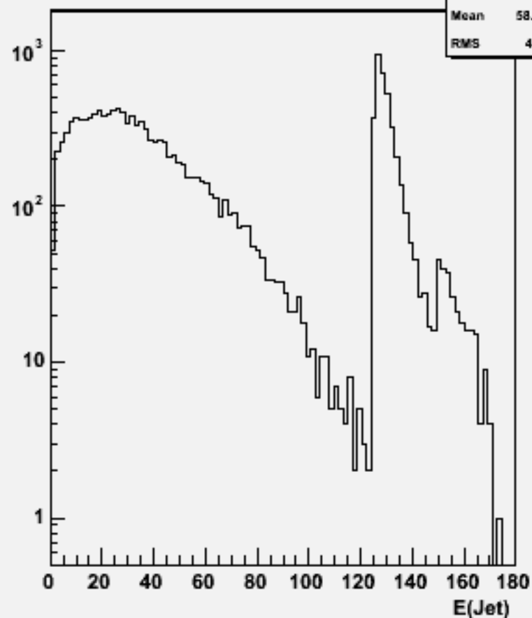
Jet energies(All jets)w103977 aa_n2e2e3n3_o
