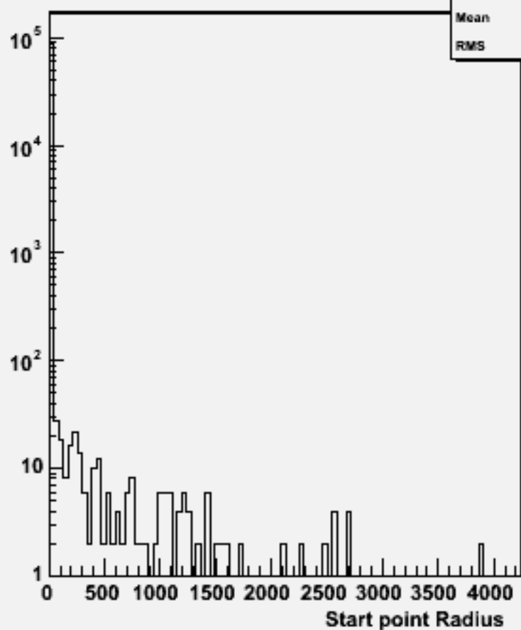
Start point R : w103977 aa_n2e2e3n3_o
