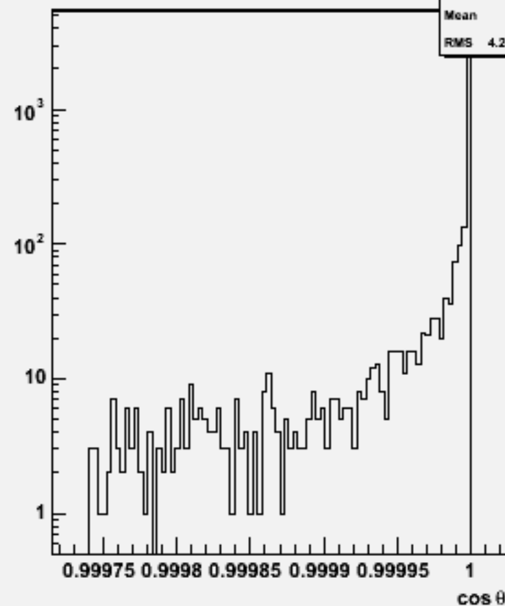
Jet cos \theta (All jets)w103977 aa_n2e2e3n3_o
