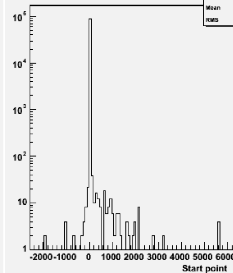
Start point Z : w103977 aa_n2e2e3n3_o
