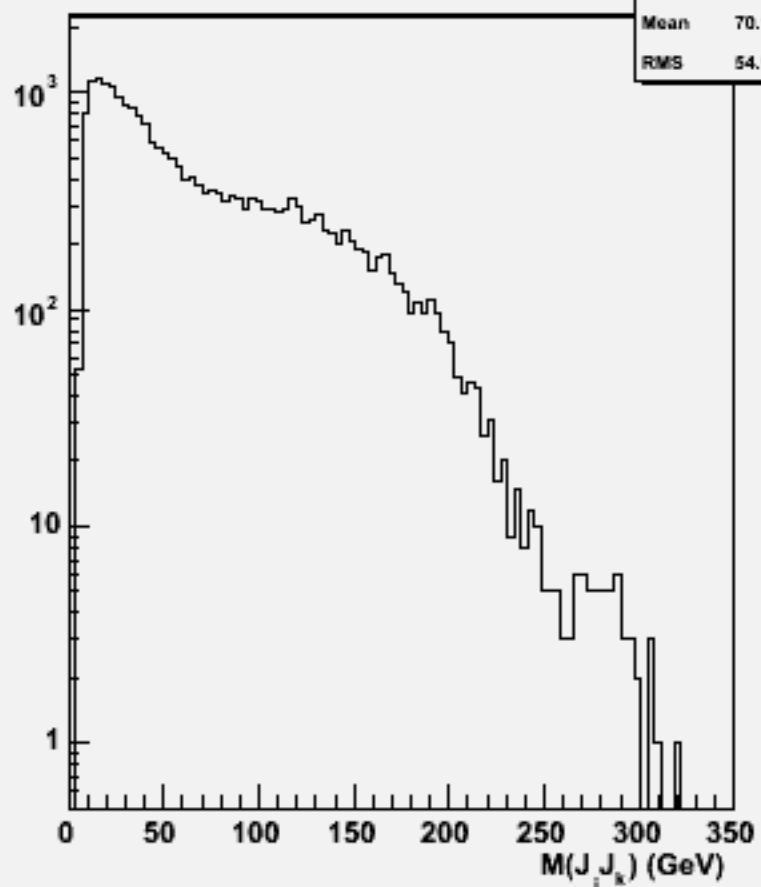
2jets mass(All comb)w103977 aa_n2e2e3n3_o
