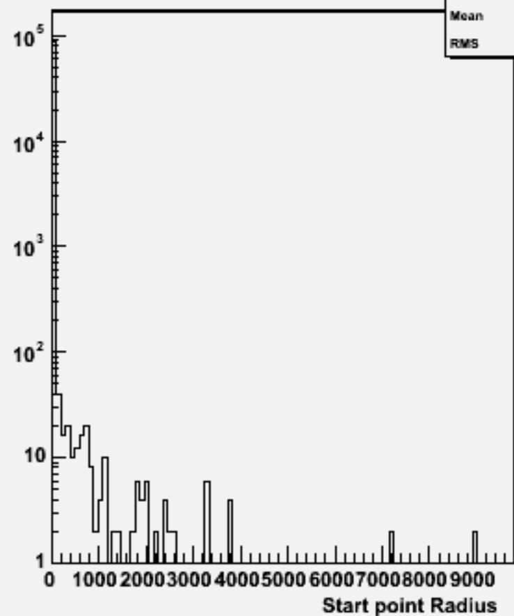
Start point R : w103976 aa_n2e2e3n3_o
