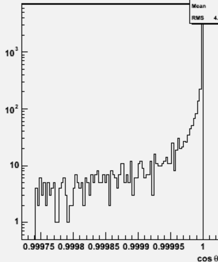
Jet cos \theta (All jets)w103976 aa_n2e2e3n3_o
