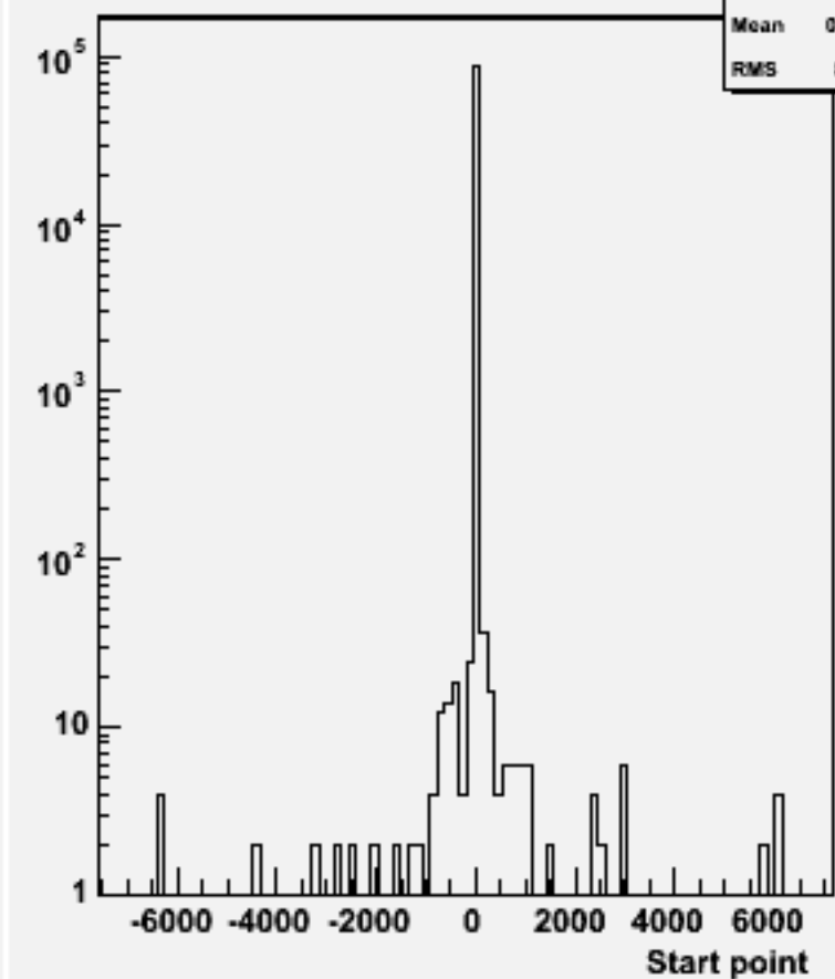
Start point Z : w103976 aa_n2e2e3n3_o
