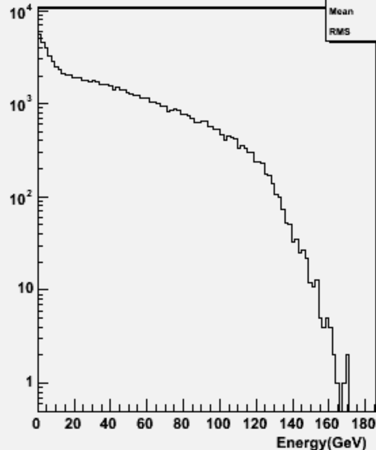
Particle Energy : w103976 aa_n2e2e3n3_o
