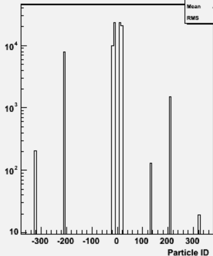
Particle ID : w103976 aa_n2e2e3n3_o
