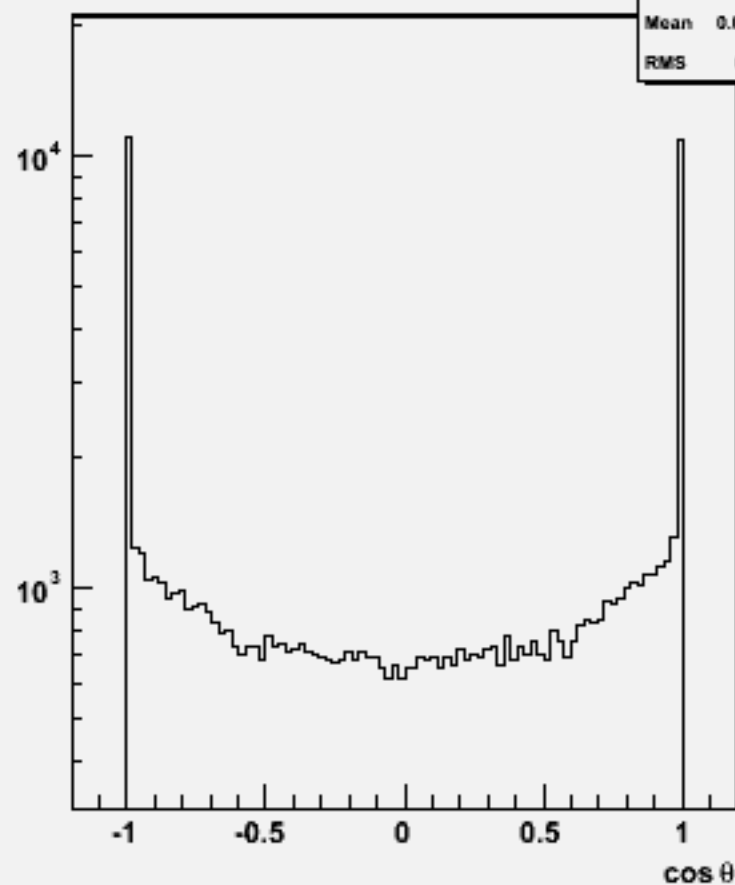
Particle cos \theta : w103976 aa_n2e2e3n3_o
