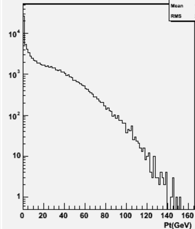
Particle Pt : w103976 aa_n2e2e3n3_o
