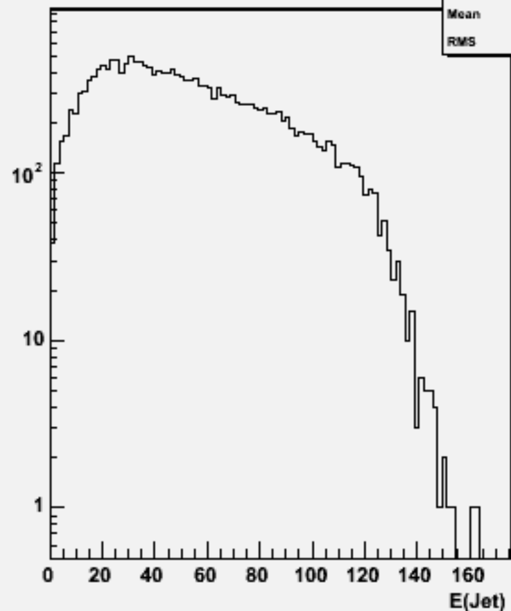
Jet energies(All jets)w103976 aa_n2e2e3n3_o
