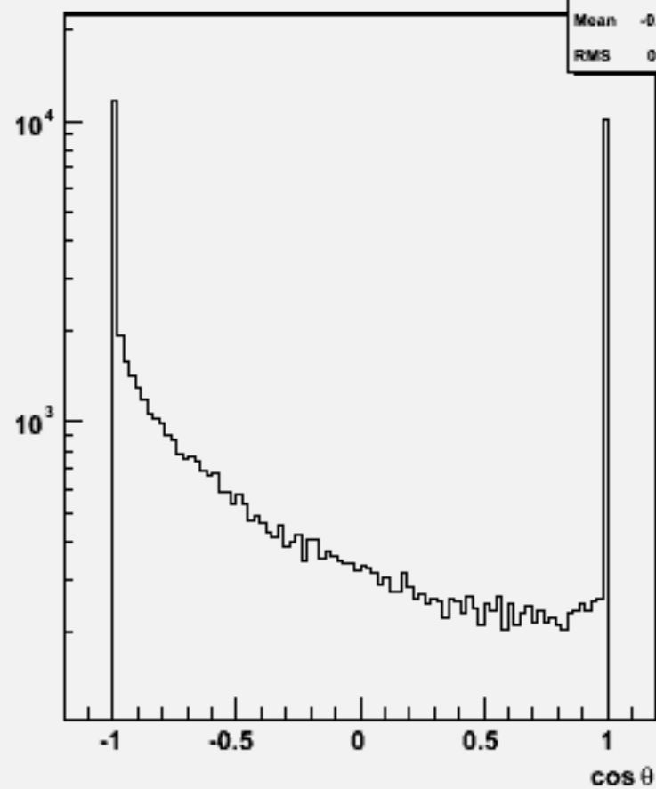
Particle cos \theta : w103974 aa_n2e2e2n2_o
