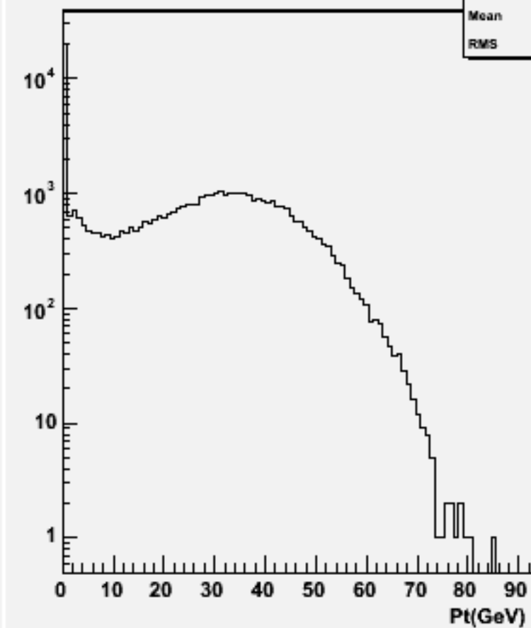
Particle Pt : w103974 aa_n2e2e2n2_o
