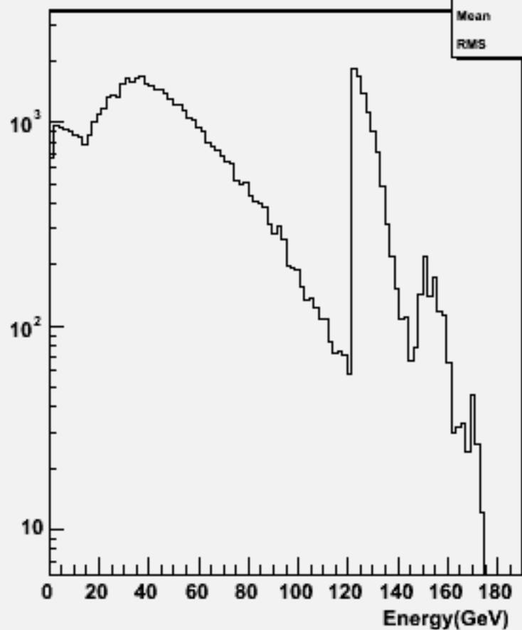
Particle Energy : w103974 aa_n2e2e2n2_o
