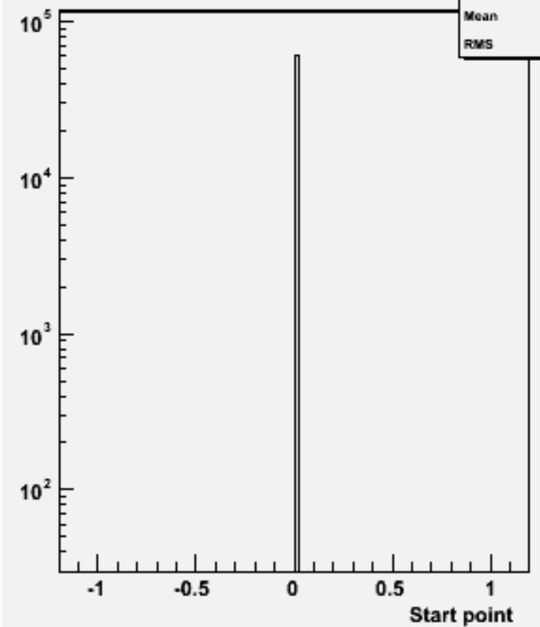
Start point Z : w103972 aa_n2e2e2n2_o
