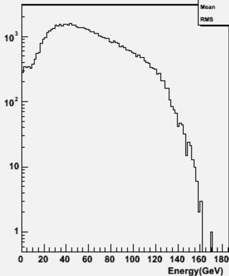
Particle Energy : w103972 aa_n2e2e2n2_o
