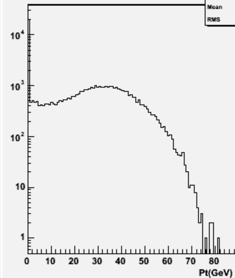
Particle Pt : w103970 aa_n2e2e1n1_o
