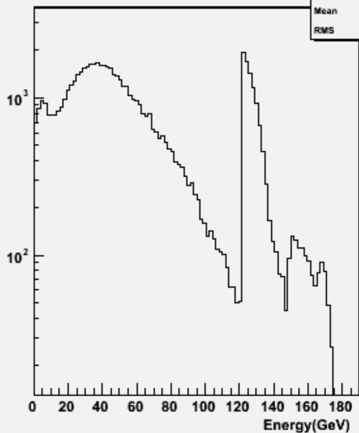
Particle Energy : w103970 aa_n2e2e1n1_o
