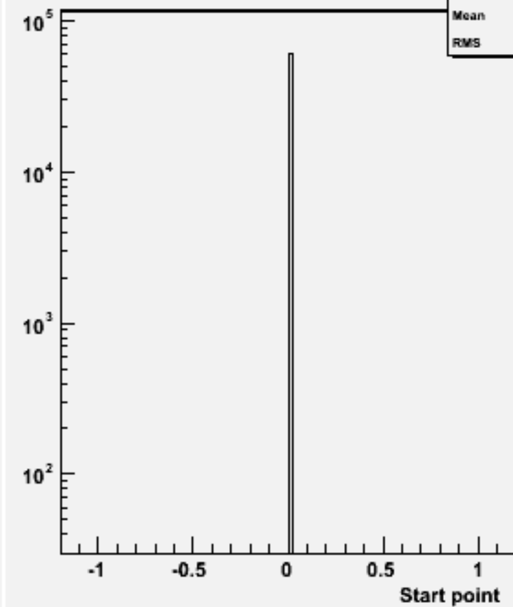
Start point Z : w103970 aa_n2e2e1n1_o
