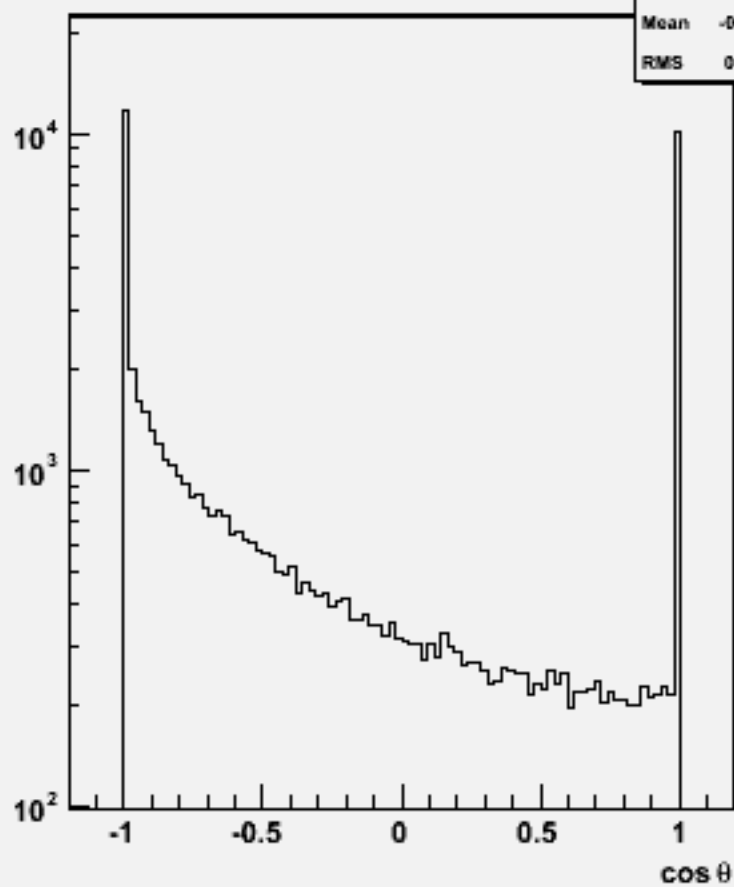
Particle cos \theta : w103970 aa_n2e2e1n1_o
