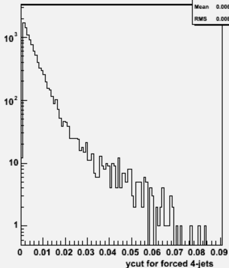
Ycut for 4-jets :w103966 aa_n1e1sc_o
