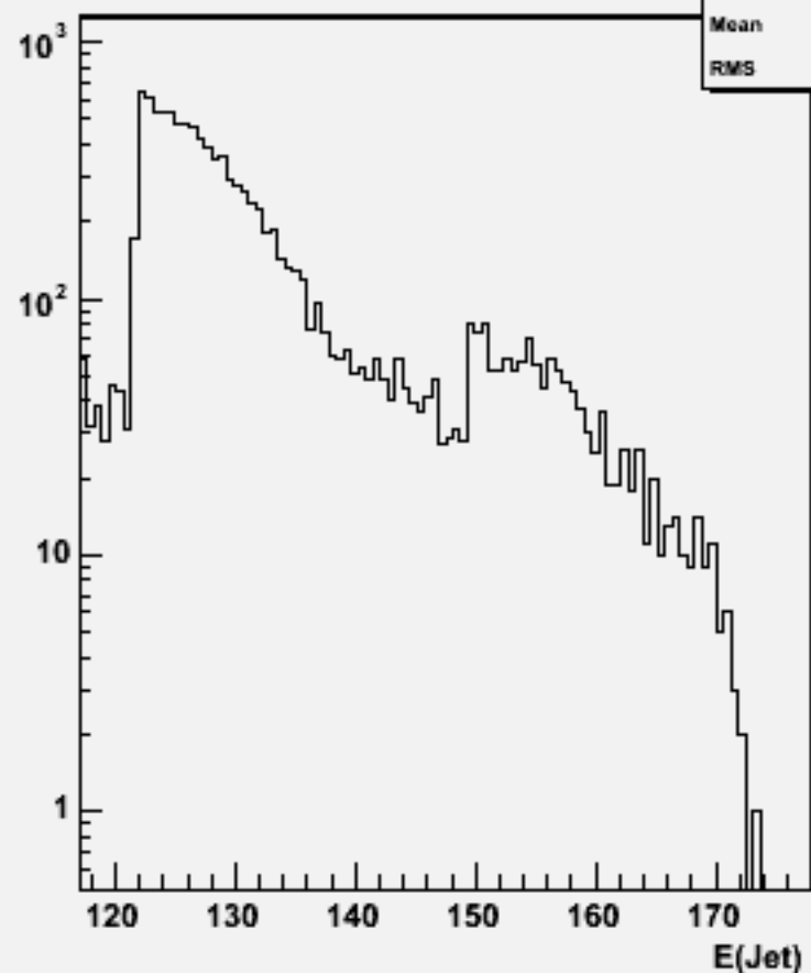
Jet energies(All jets)w103966 aa_n1e1sc_o
