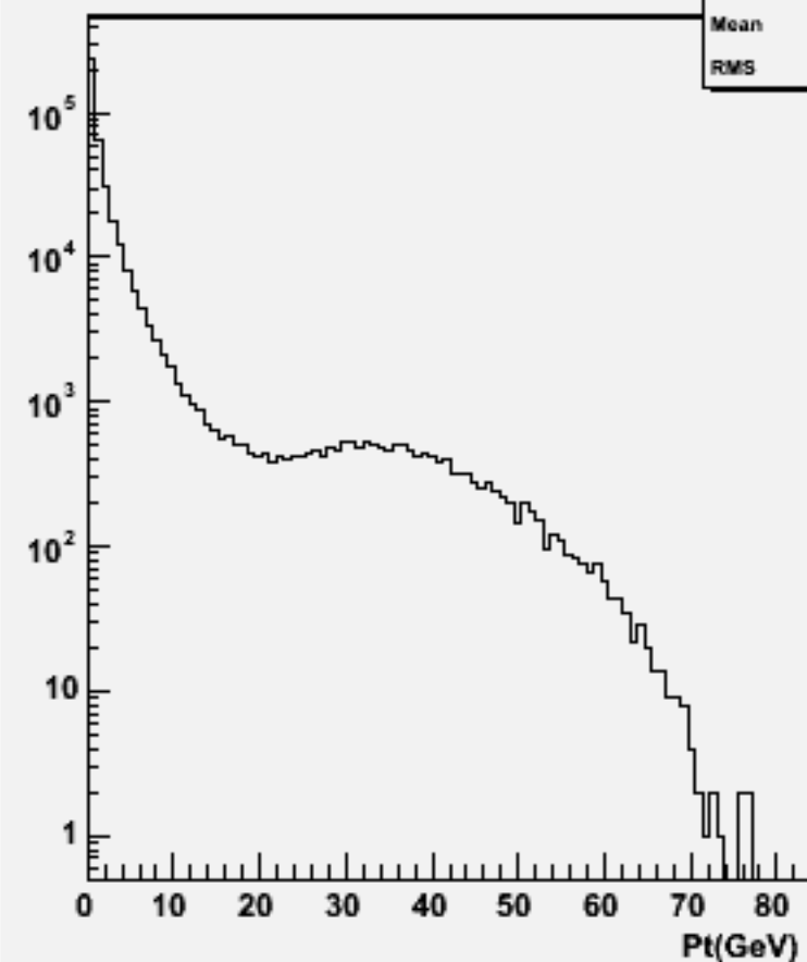
Particle Pt : w103966 aa_n1e1sc_o
