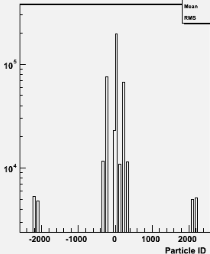
Particle ID : w103966 aa_n1e1sc_o
