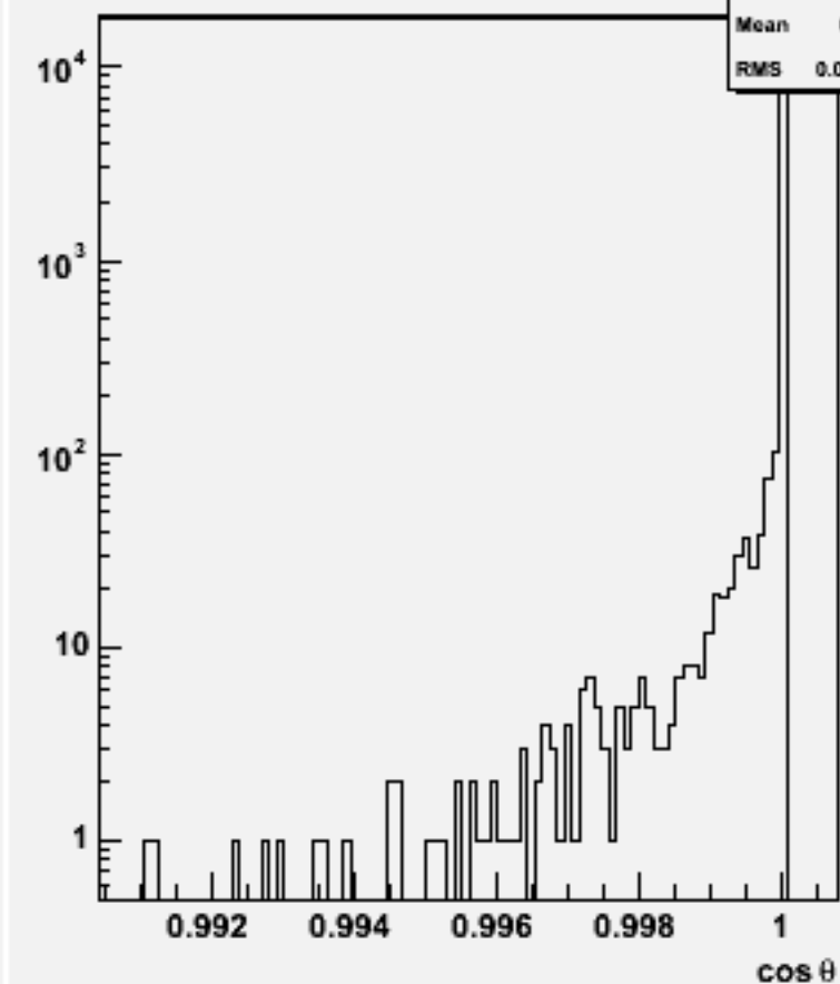
Jet cos \theta (All jets)w103966 aa_n1e1sc_o
