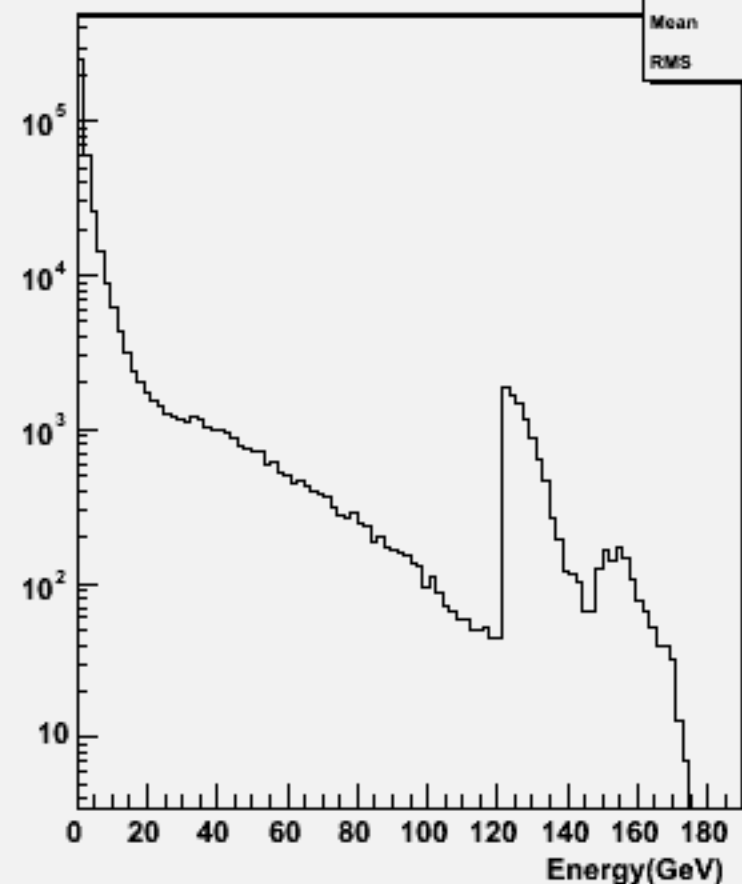
Particle Energy : w103966 aa_n1e1sc_o
