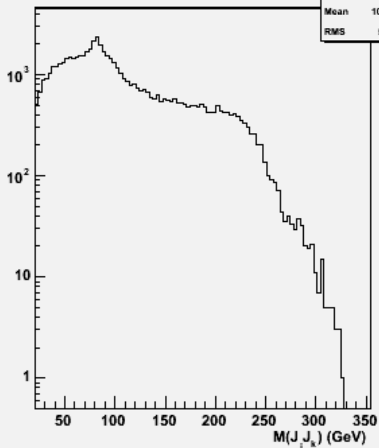
2jets mass(All comb)w103966 aa_n1e1sc_o
