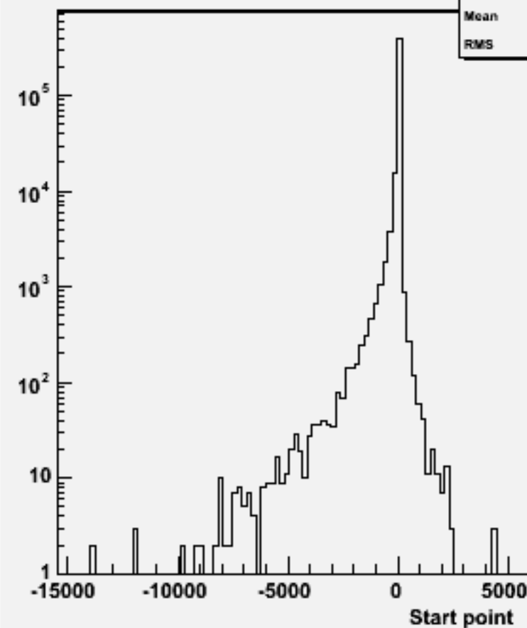
Start point Z : w103966 aa_n1e1sc_o
