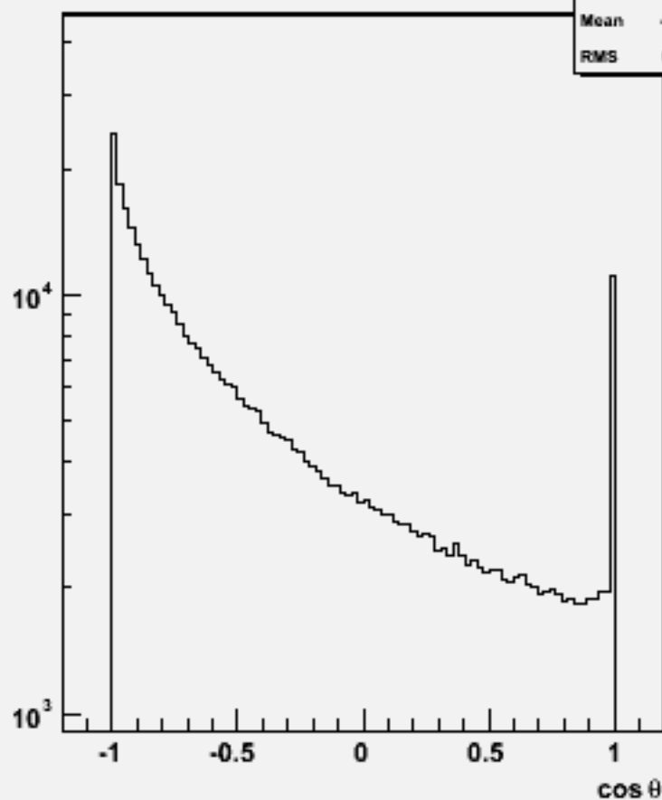
Particle cos \theta : w103966 aa_n1e1sc_o
