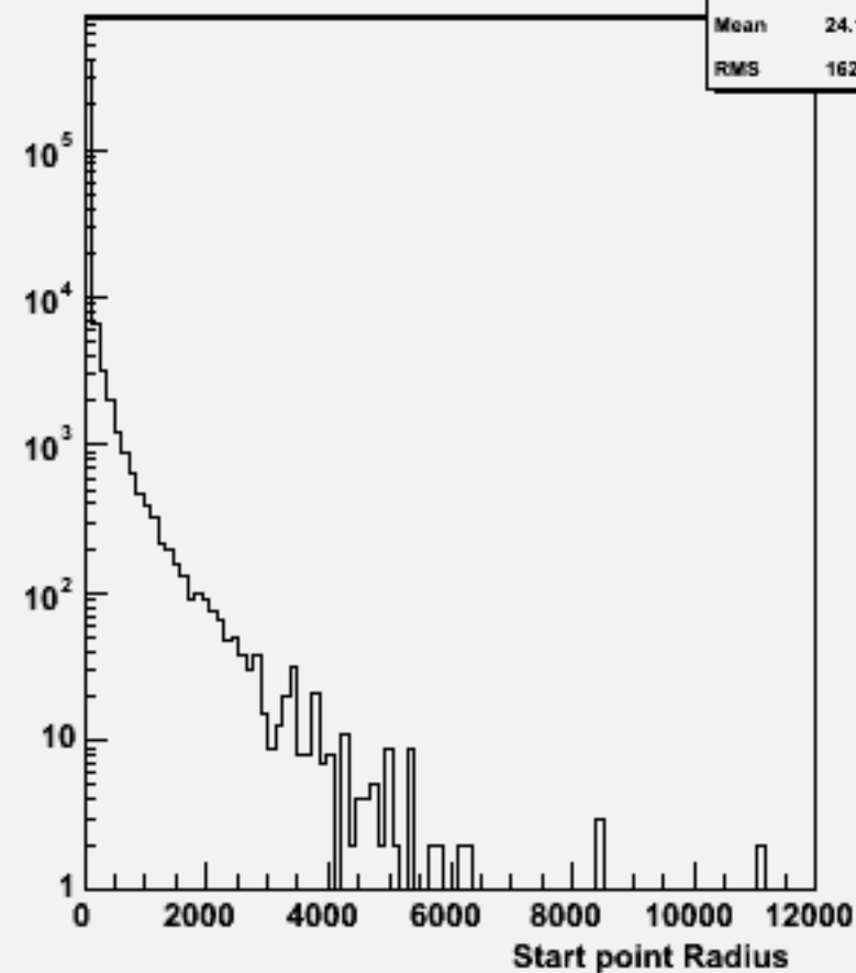
Start point R : w103966 aa_n1e1sc_o
