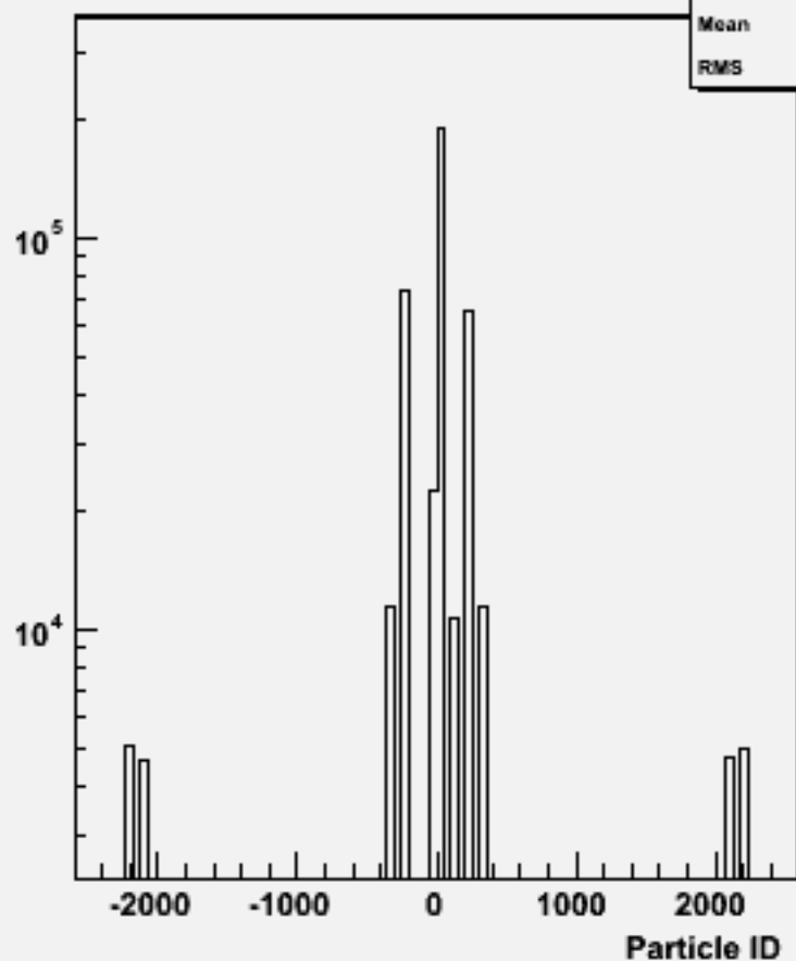
Particle ID : w103965 aa_n1e1sc_o
