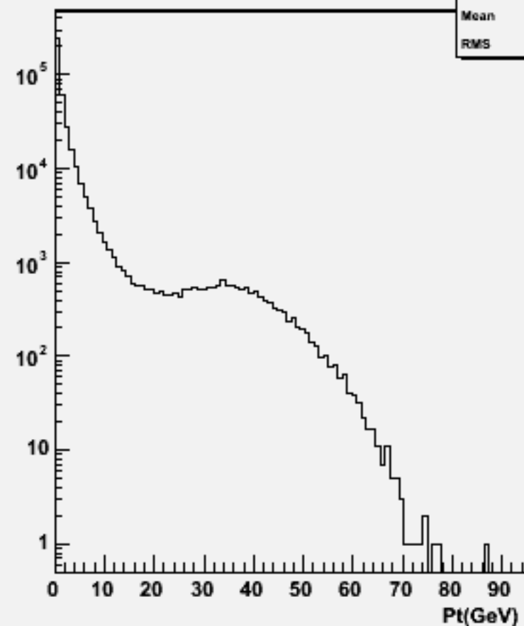
Particle Pt : w103965 aa_n1e1sc_o
