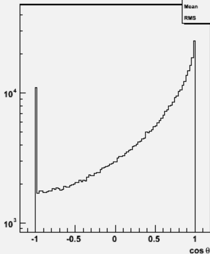
Particle cos \theta : w103965 aa_n1e1sc_o
