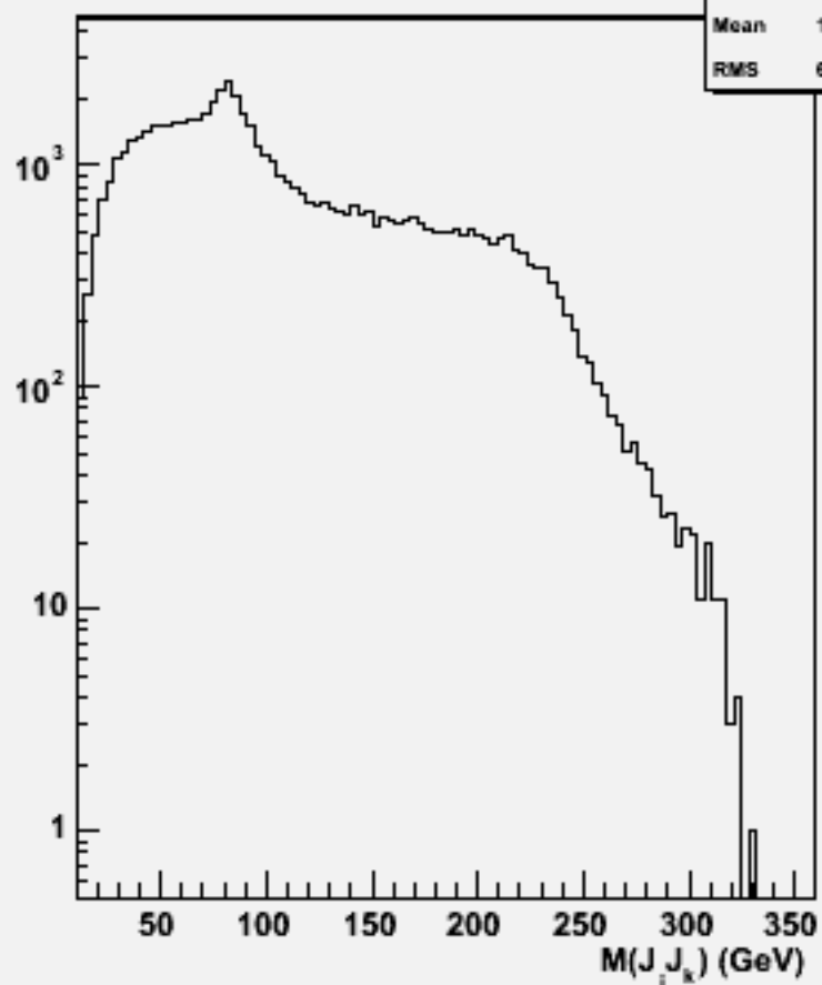
2jets mass(All comb)w103965 aa_n1e1sc_o
