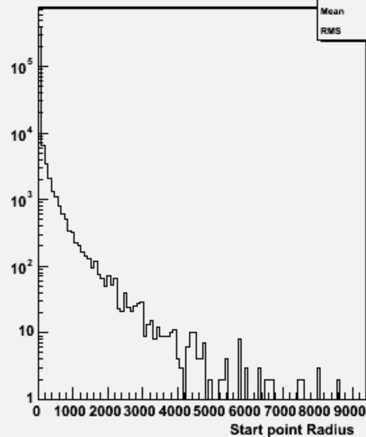
Start point R : w103965 aa_n1e1sc_o
