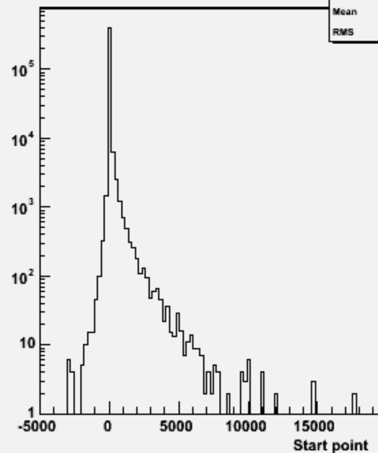
Start point Z : w103965 aa_n1e1sc_o
