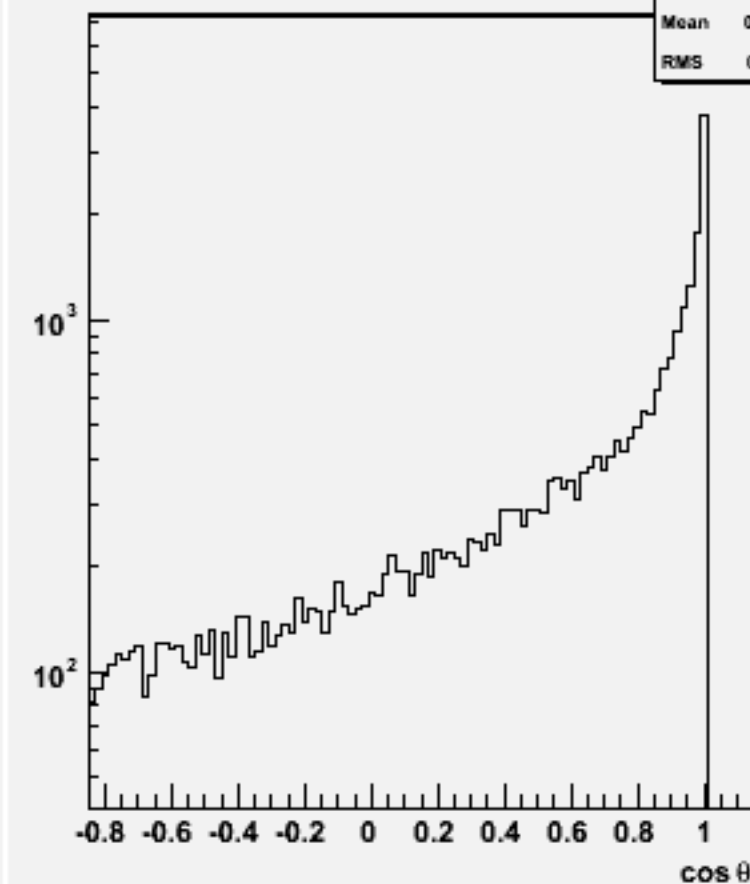
Jet cos \theta (All jets)w103965 aa_n1e1sc_o
