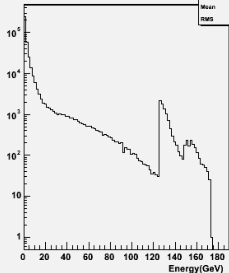
Particle Energy : w103965 aa_n1e1sc_o
