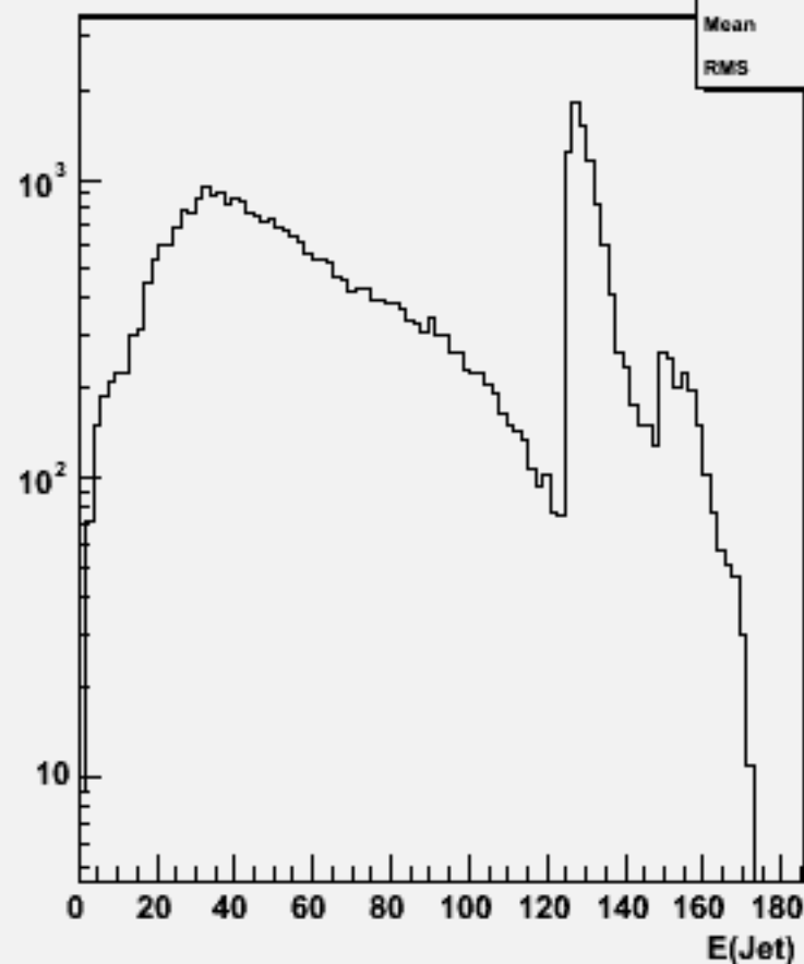
Jet energies(All jets)w103965 aa_n1e1sc_o
