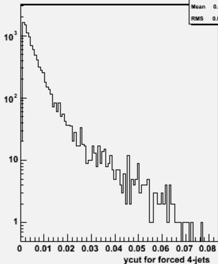
Ycut for 4-jets :w103965 aa_n1e1sc_o
