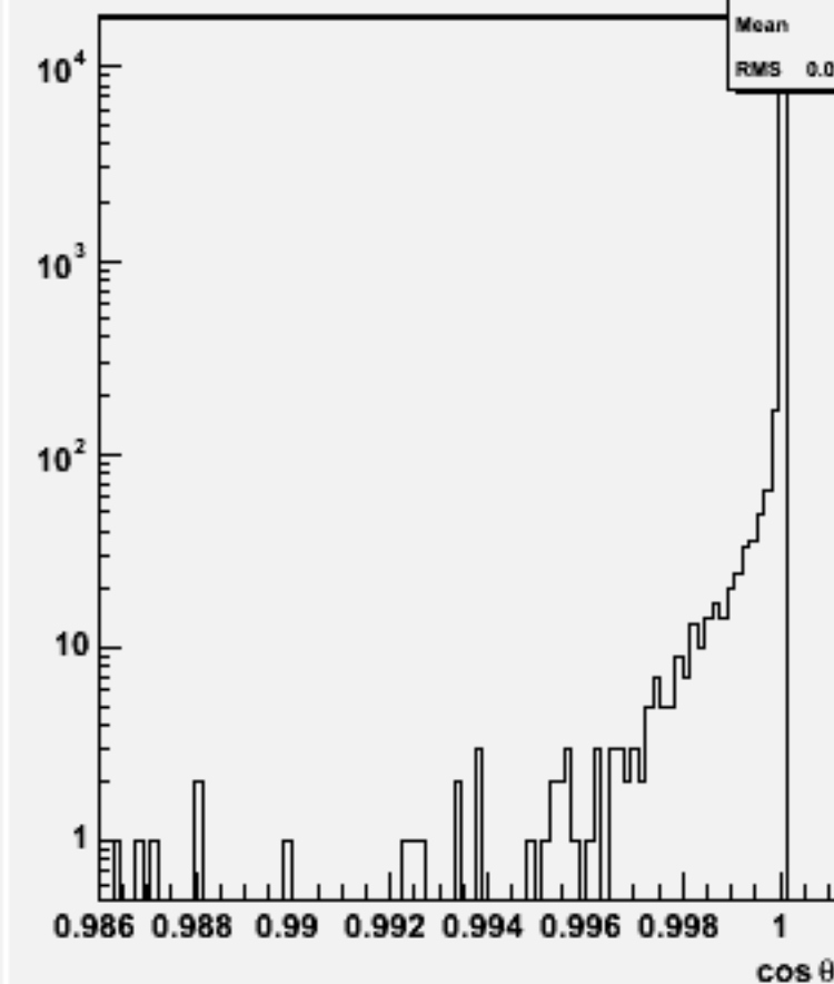
Jet cos \theta (All jets)w103962 aa_n1e1du_o
