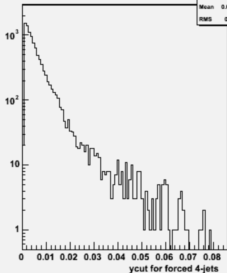
Ycut for 4-jets :w103962 aa_n1e1du_o
