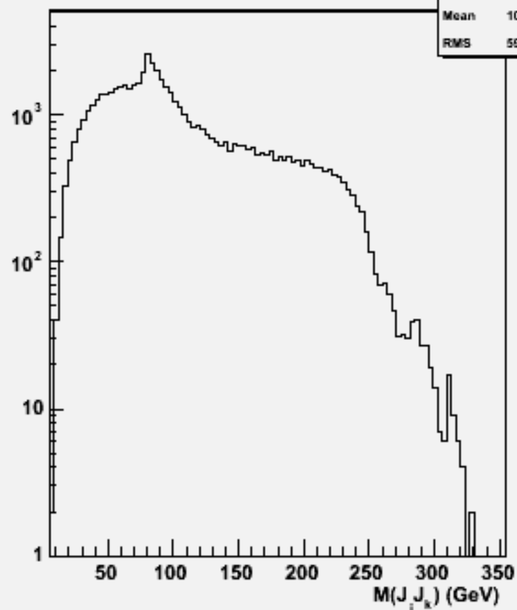
2jets mass(All comb)w103962 aa_n1e1du_o
