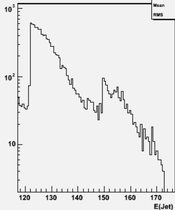
Jet energies(All jets)w103962 aa_n1e1du_o
