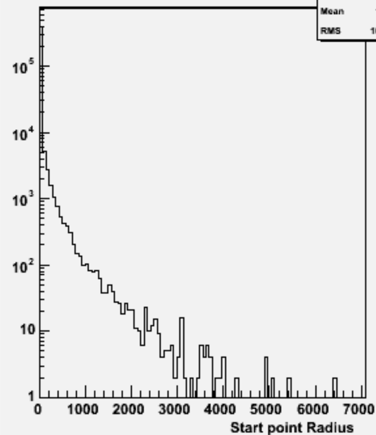
Start point R : w103962 aa_n1e1du_o
