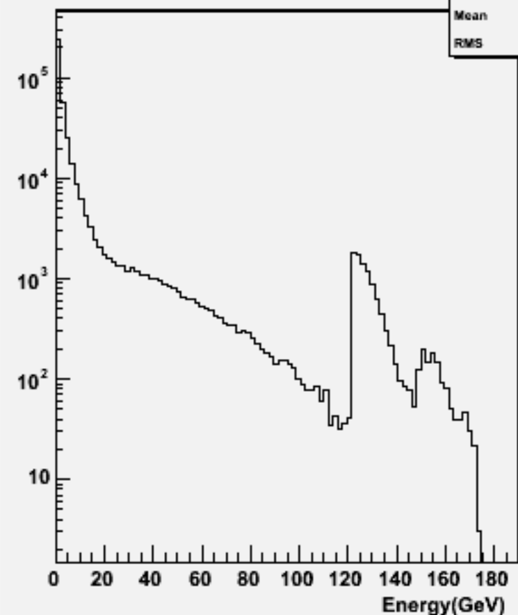
Particle Energy : w103962 aa_n1e1du_o
