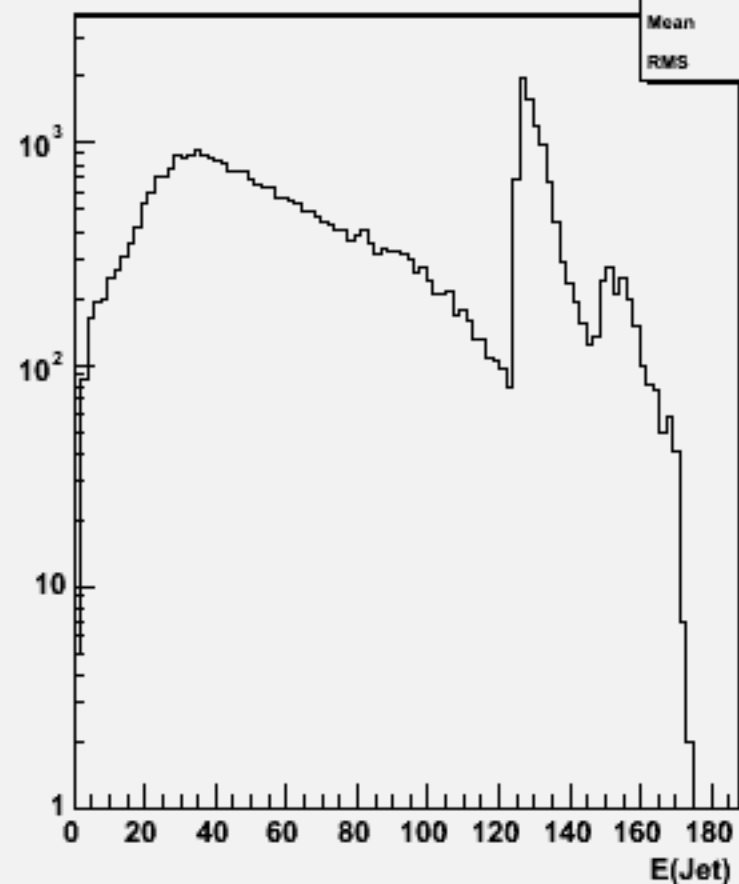
Jet energies(All jets)w103961 aa_n1e1du_o
