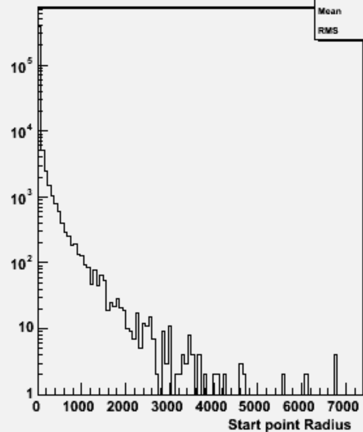
Start point R : w103961 aa_n1e1du_o
