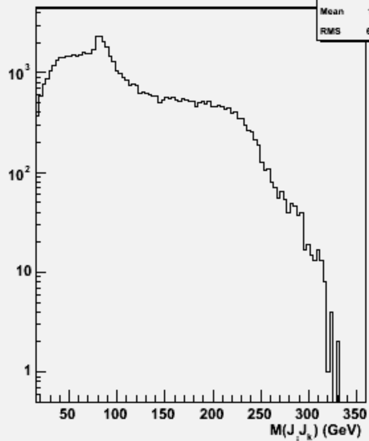
2jets mass(All comb)w103961 aa_n1e1du_o
