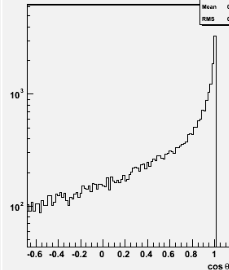
Jet cos \theta (All jets)w103961 aa_n1e1du_o
