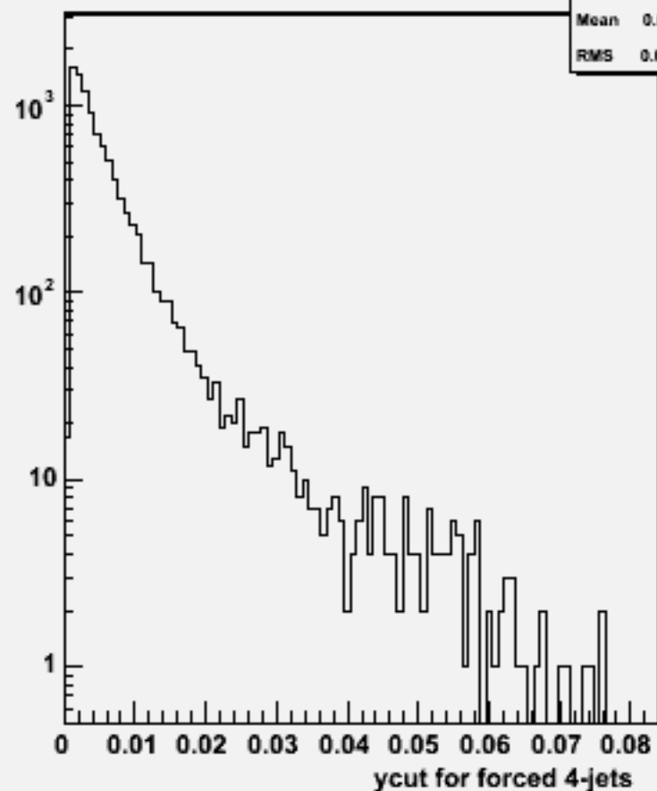
Ycut for 4-jets :w103961 aa_n1e1du_o
