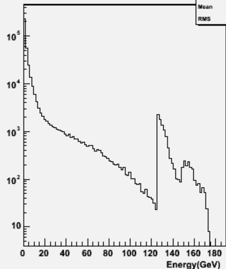
Particle Energy : w103961 aa_n1e1du_o
