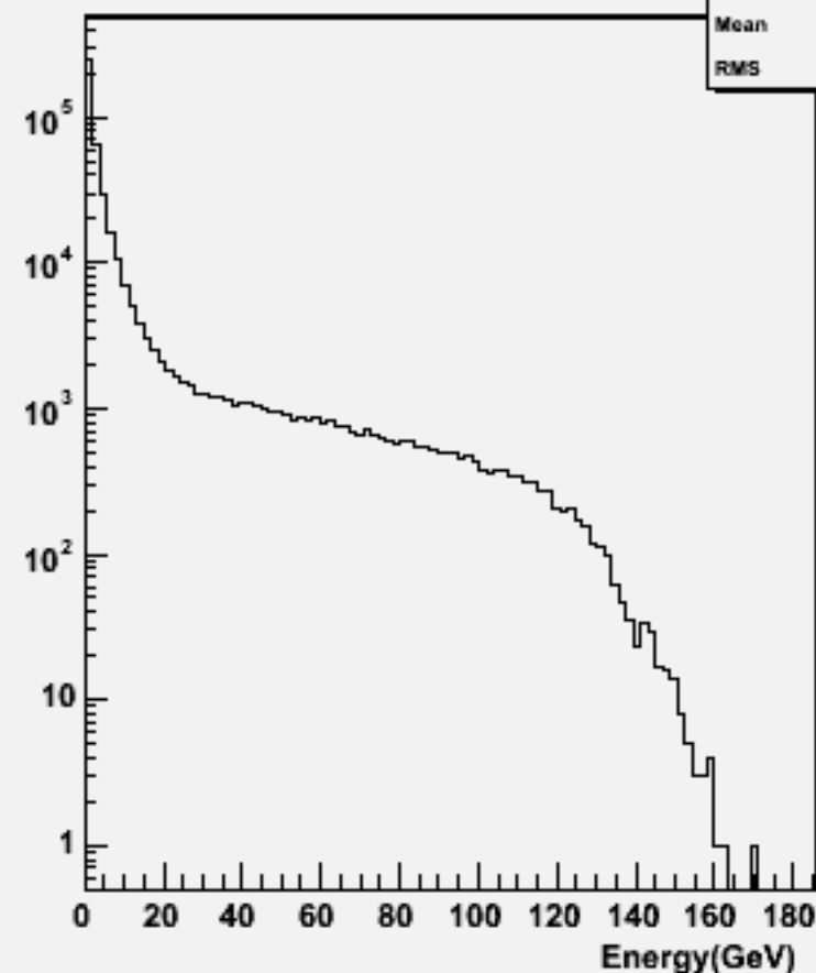
Particle Energy : w103960 aa_n1e1du_o
