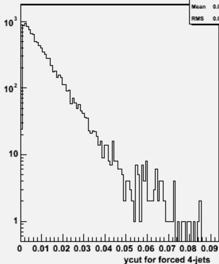
Ycut for 4-jets :w103960 aa_n1e1du_o
