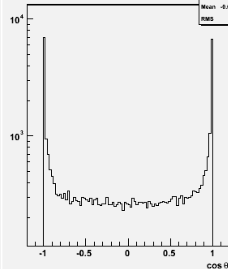
Jet cos \theta (All jets)w103960 aa_n1e1du_o
