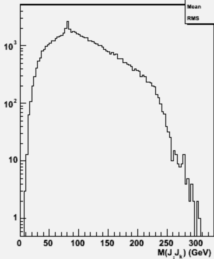
2jets mass(All comb)w103960 aa_n1e1du_o
