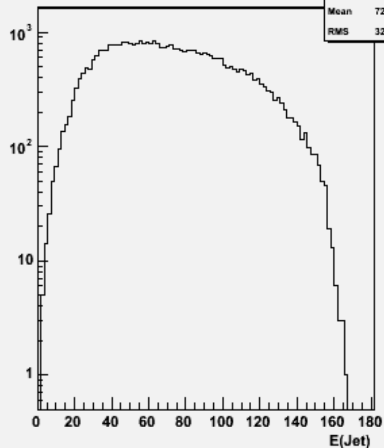
Jet energies(All jets)w103960 aa_n1e1du_o
