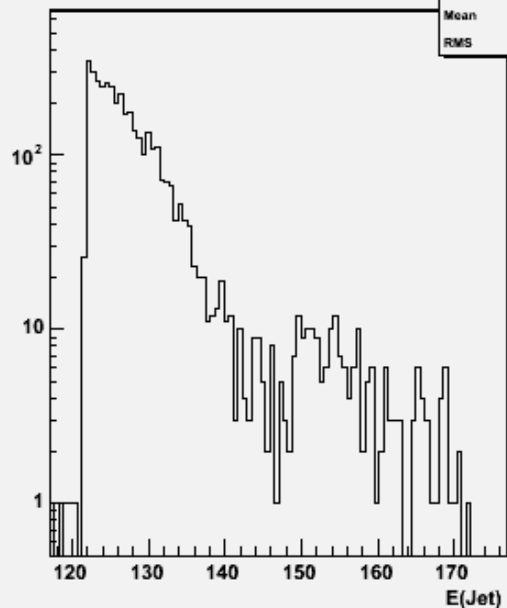
Jet energies(All jets)w103958 aa_n1e1e3n3_o
