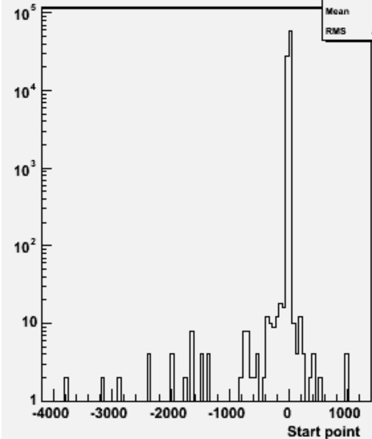
Start point Z : w103958 aa_n1e1e3n3_o
