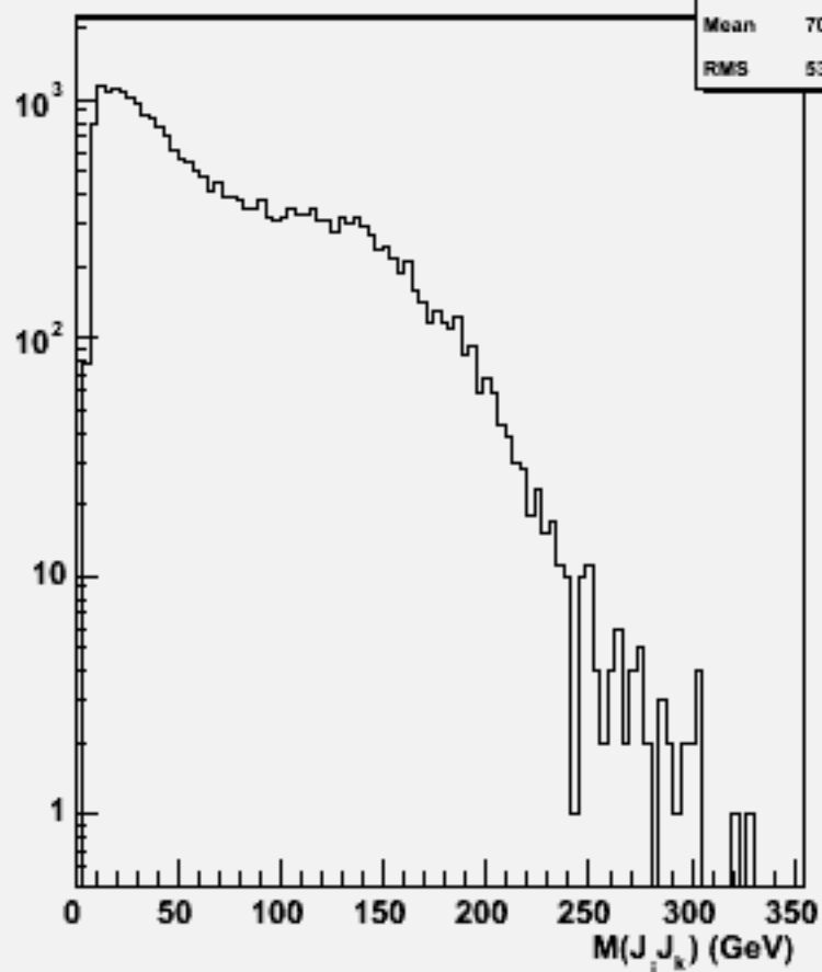
2jets mass(All comb)w103958 aa_n1e1e3n3_o
