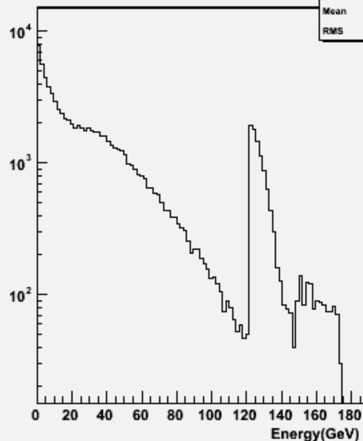
Particle Energy : w103958 aa_n1e1e3n3_o
