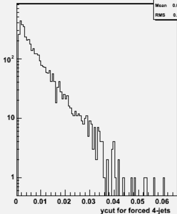
Ycut for 4-jets :w103958 aa_n1e1e3n3_o
