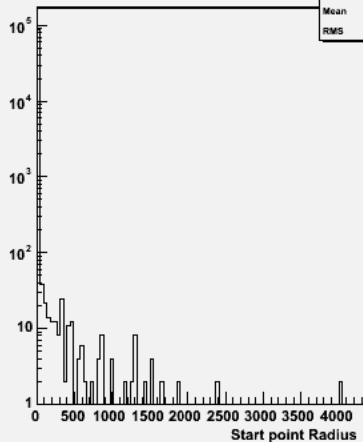
Start point R : w103958 aa_n1e1e3n3_o
