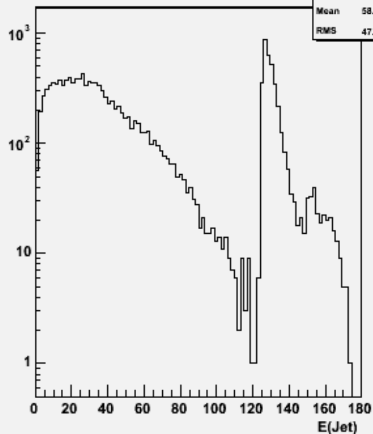
Jet energies(All jets)w103957 aa_n1e1e3n3_o
