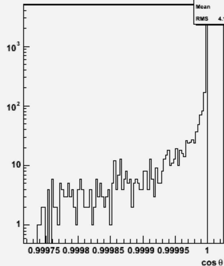
Jet cos \theta (All jets)w103957 aa_n1e1e3n3_o
