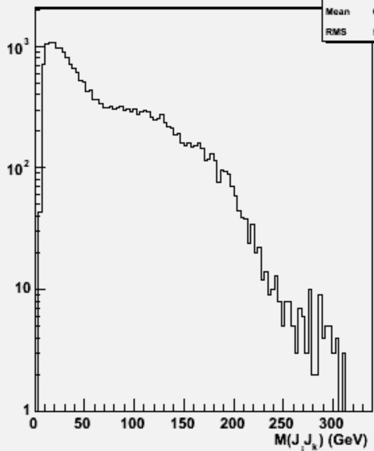
2jets mass(All comb)w103957 aa_n1e1e3n3_o
