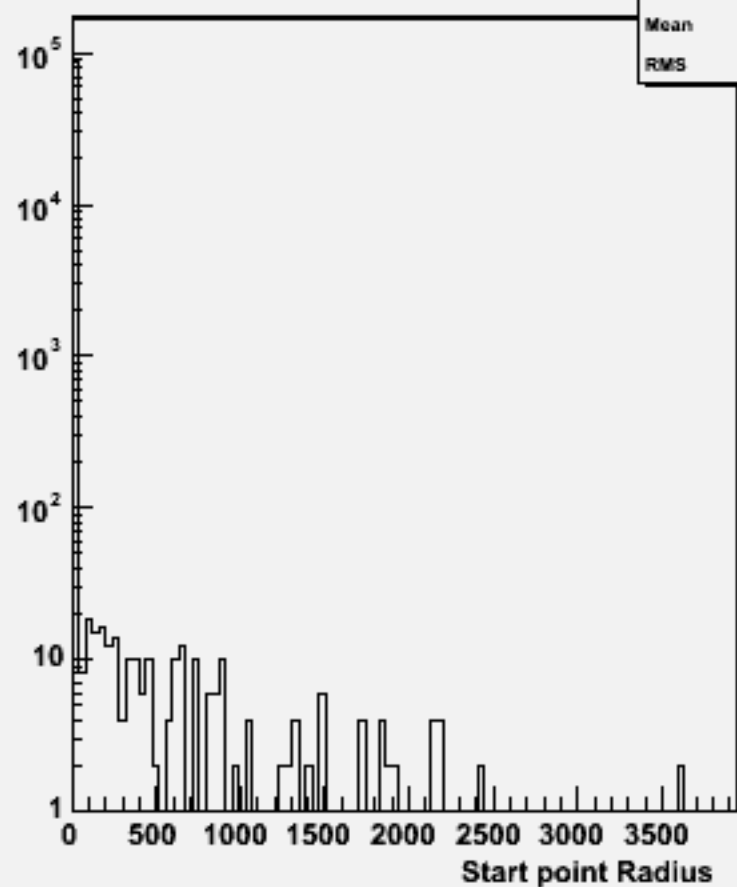
Start point R : w103957 aa_n1e1e3n3_o
