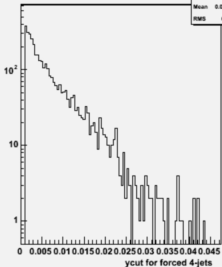
Ycut for 4-jets :w103957 aa_n1e1e3n3_o
