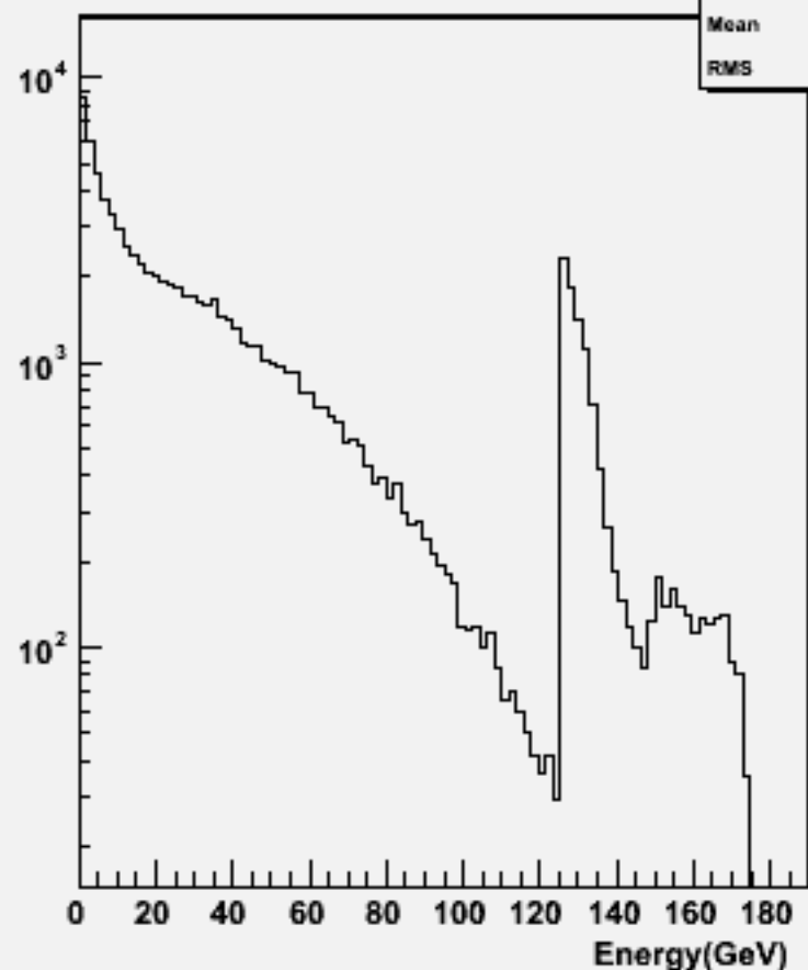
Particle Energy : w103957 aa_n1e1e3n3_o
