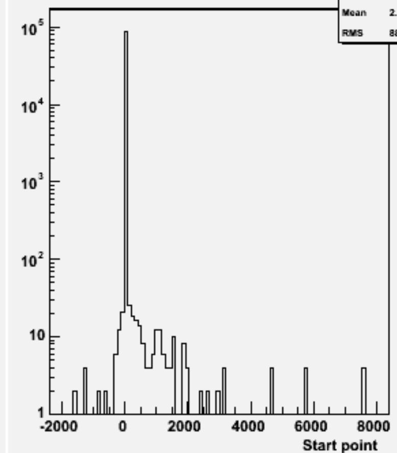
Start point Z : w103957 aa_n1e1e3n3_o
