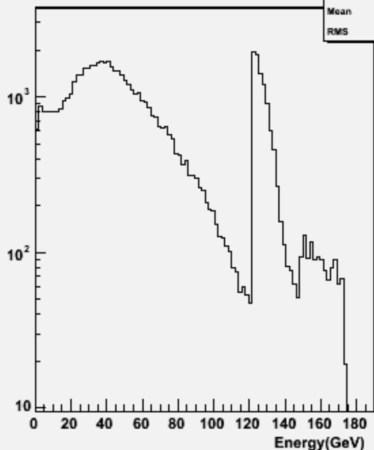
Particle Energy : w103954 aa_n1e1e2n2_o
