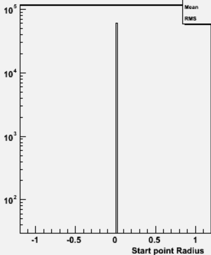
Start point R : w103953 aa_n1e1e2n2_o
