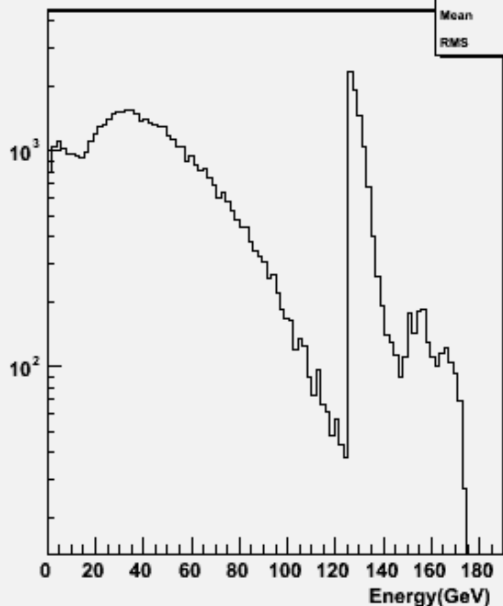
Particle Energy : w103953 aa_n1e1e2n2_o
