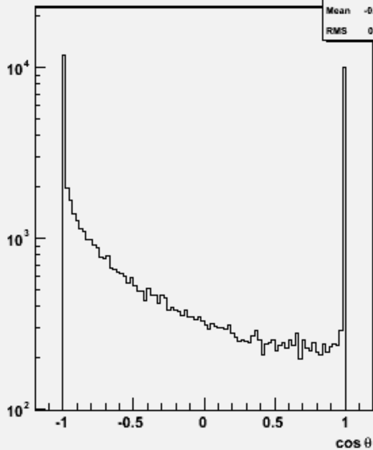
Particle cos \theta : w103950 aa_n1e1e1n1_o
