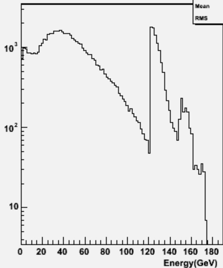
Particle Energy : w103950 aa_n1e1e1n1_o
