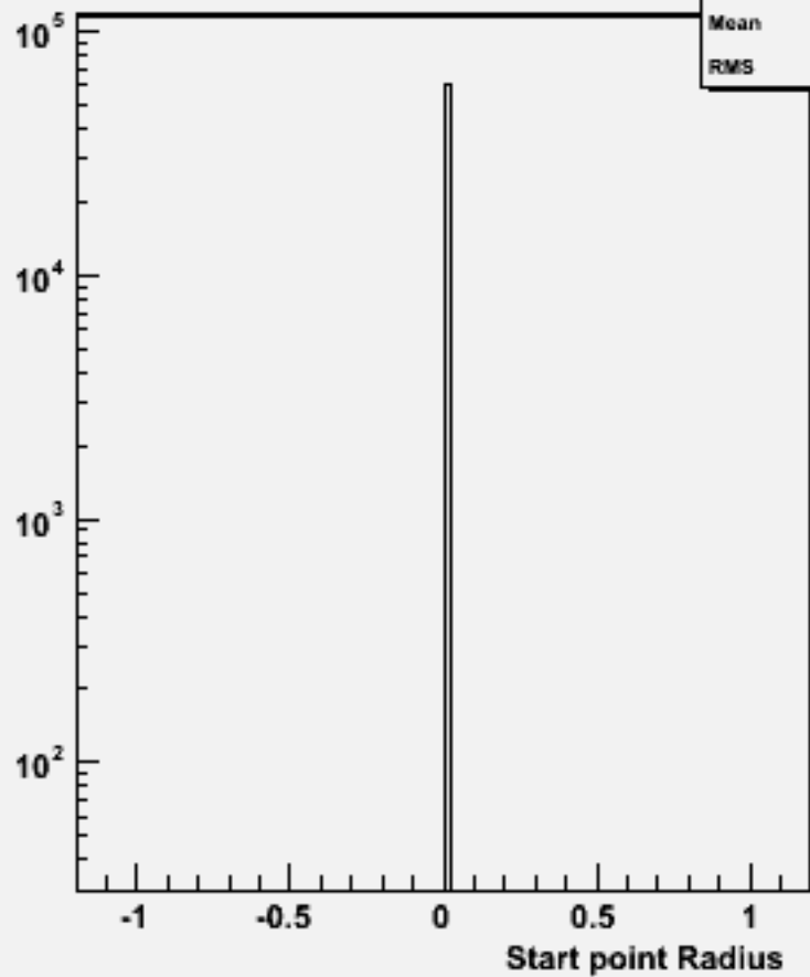
Start point R : w103950 aa_n1e1e1n1_o
