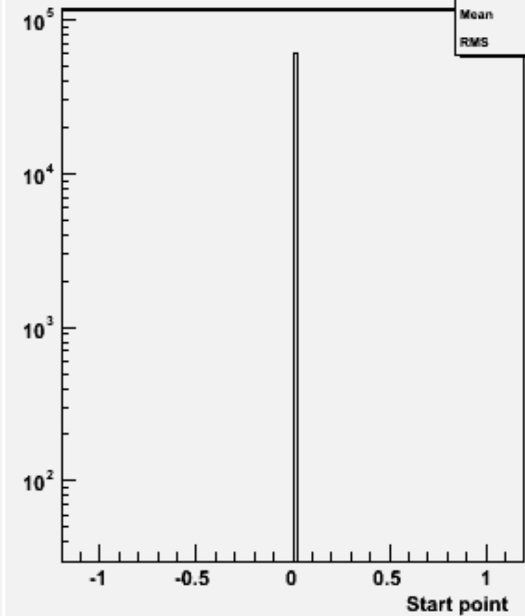
Start point Z : w103950 aa_n1e1e1n1_o
