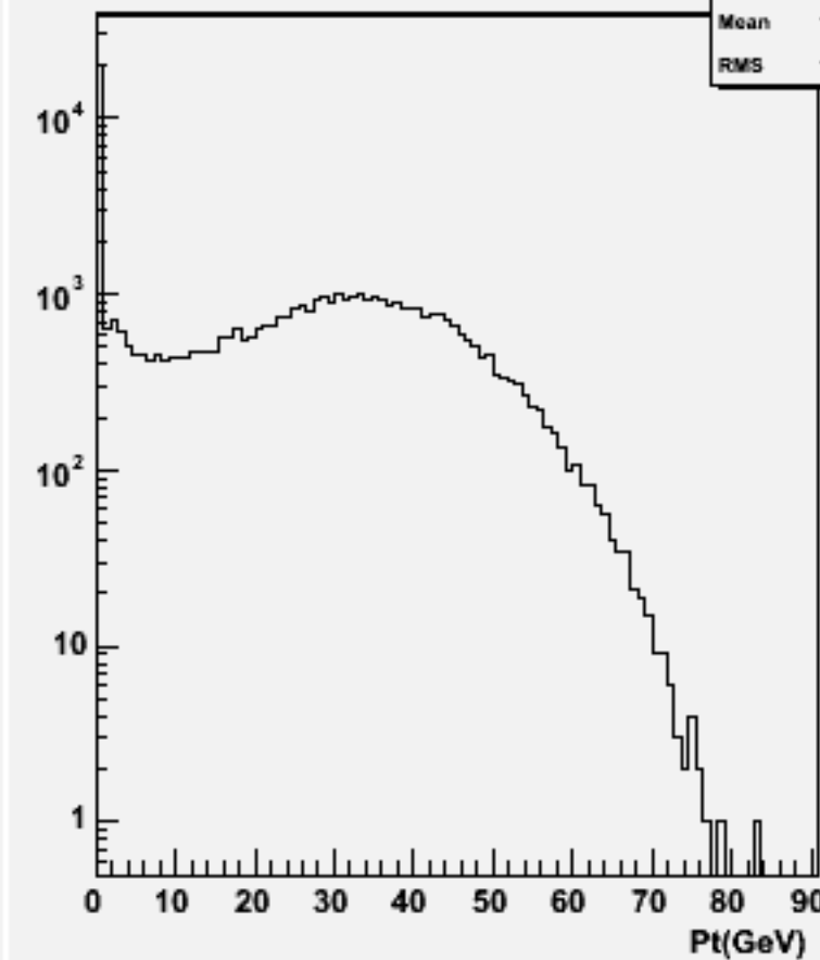
Particle Pt : w103950 aa_n1e1e1n1_o
