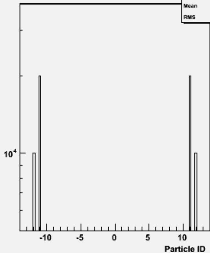
Particle ID : w103950 aa_n1e1e1n1_o
