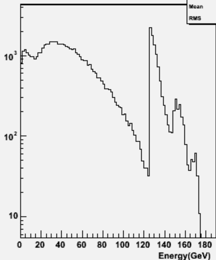
Particle Energy : w103949 aa_n1e1e1n1_o
