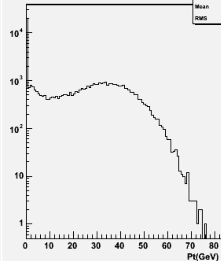
Particle Pt : w103949 aa_n1e1e1n1_o
