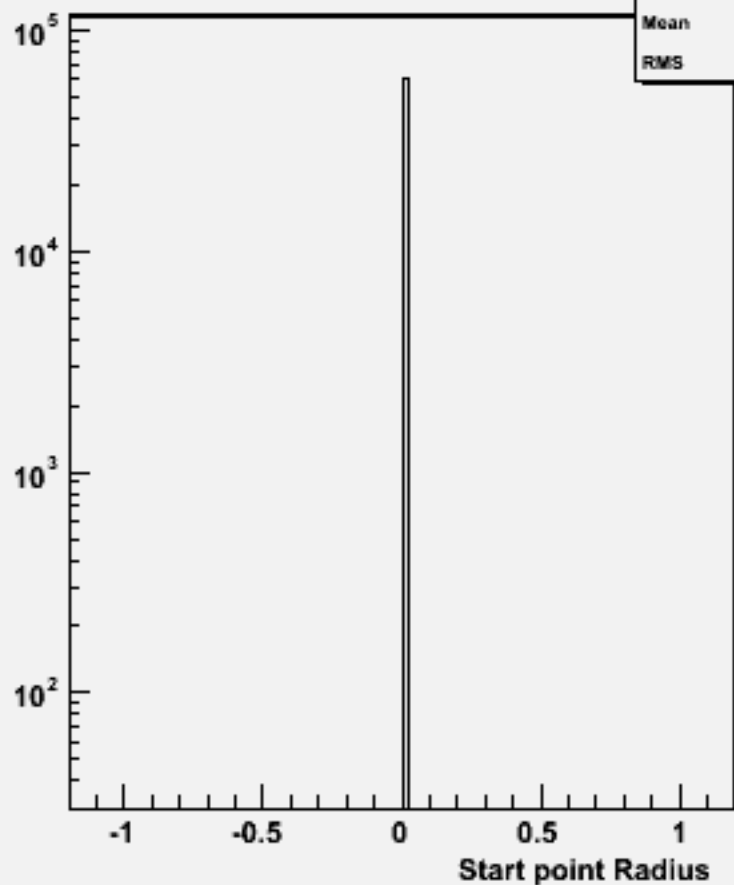
Start point R : w103949 aa_n1e1e1n1_o
