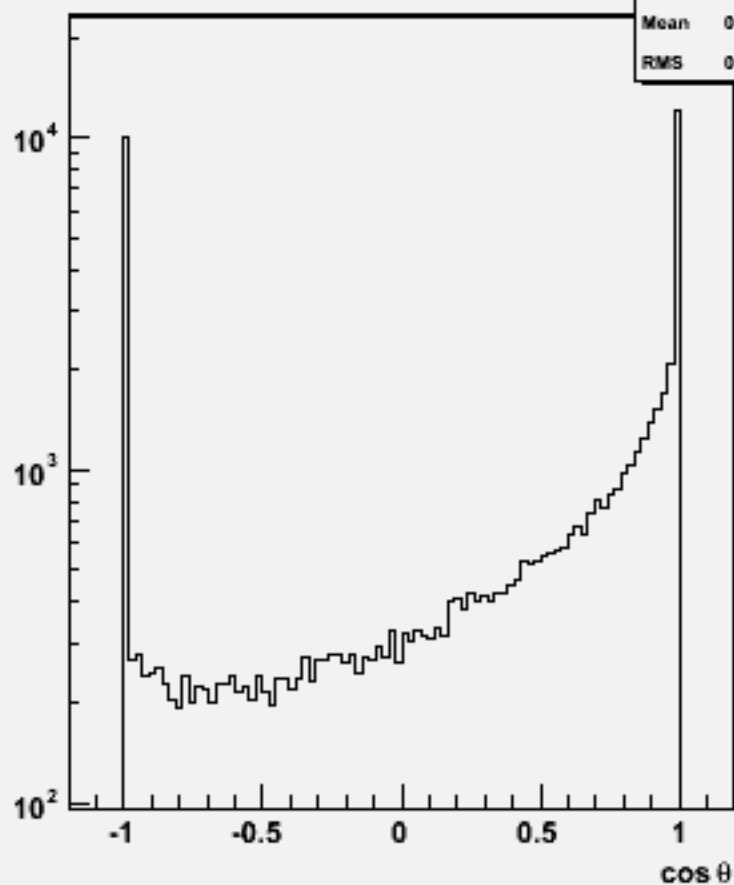
Particle cos \theta : w103949 aa_n1e1e1n1_o
