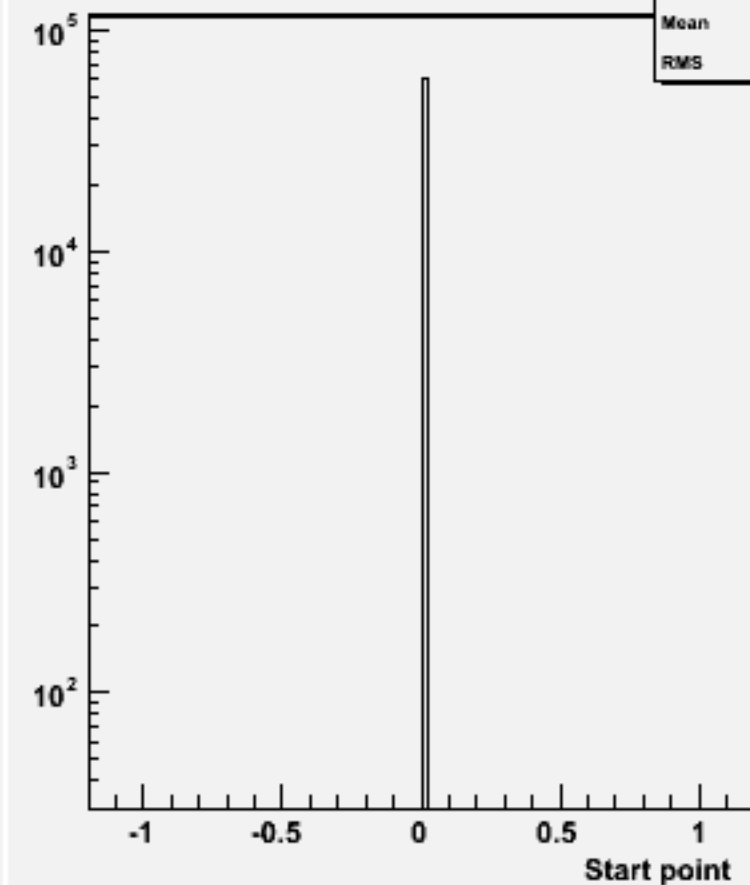
Start point Z : w103949 aa_n1e1e1n1_o
