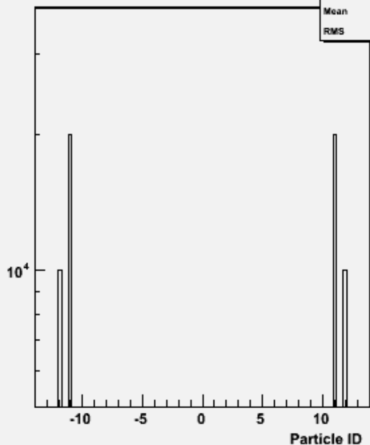
Particle ID : w103948 aa_n1e1e1n1_o
