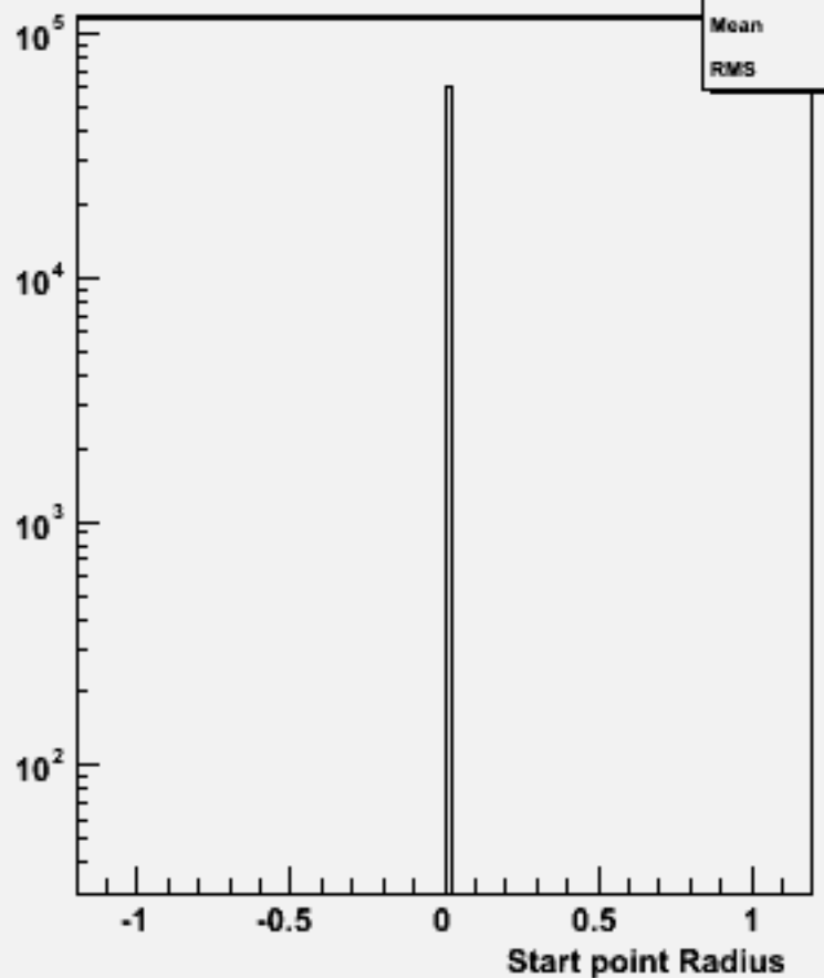
Start point R : w103948 aa_n1e1e1n1_o
