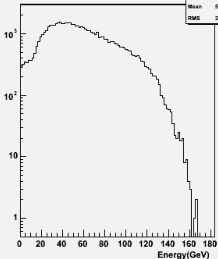
Particle Energy : w103948 aa_n1e1e1n1_o
