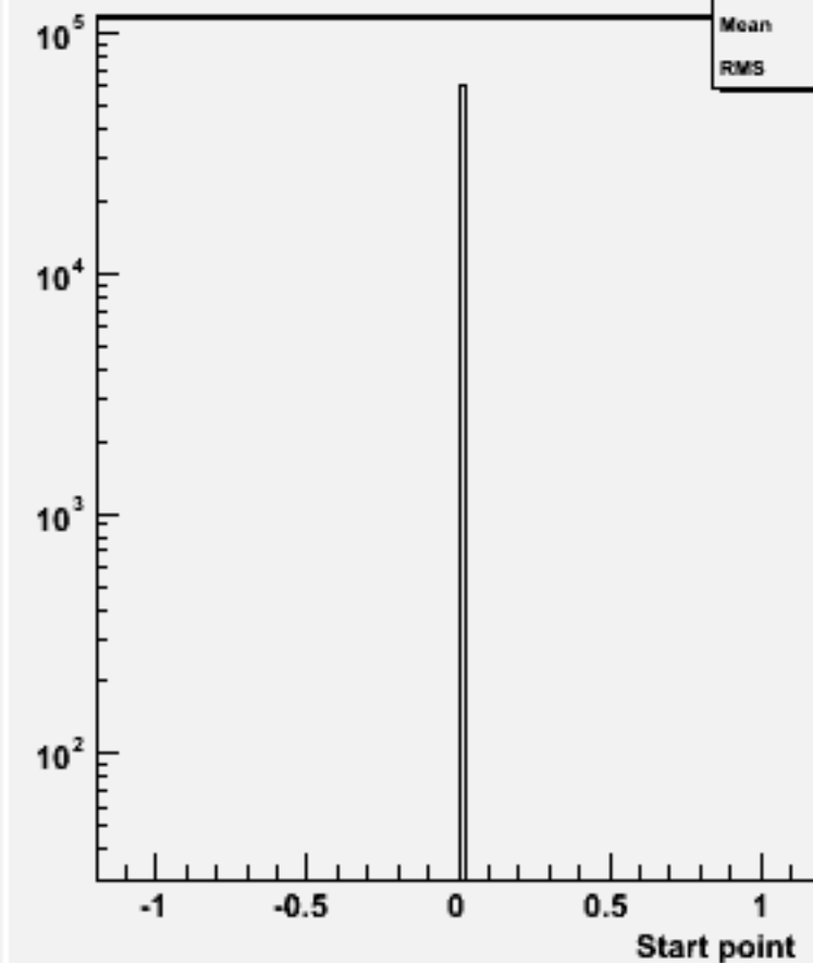
Start point Z : w103948 aa_n1e1e1n1_o
