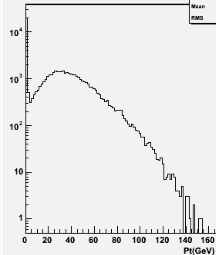
Particle Pt : w103948 aa_n1e1e1n1_o
