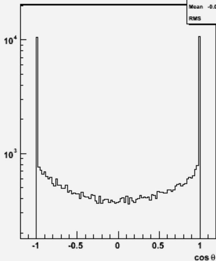
Particle cos \theta : w103948 aa_n1e1e1n1_o
