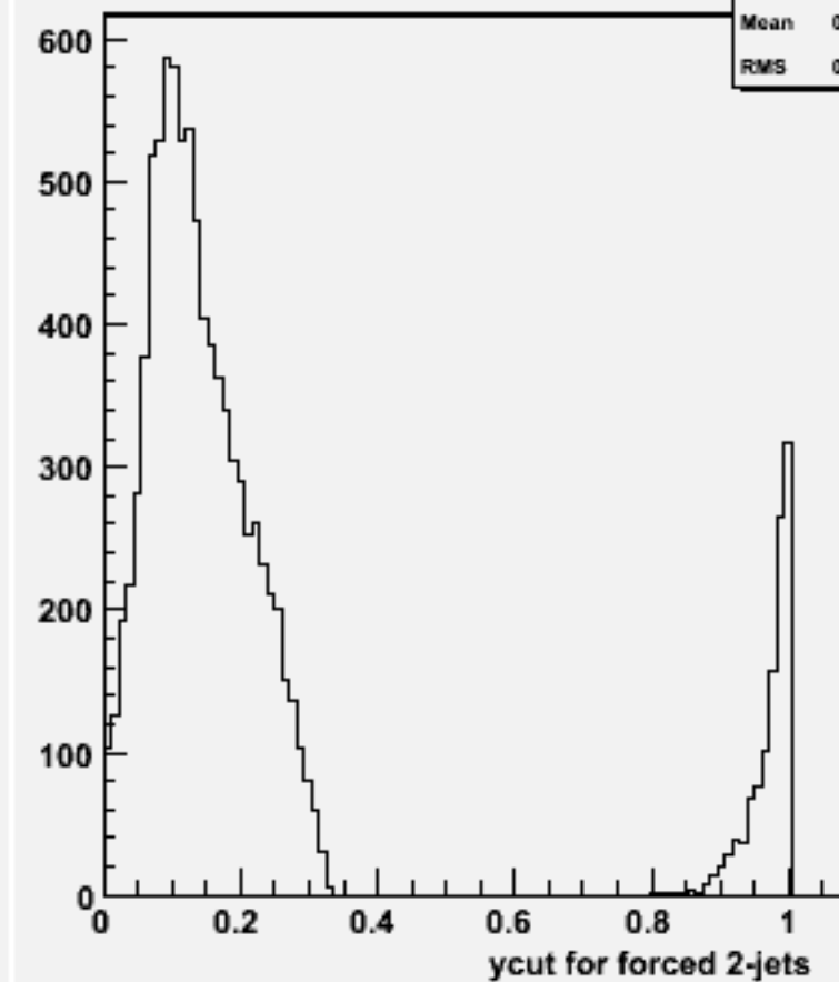
Ycut for 2-jets :w103944 ae1_e1bbbb_o
