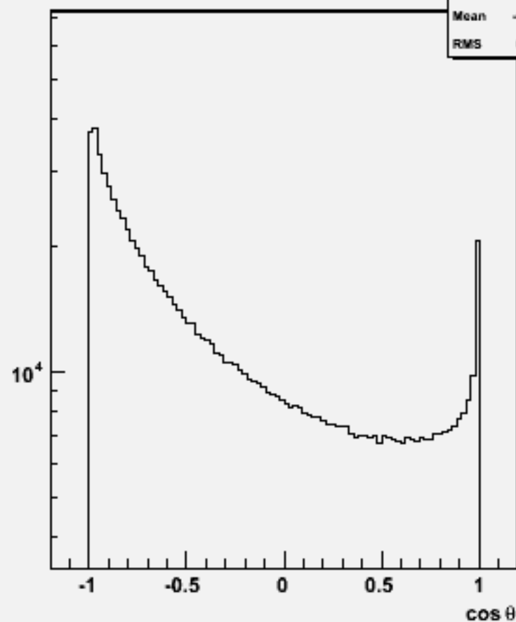
Particle cos \theta : w103944 ae1_e1bbbb_o
