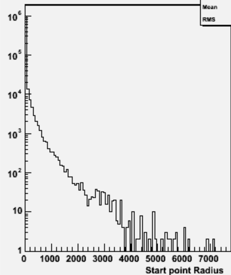
Start point R : w103944 ae1_e1bbbb_o
