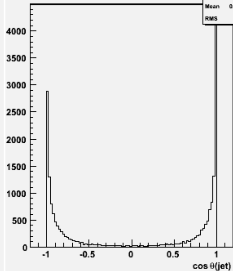
cos \theta for 2-jets :w103944 ae1_e1bbbb_o
