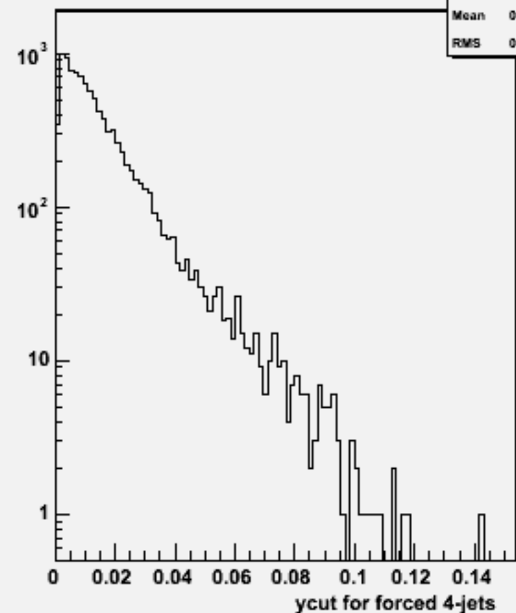
Ycut for 4-jets :w103944 ae1_e1bbbb_o
