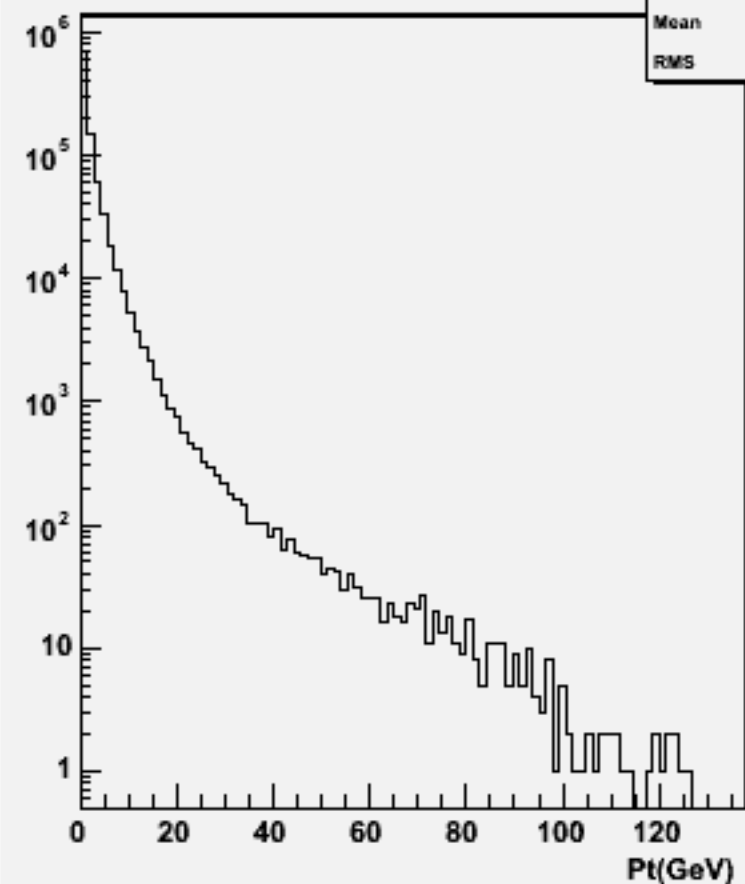
Particle Pt : w103944 ae1_e1bbbb_o
