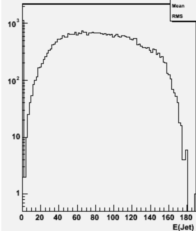
Jet energies(All jets)w103944 ae1_e1bbbb_o
