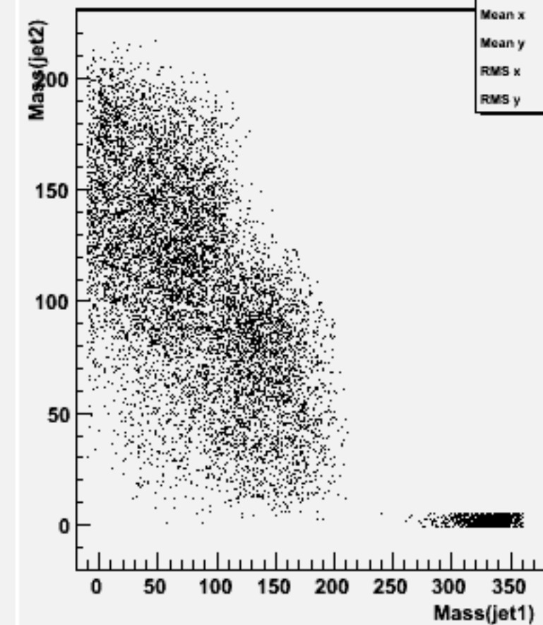
Jet mass for forced 2-jets : w103944 ae1_e1bbbb_o
