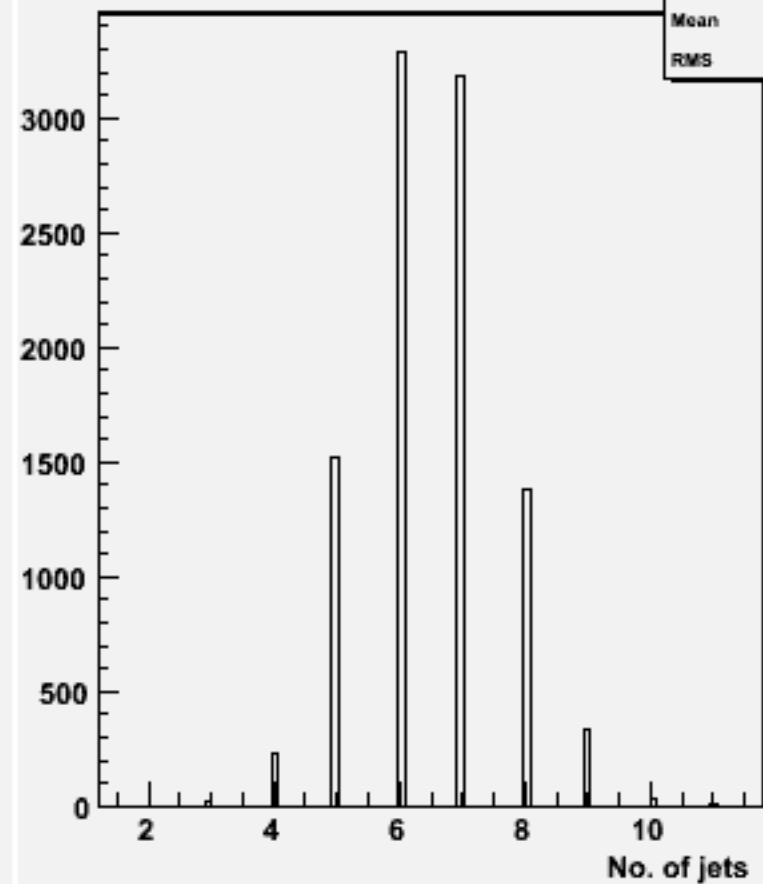
No. jets (ycut=0.001) : w103944 ae1_e1bbbb_o
