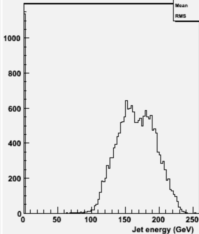
energy for 2-jets :w103944 ae1_e1bbbb_o
