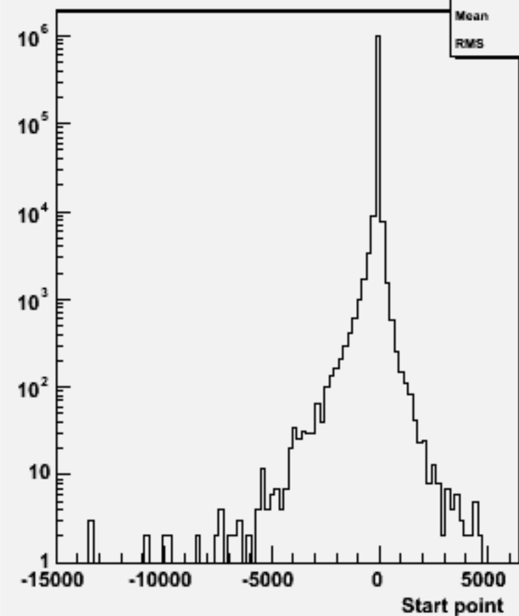
Start point Z : w103944 ae1_e1bbbb_o
