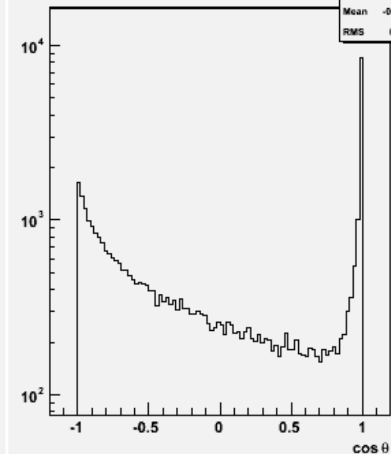
Jet cos \theta (All jets)w103944 ae1_e1bbbb_o
