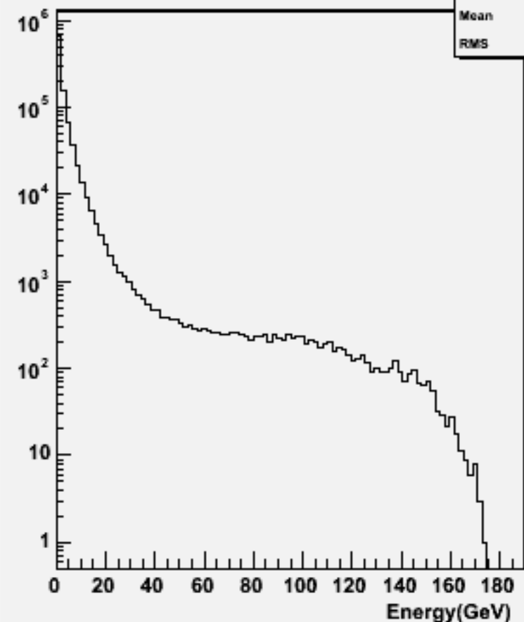
Particle Energy : w103944 ae1_e1bbbb_o
