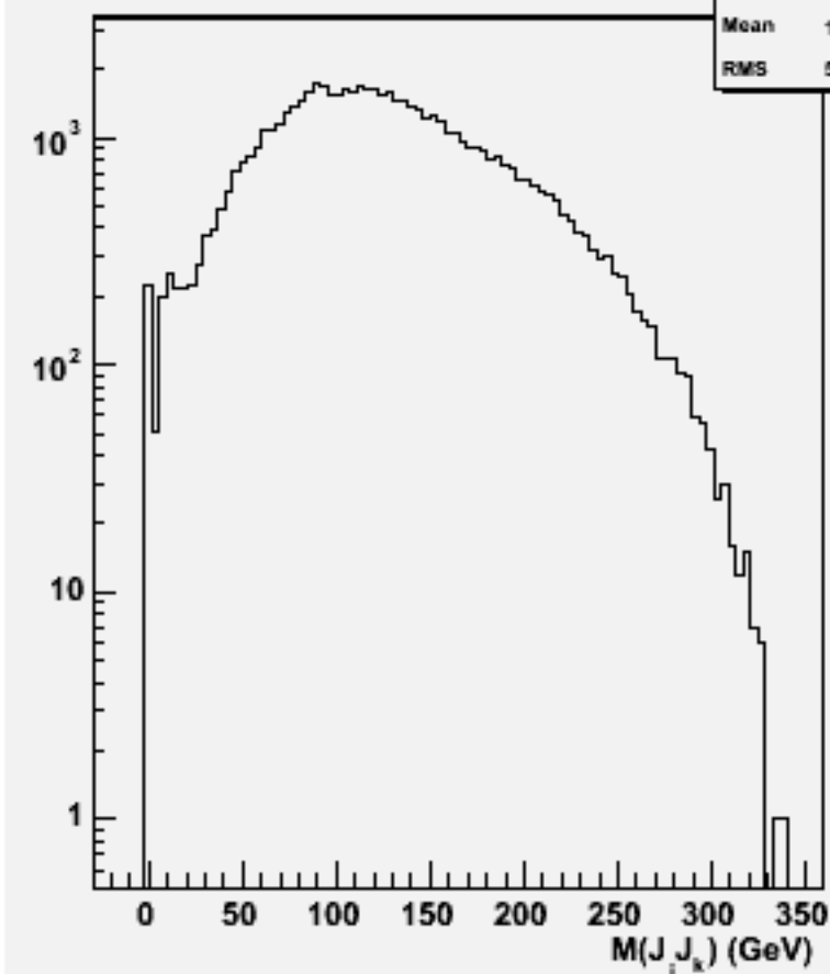
2jets mass(All comb)w103944 ae1_e1bbbb_o
