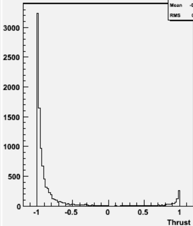
cos \Theta (thrust) w103944 ae1_e1bbbb_o
