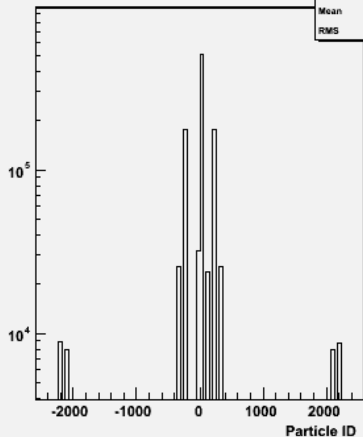
Particle ID : w103944 ae1_e1bbbb_o
