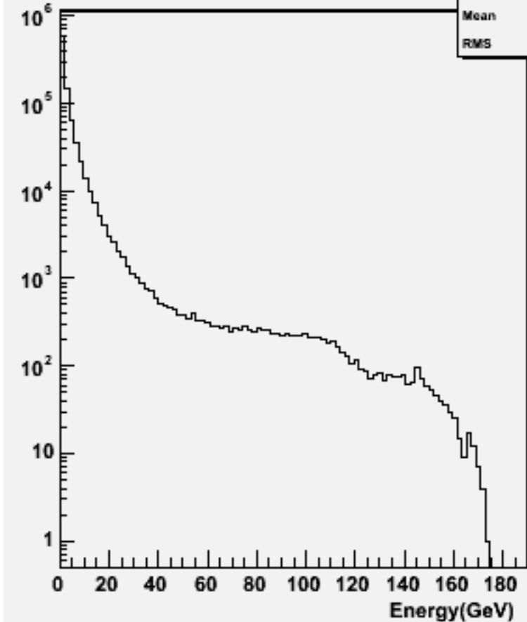
Particle Energy : w103942 ae1_e1ssbb_o
