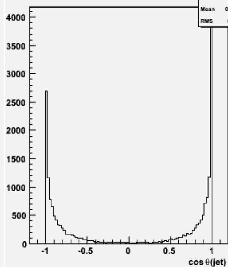
cos \theta for 2-jets :w103942 ae1_e1ssbb_o
