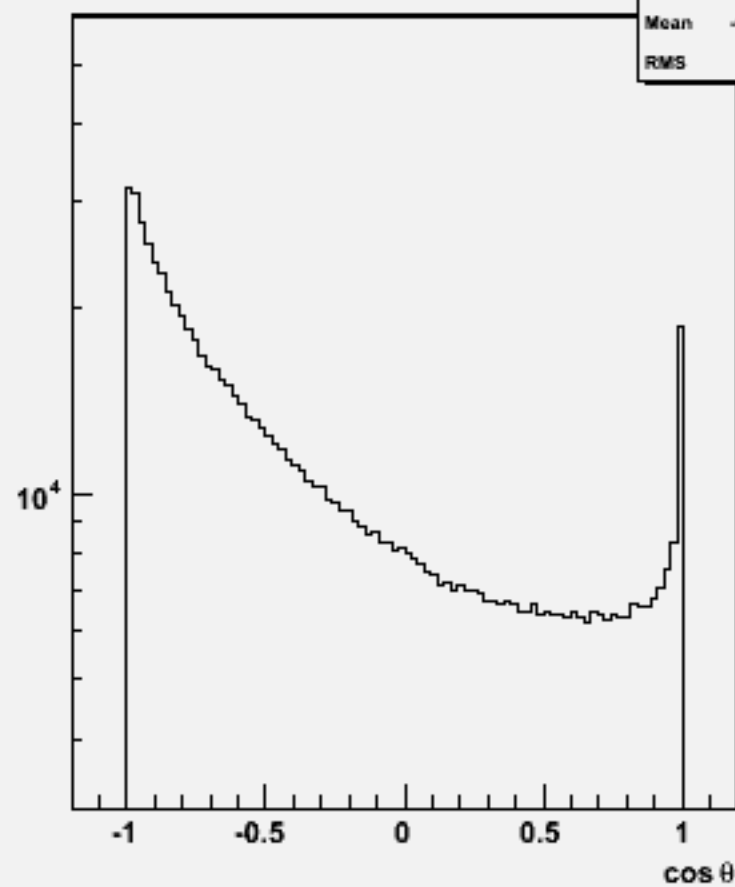
Particle cosθ : w103942 ae1_e1ssbb_o
