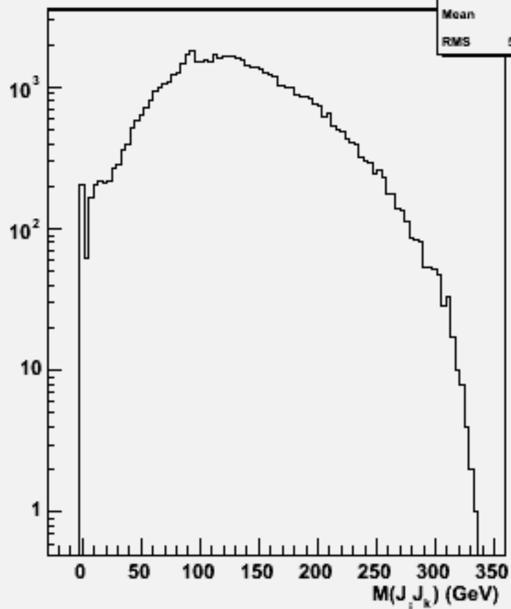
2jets mass(All comb)w103942 ae1_e1ssbb_o
