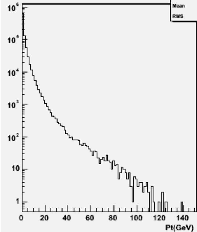
Particle Pt : w103942 ae1_e1ssbb_o
