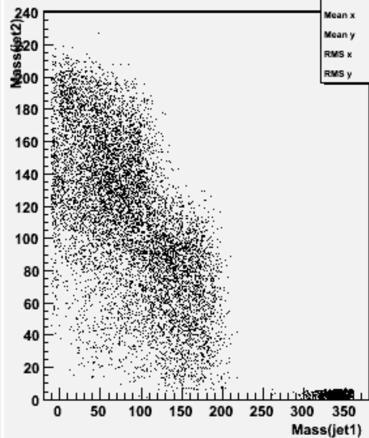
Jet mass for forced 2-jets : w103942 ae1_e1ssbb_o
