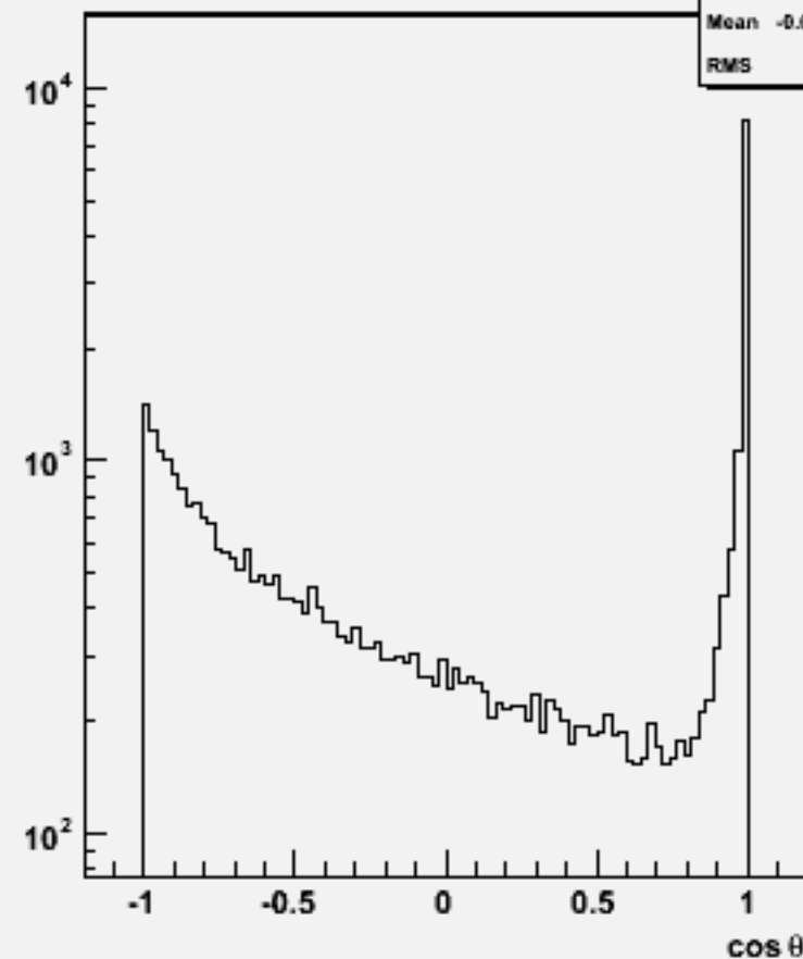
Jet cos \theta (All jets)w103942 ae1_e1ssbb_o
