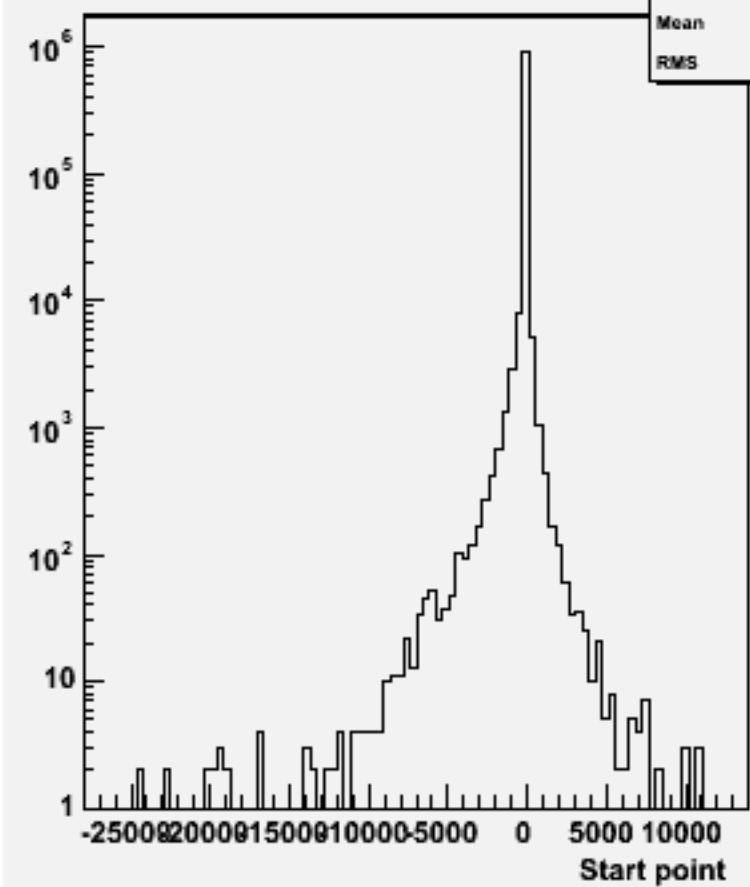
Start point Z : w103942 ae1_e1ssbb_o
