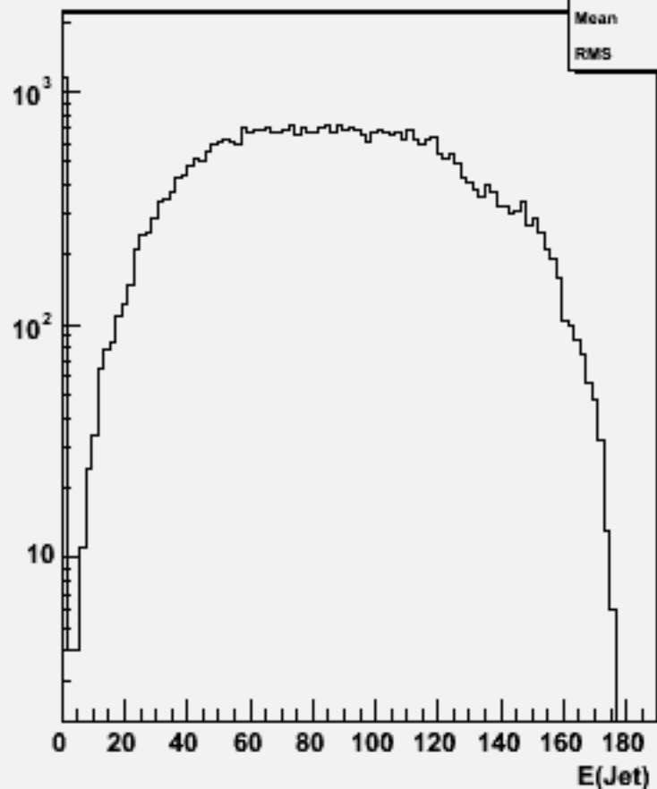
Jet energies(All jets)w103942 ae1_e1ssbb_o
