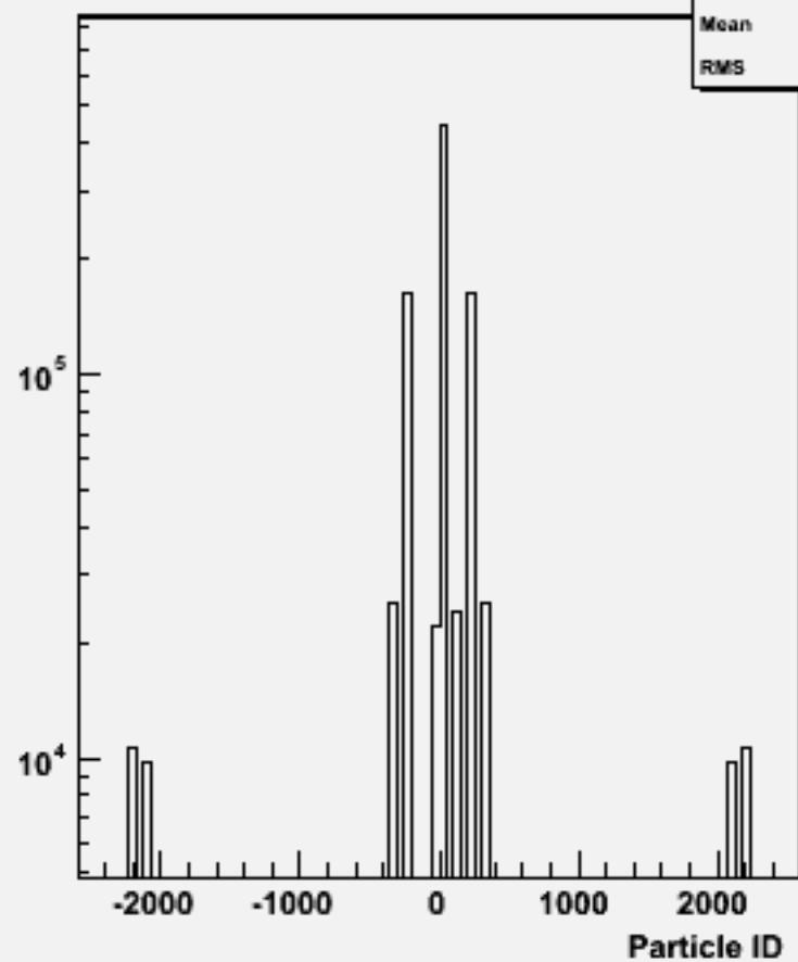
Particle ID : w103942 ae1_e1ssbb_o
