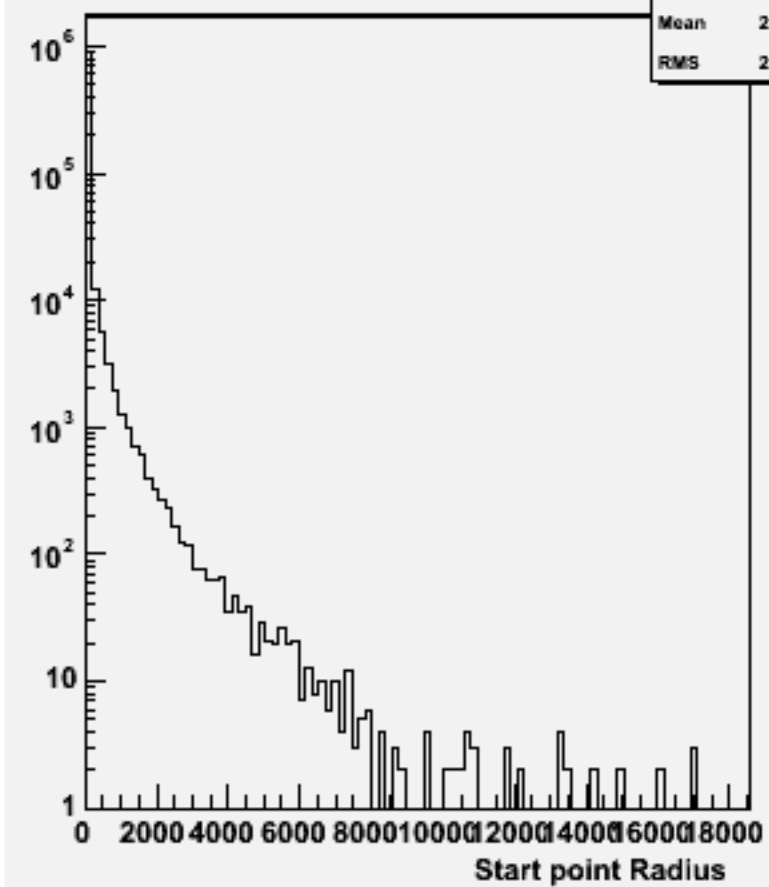
Start point R : w103942 ae1_e1ssbb_o
