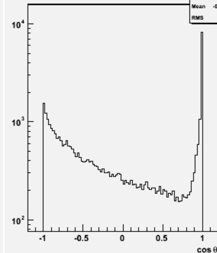
Jet cos \theta (All jets)w103938 ae1_e1ssss_o
