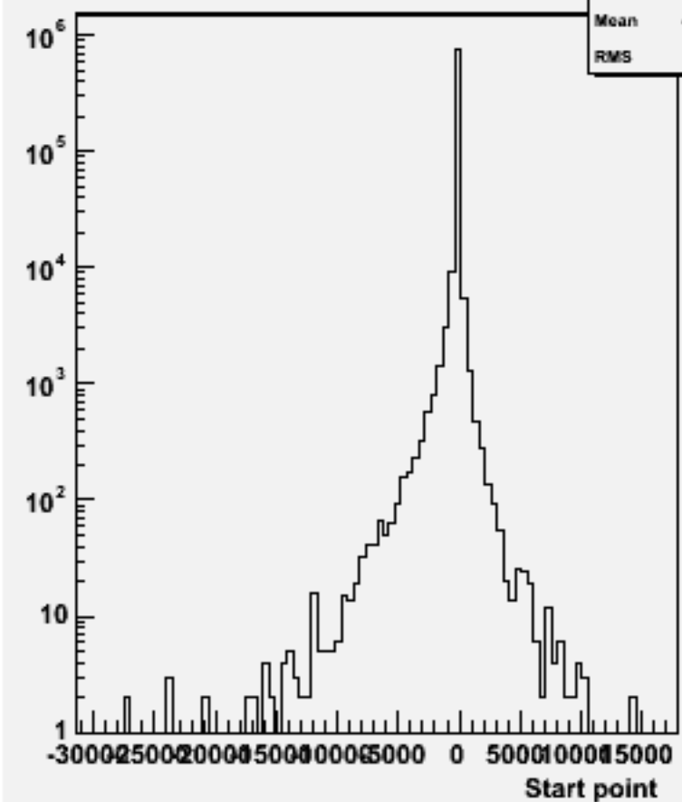
Start point Z : w103938 ae1_e1ssss_o
