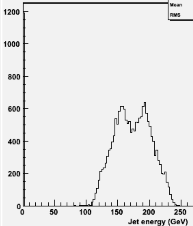
energy for 2-jets :w103938 ae1_e1ssss_o
