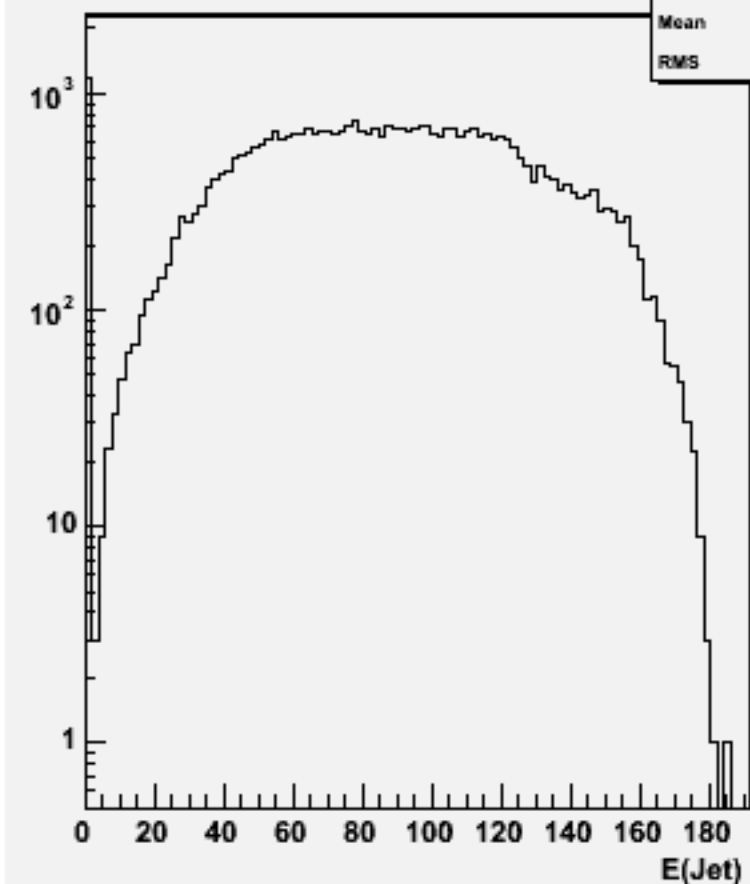
Jet energies(All jets)w103938 ae1_e1ssss_o
