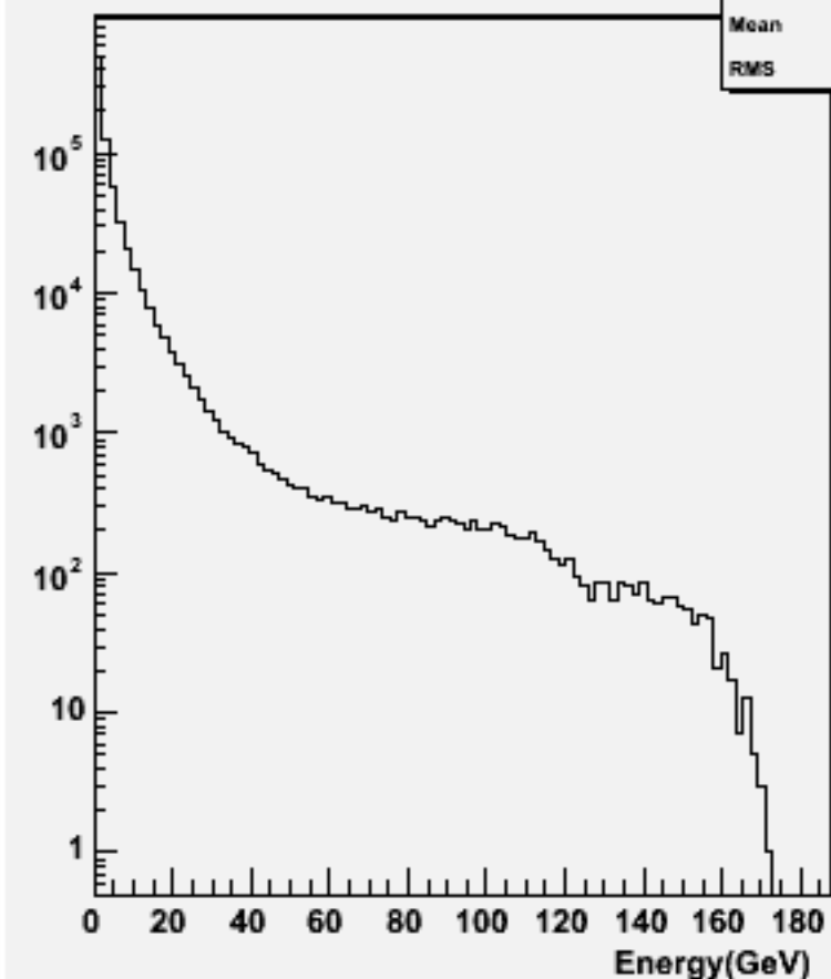
Particle Energy : w103938 ae1_e1ssss_o
