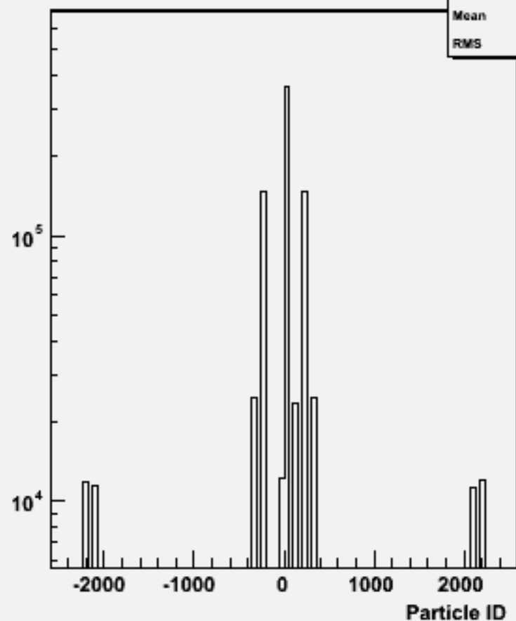
Particle ID : w103938 ae1_e1ssss_o
