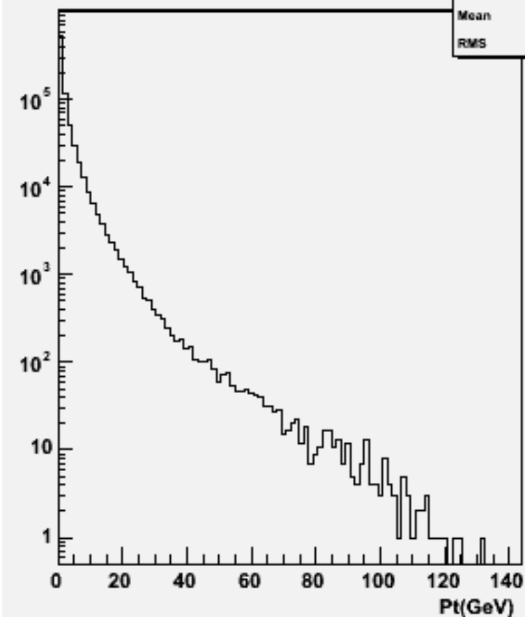
Particle Pt : w103938 ae1_e1ssss_o
