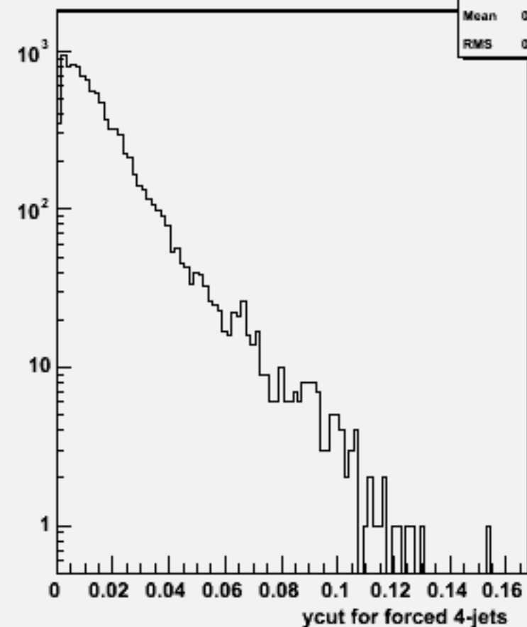
Ycut for 4-jets :w103938 ae1_e1ssss_o
