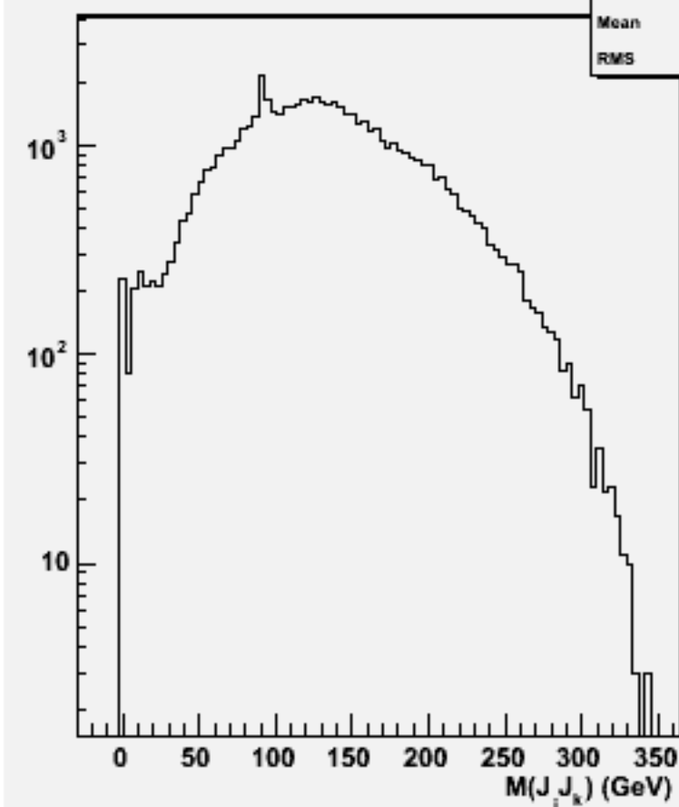
2jets mass(All comb)w103938 ae1_e1ssss_o
