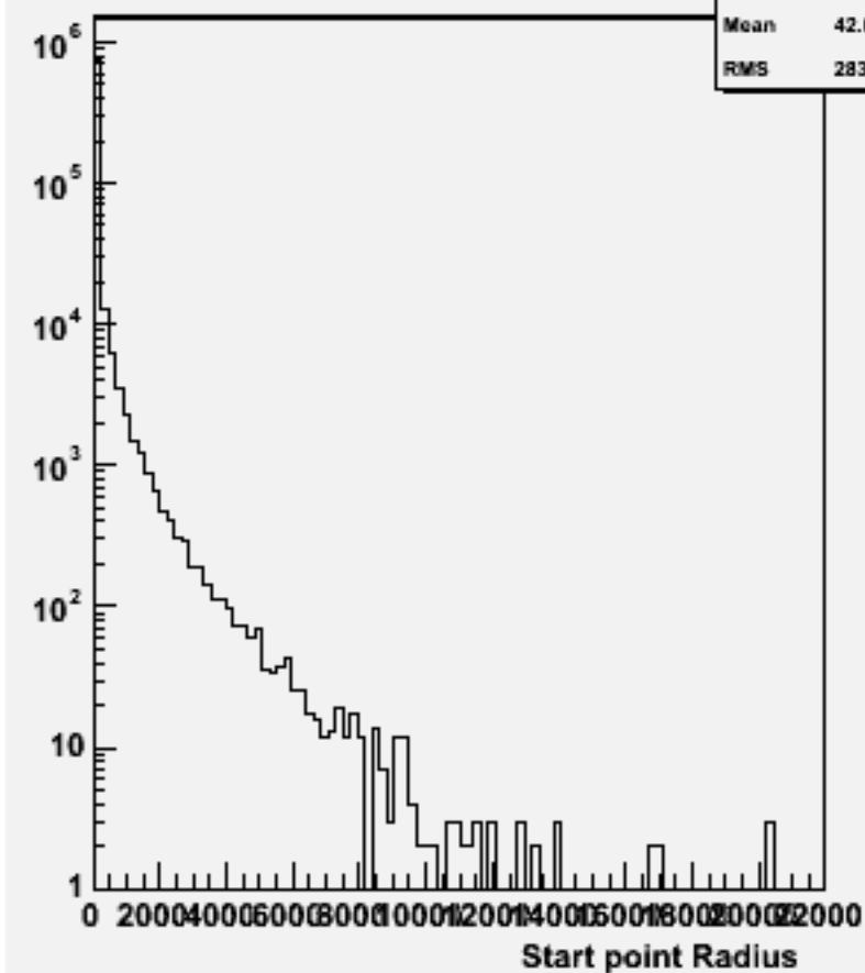
Start point R : w103938 ae1_e1ssss_o
