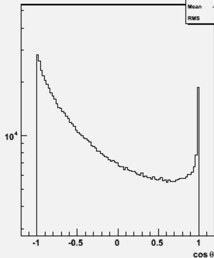
Particle cos \theta : w103938 ae1_e1ssss_o
