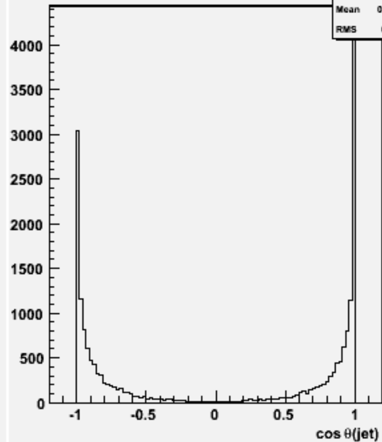
cos \theta for 2-jets :w103938 ae1_e1ssss_o
