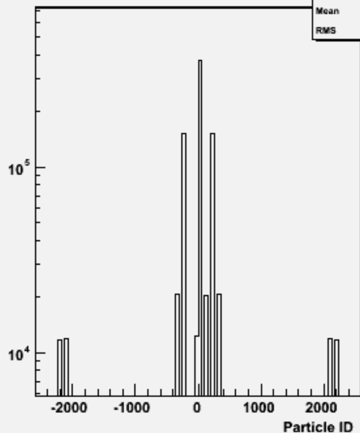
Particle ID : w103930 ae1_e1ddss_o
