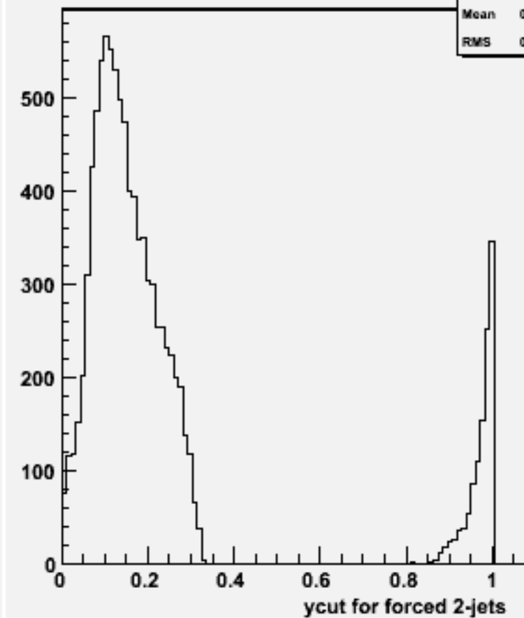
Ycut for 2-jets :w103930 ae1_e1ddss_o
