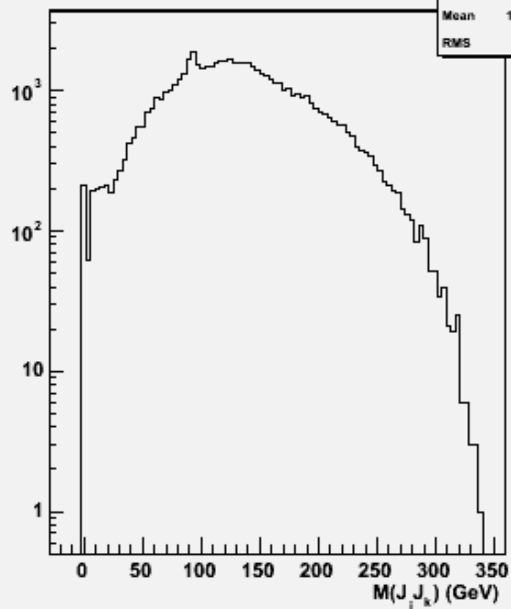
2jets mass(All comb)w103930 ae1_e1ddss_o
