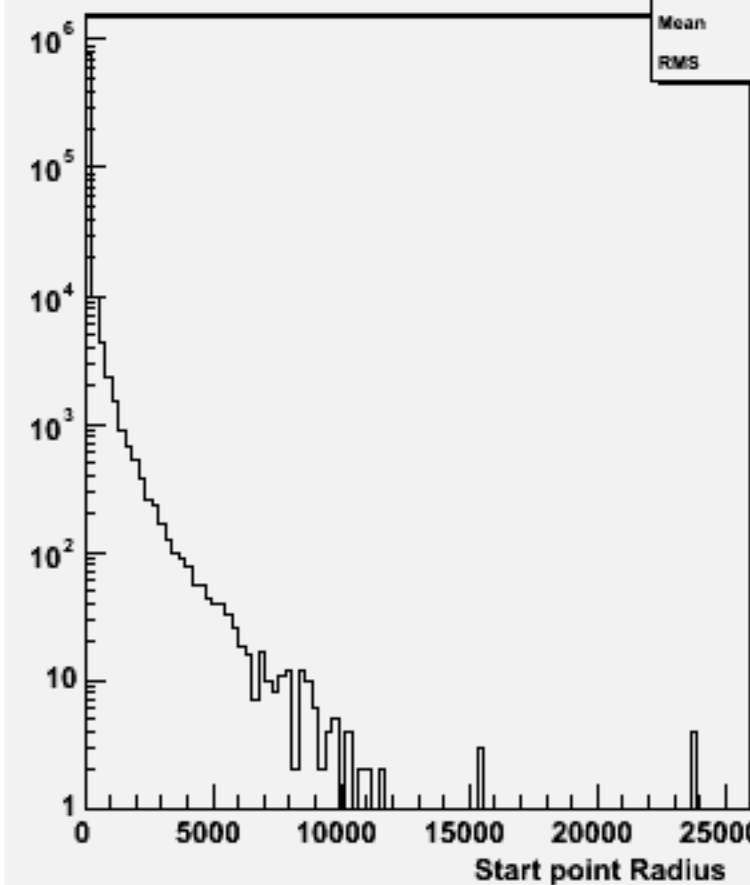
Start point R : w103930 ae1_e1ddss_o
