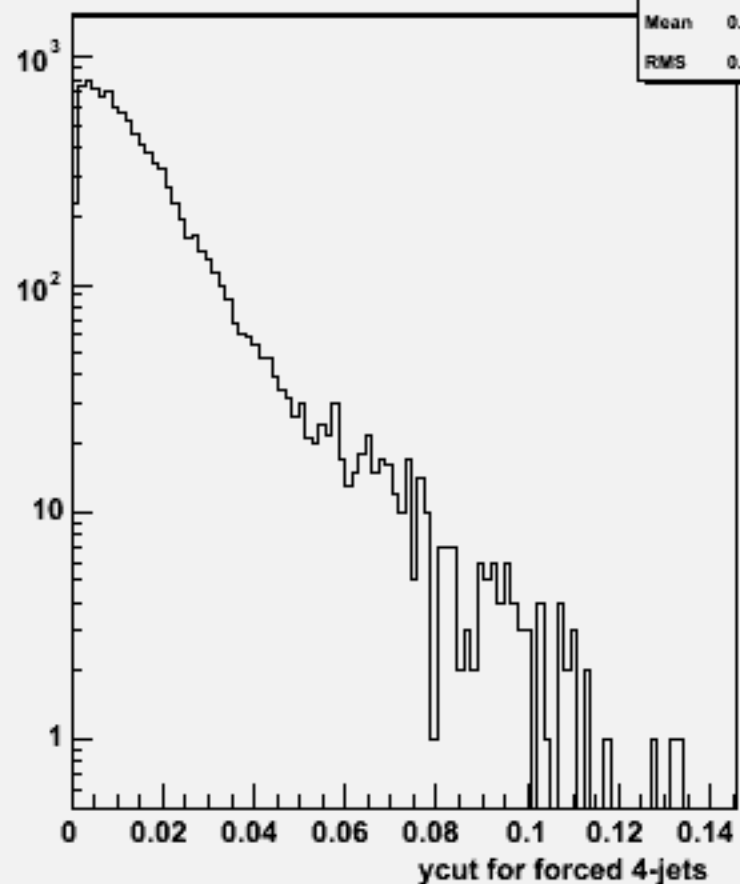
Ycut for 4-jets :w103930 ae1_e1ddss_o
