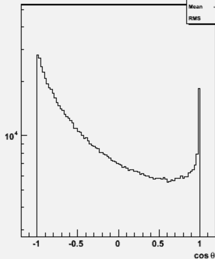
Particle cos \theta : w103930 ae1_e1ddss_o
