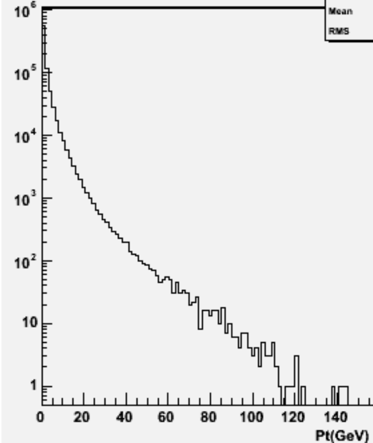
Particle Pt : w103930 ae1_e1ddss_o
