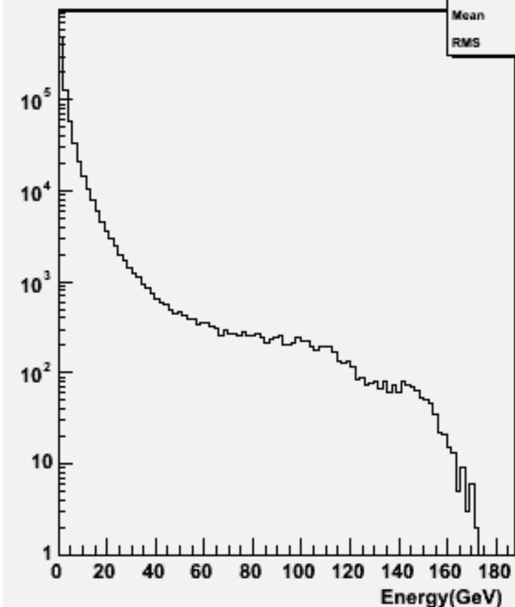
Particle Energy : w103930 ae1_e1ddss_o
