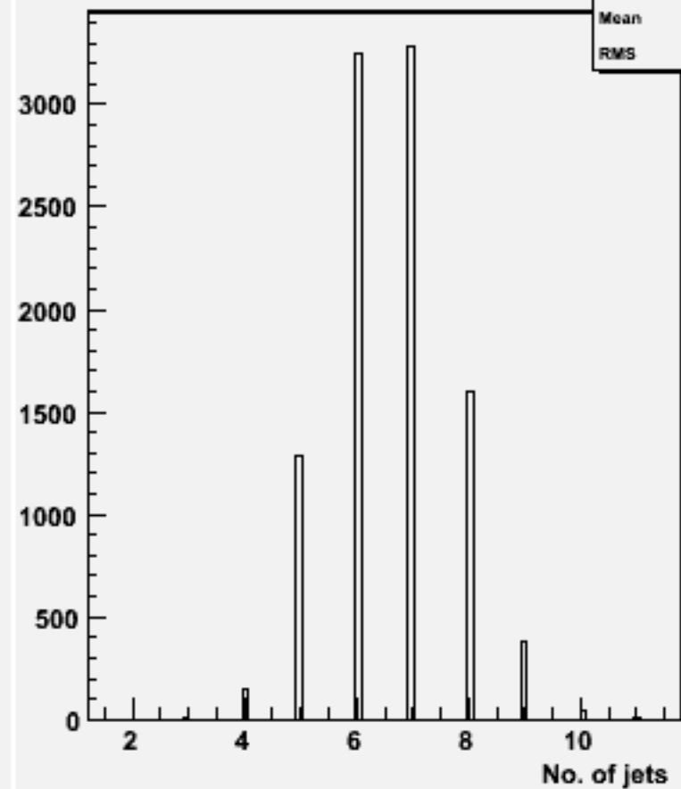
No. jets (ycut=0.001) : w103930 ae1_e1ddss_o
