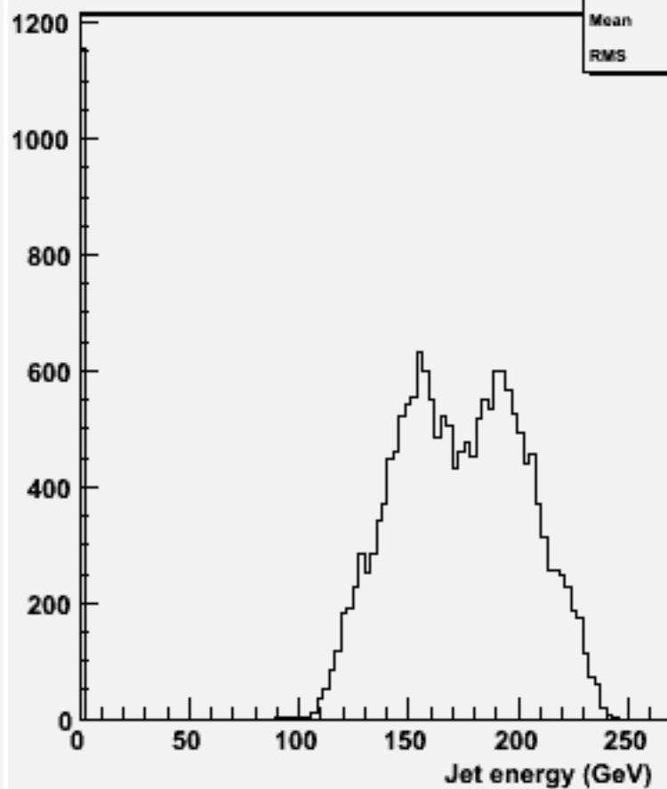
energy for 2-jets :w103930 ae1_e1ddss_o
