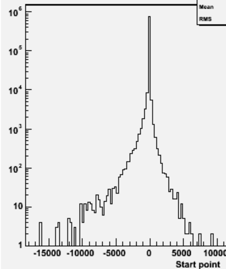
Start point Z : w103930 ae1_e1ddss_o
