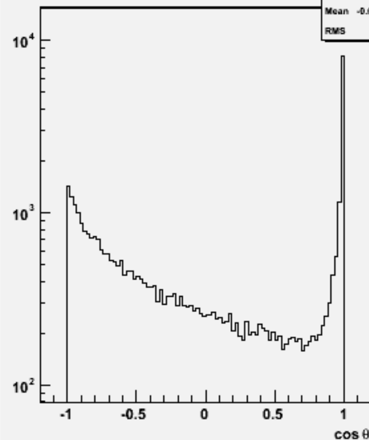
Jet cos \theta (All jets)w103930 ae1_e1ddss_o
