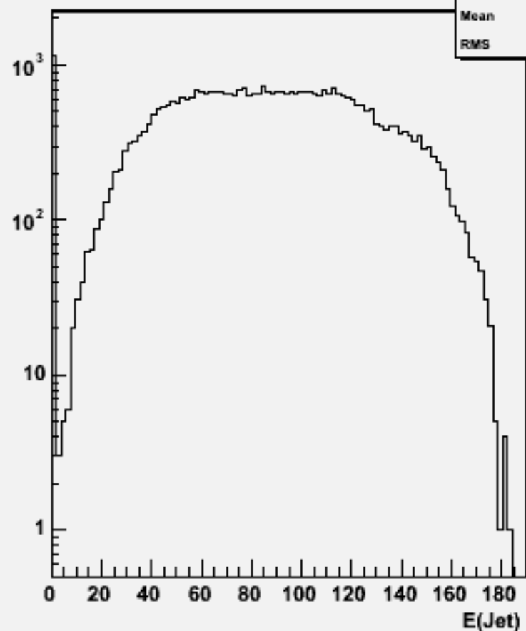
Jet energies(All jets)w103930 ae1_e1ddss_o
