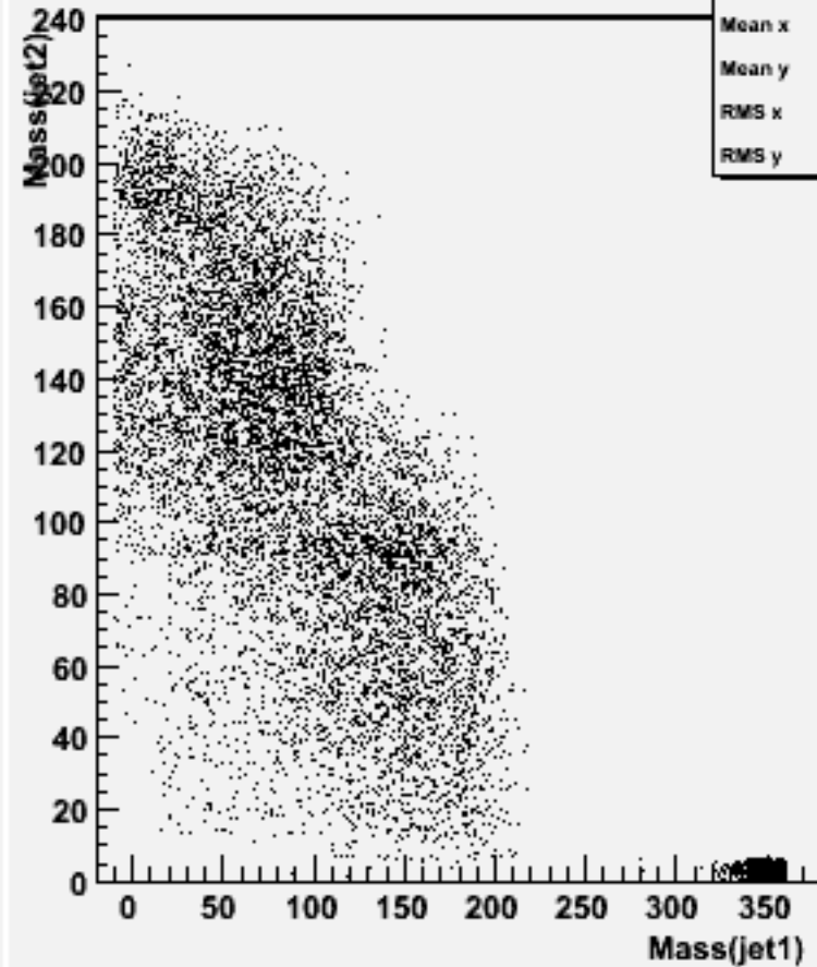
Jet mass for forced 2-jets : w103930 ae1_e1ddss_o
