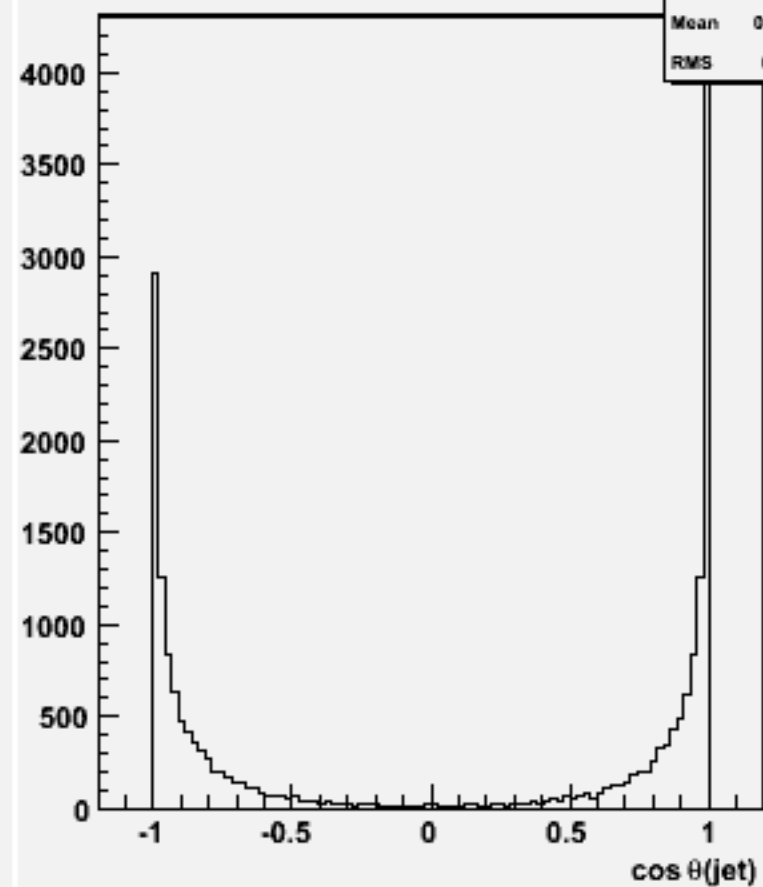
cos \theta for 2-jets :w103930 ae1_e1ddss_o
