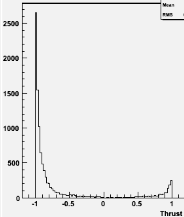
cos \Theta (thrust) w103930 ae1_e1ddss_o
