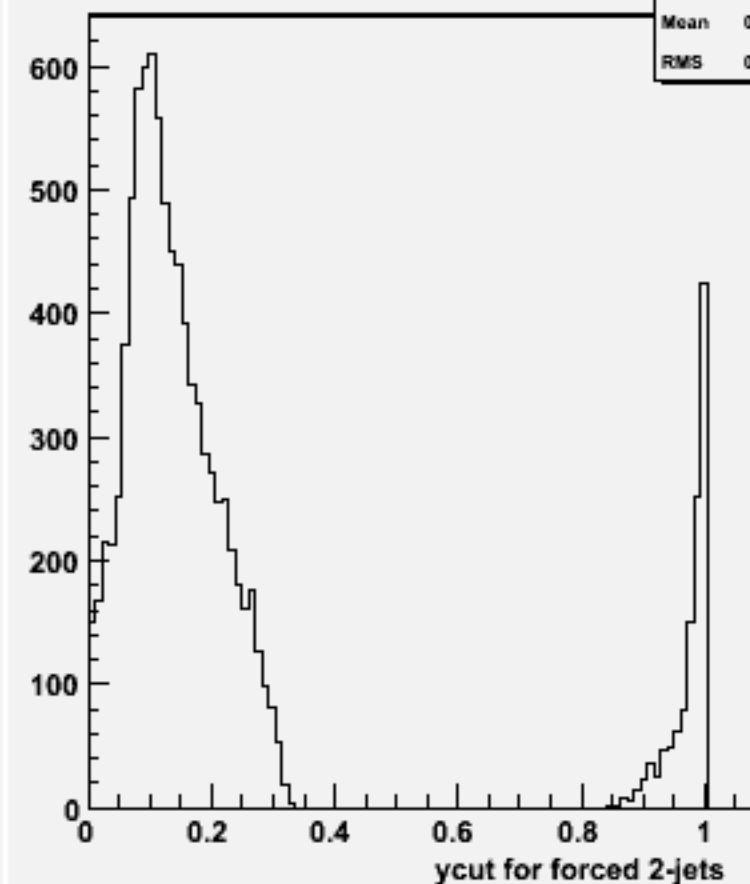
Ycut for 2-jets :w103928 ae1_e1ddss_o
