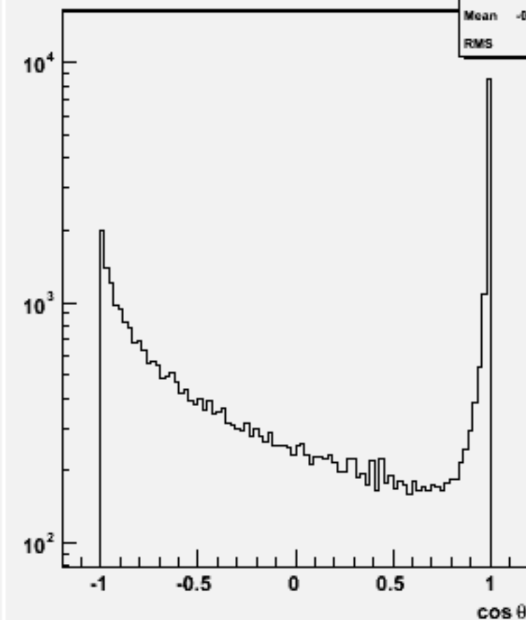
Jet cos \theta (All jets)w103928 ae1_e1ddss_o
