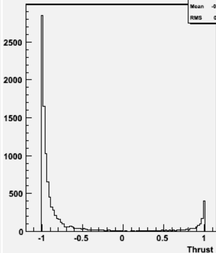
cos \Theta (thrust) w103928 ae1_e1ddss_o
