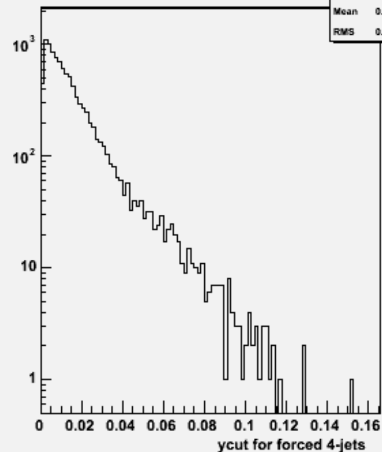
Ycut for 4-jets :w103928 ae1_e1ddss_o
