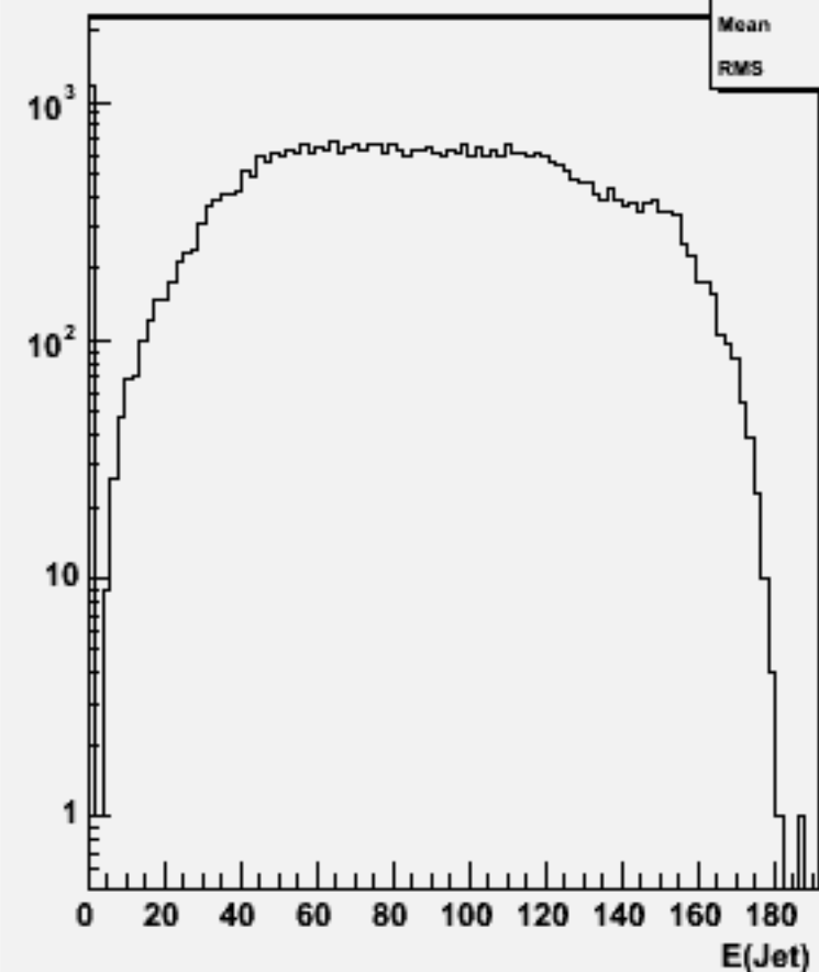
Jet energies(All jets)w103928 ae1_e1ddss_o
