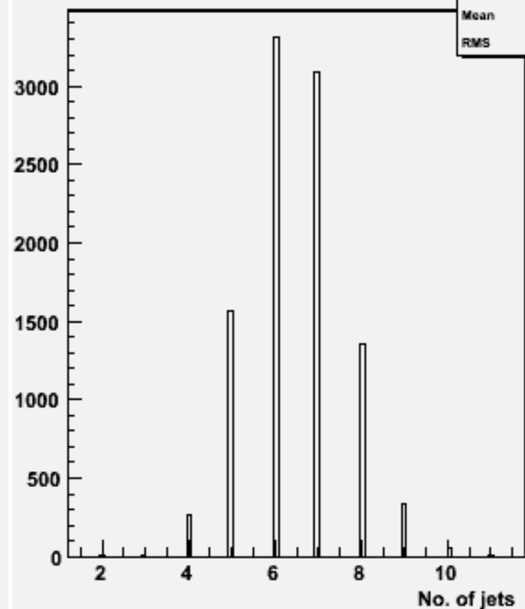
No. jets (ycut=0.001) : w103928 ae1_e1ddss_o
