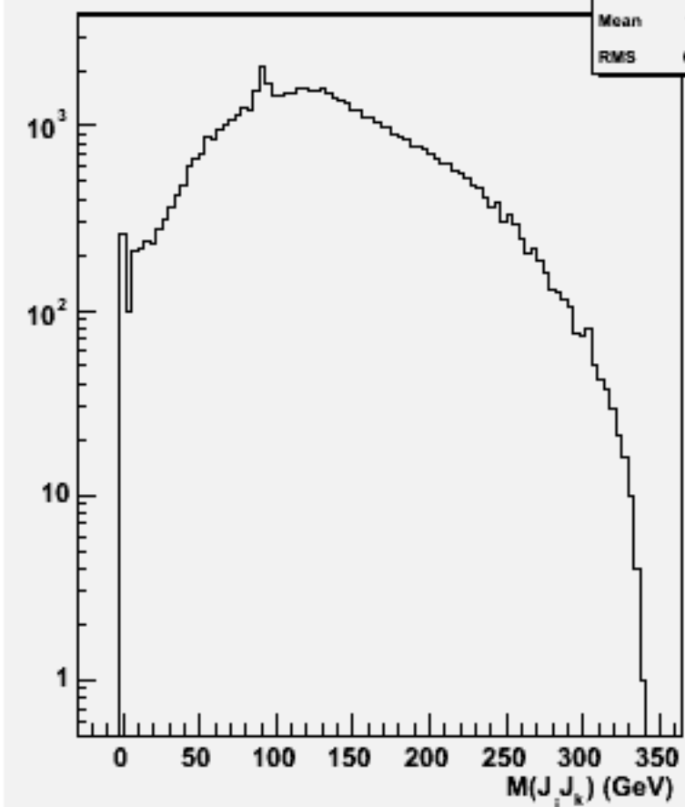
2jets mass(All comb)w103928 ae1_e1ddss_o
