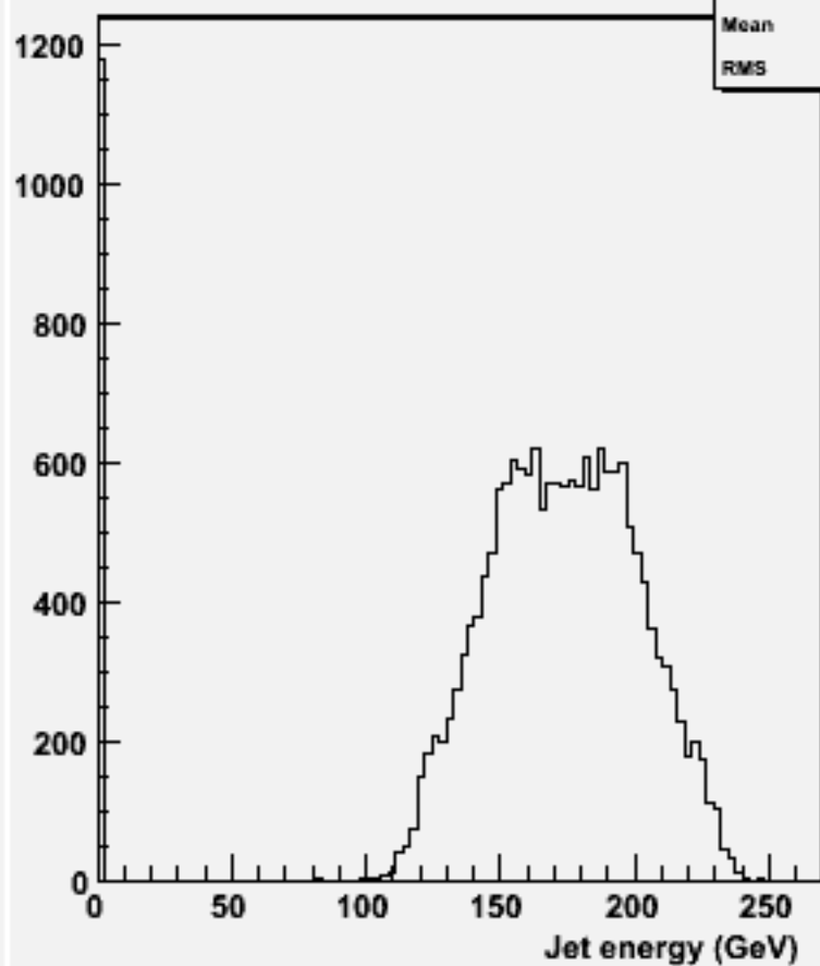
energy for 2-jets :w103928 ae1_e1ddss_o
