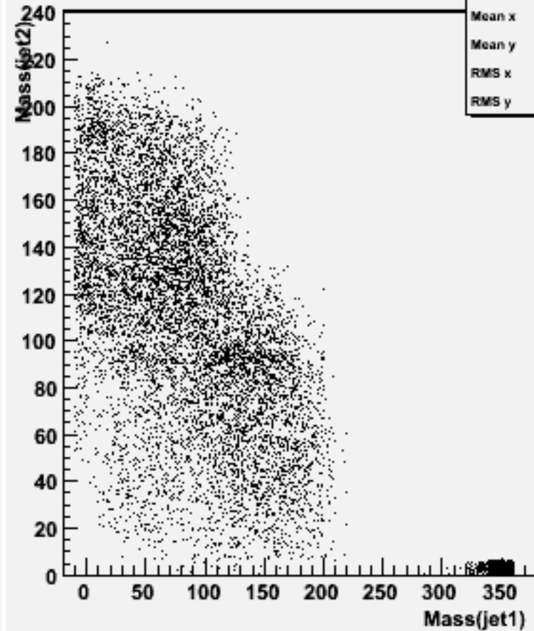
Jet mass for forced 2-jets : w103928 ae1_e1ddss_o
