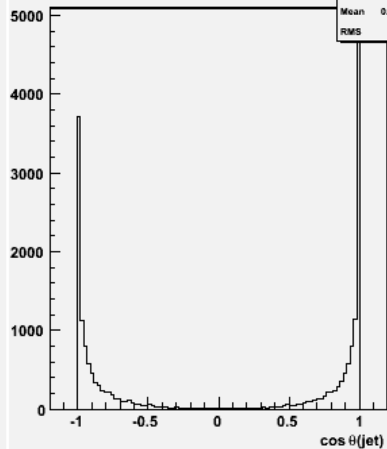
cos \theta for 2-jets :w103928 ae1_e1ddss_o
