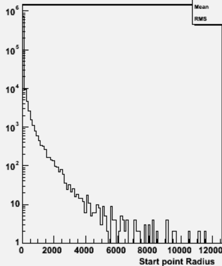
Start point R : w103924 ae1_e1dddd_o
