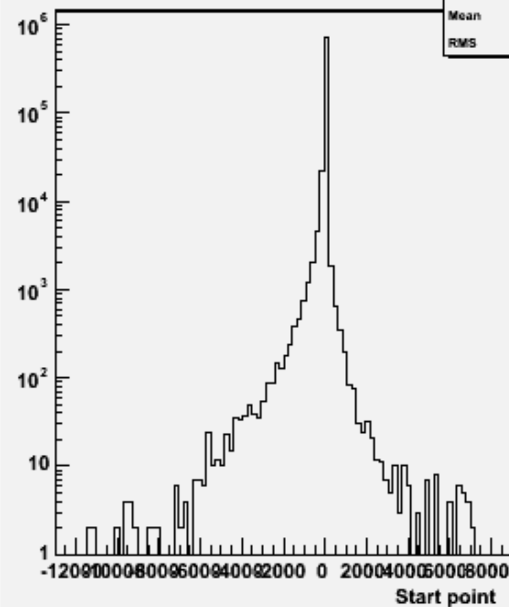
Start point Z : w103924 ae1_e1dddd_o
