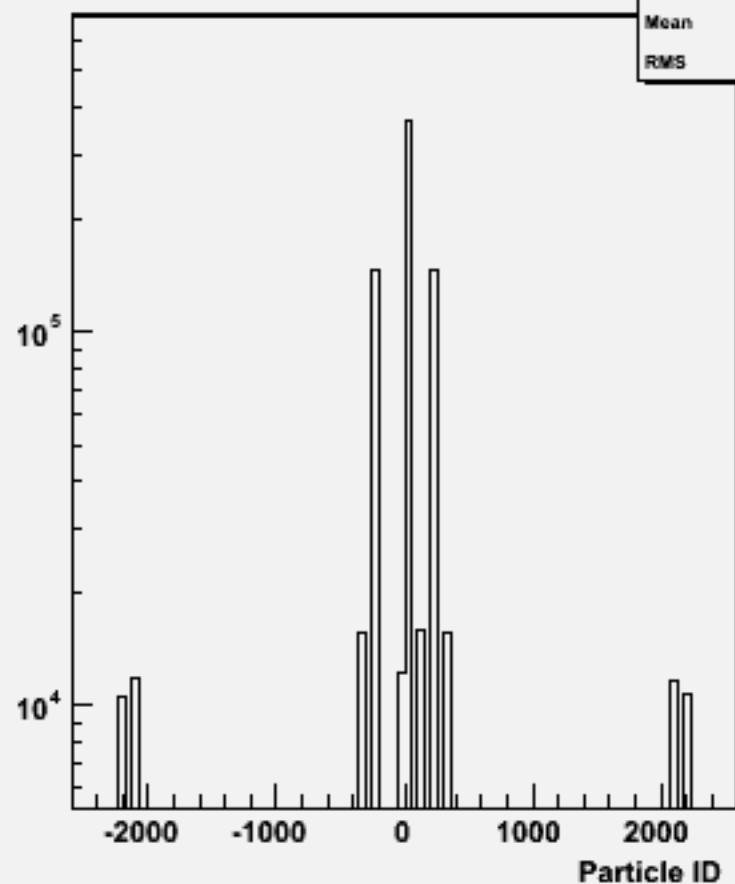
Particle ID : w103924 ae1_e1dddd_o
