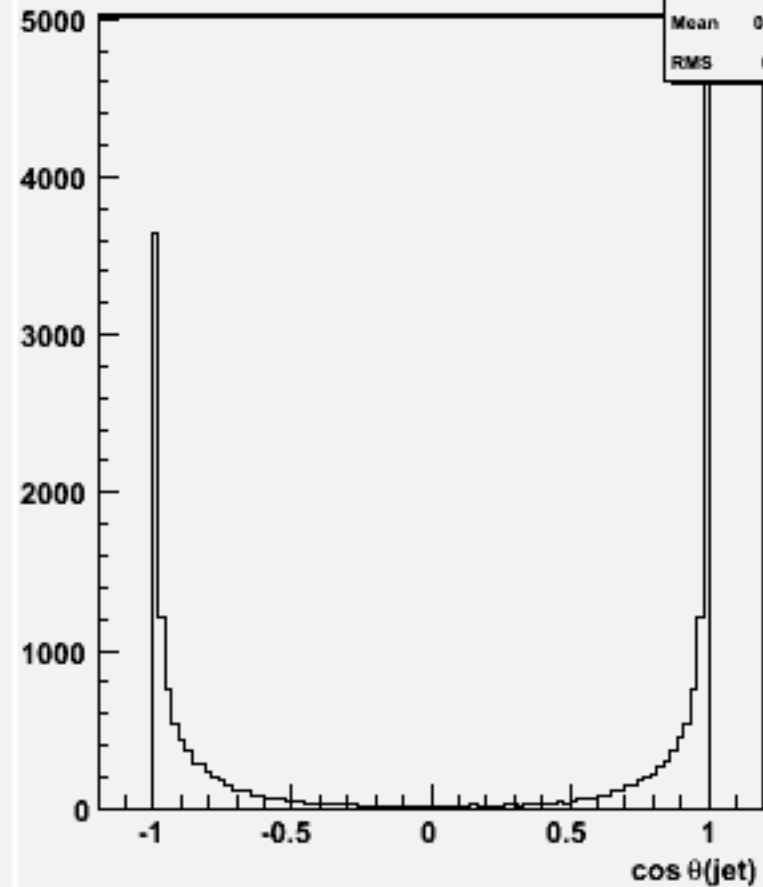
cos \theta for 2-jets :w103924 ae1_e1dddd_o
