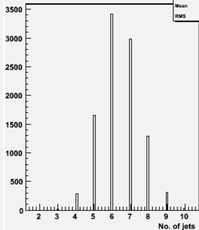
No. jets (ycut=0.001) : w103924 ae1_e1dddd_o
