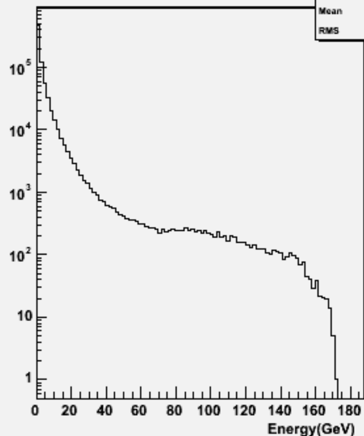
Particle Energy : w103924 ae1_e1dddd_o
