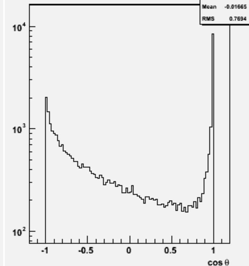
Jet cos \theta (All jets)w103924 ae1_e1dddd_o
