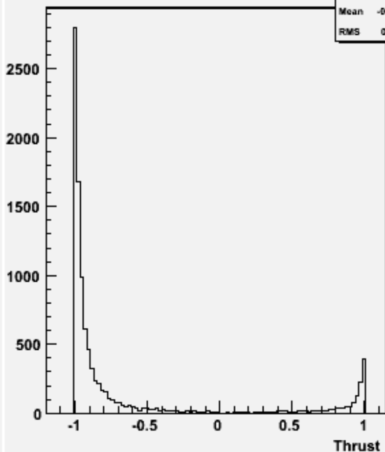
cos \Theta (thrust) w103924 ae1_e1dddd_o
