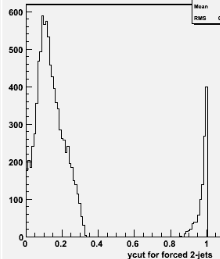
Ycut for 2-jets :w103924 ae1_e1dddd_o
