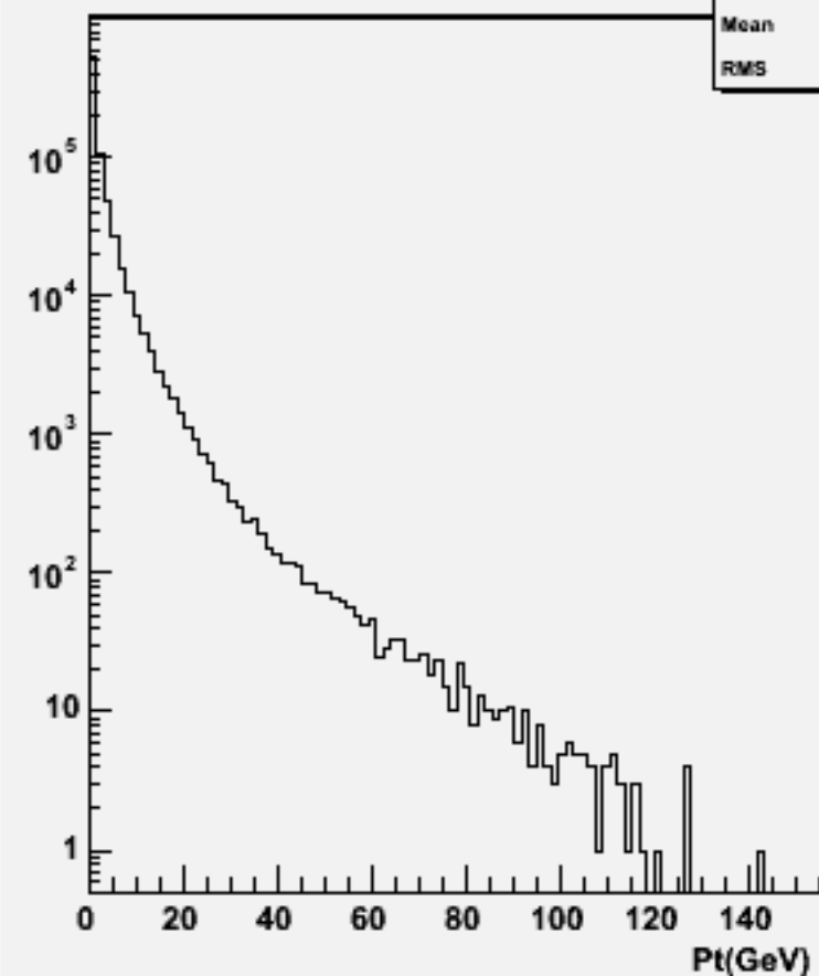
Particle Pt : w103924 ae1_e1dddd_o
