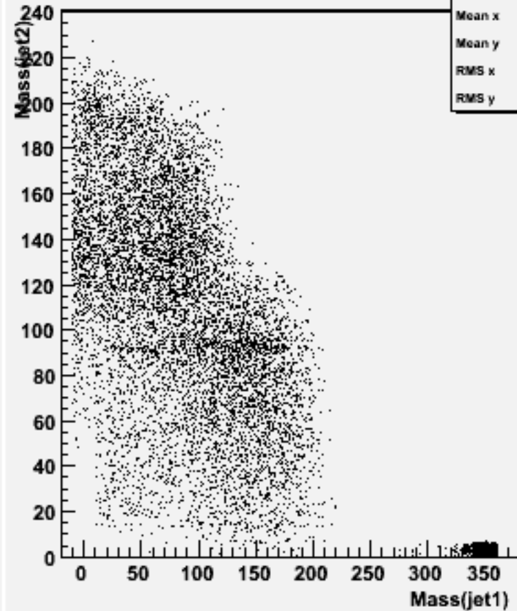
Jet mass for forced 2-jets : w103924 ae1_e1dddd_o
