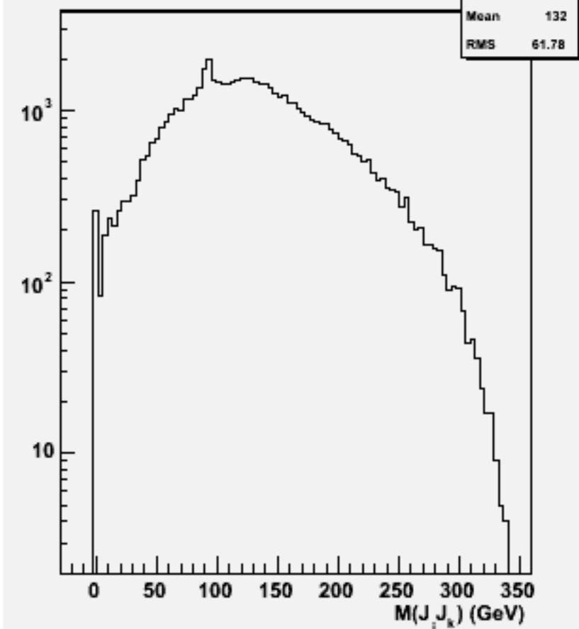
2jets mass(All comb)w103924 ae1_e1dddd_o
