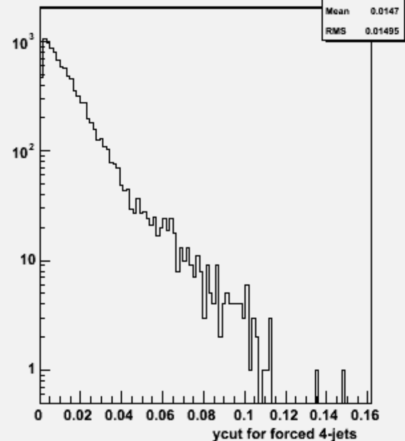
Ycut for 4-jets :w103924 ae1_e1dddd_o
