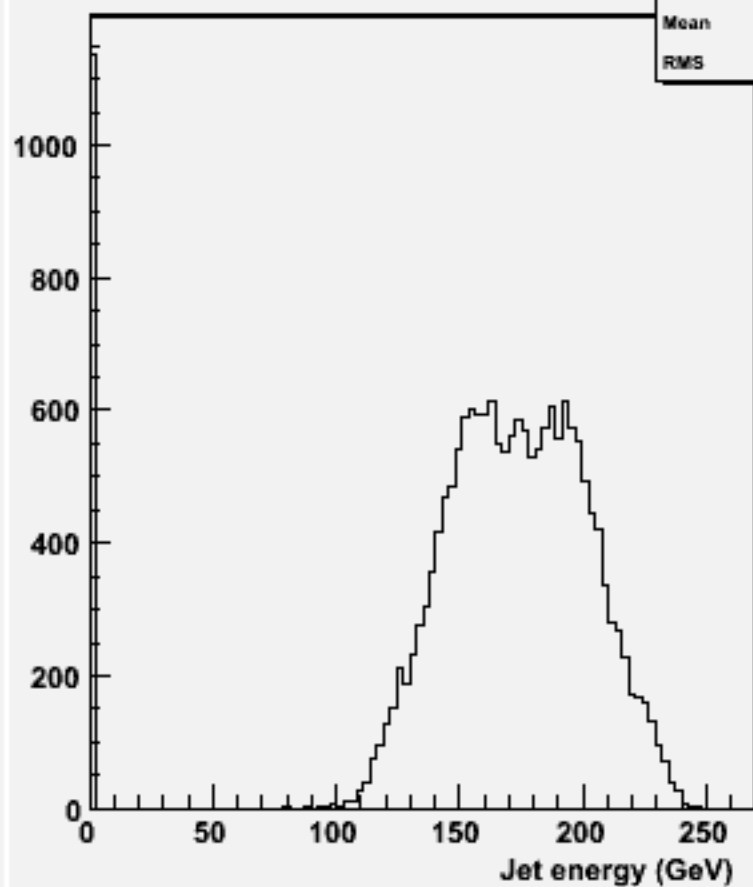
energy for 2-jets :w103924 ae1_e1dddd_o
