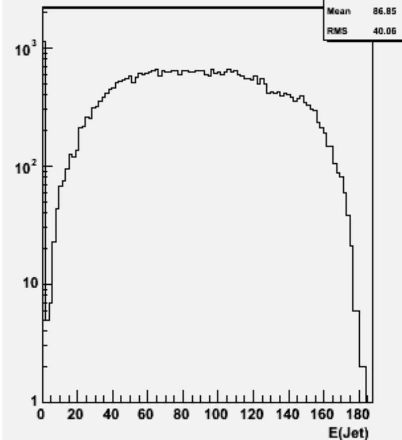
Jet energies(All jets)w103924 ae1_e1dddd_o
