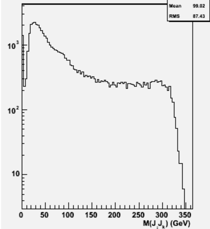
2jets mass(All comb)w103923 ae1_e1e3e3bb_o
