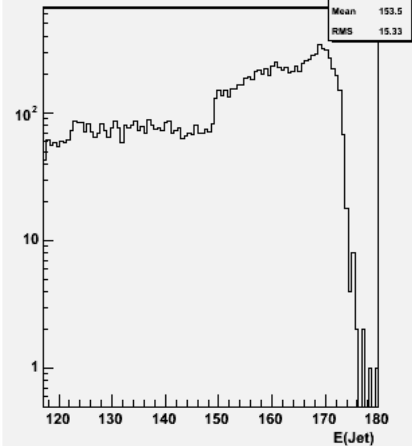
Jet energies(All jets)w103923 ae1_e1e3e3bb_o
