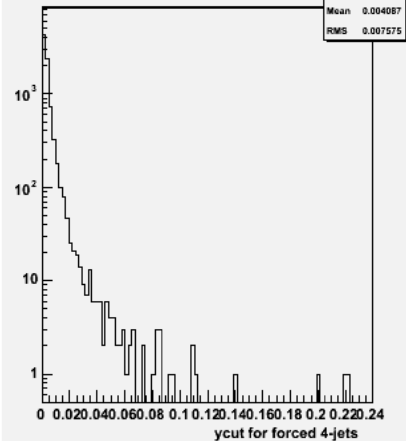
Ycut for 4-jets :w103923 ae1_e1e3e3bb_o
