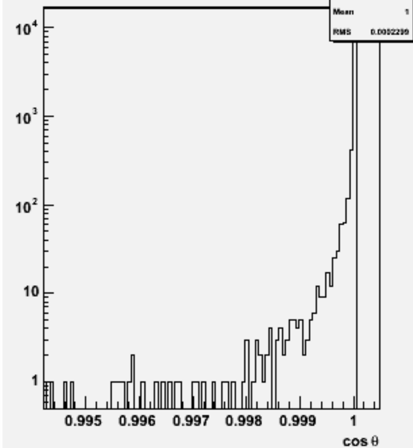
Jet cos \theta (All jets)w103923 ae1_e1e3e3bb_o
