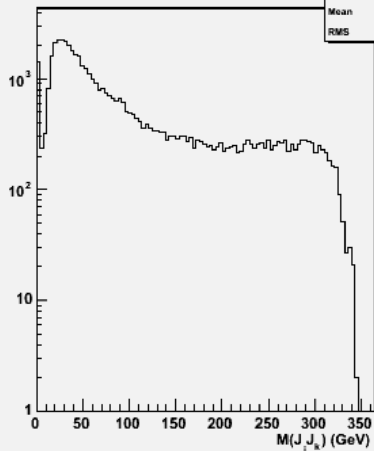
2jets mass(All comb)w103921 ae1_e1e3e3bb_o
