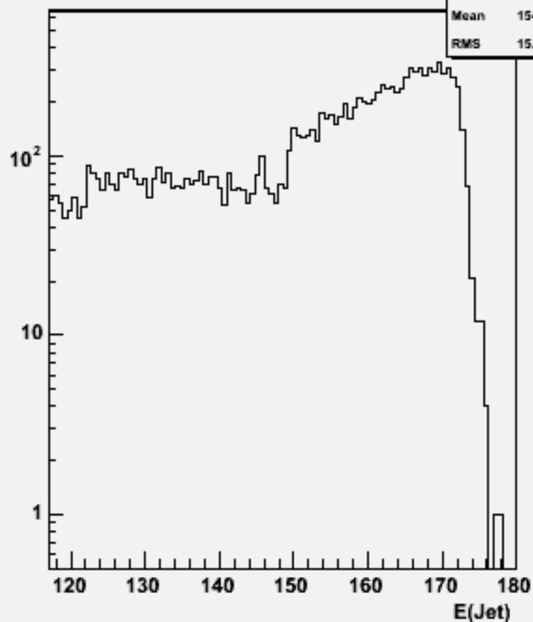
Jet energies(All jets)w103921 ae1_e1e3e3bb_o
