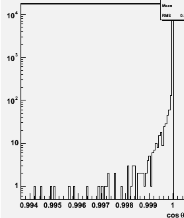
Jet cos \theta (All jets)w103921 ae1_e1e3e3bb_o
