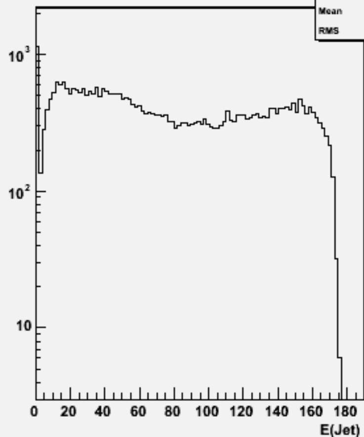
Jet energies(All jets)w103920 ae1_e1e3e3bb_o
