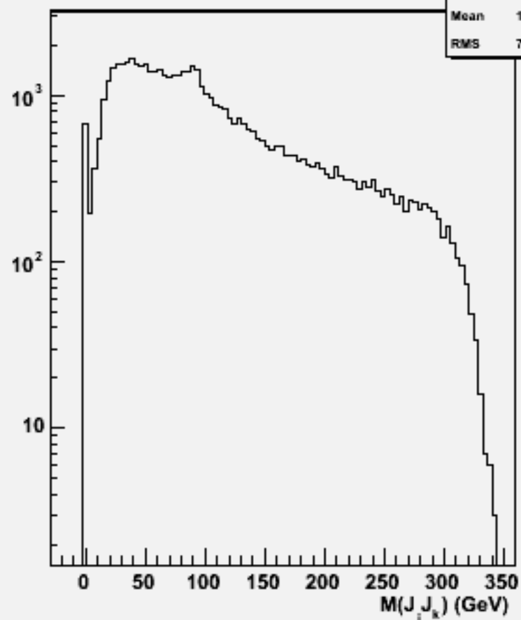
2jets mass(All comb)w103920 ae1_e1e3e3bb_o
