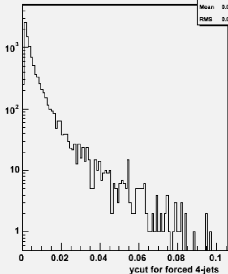
Ycut for 4-jets :w103920 ae1_e1e3e3bb_o
