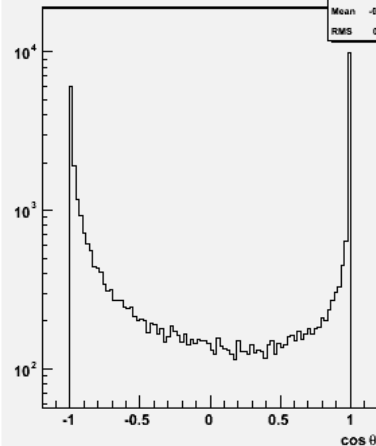
Jet cos \theta (All jets)w103920 ae1_e1e3e3bb_o
