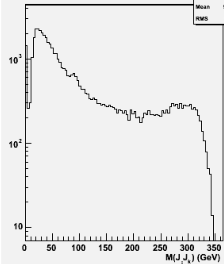
2jets mass(All comb)w103919 ae1_e1e3e3ss_o
