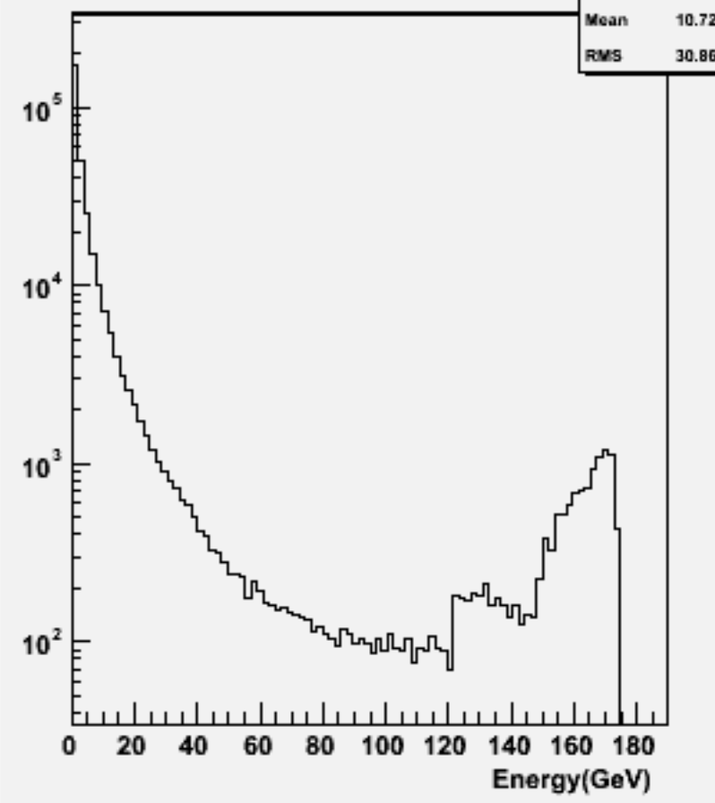
Start point R : w103919 ae1_e1e3e3ss_o
