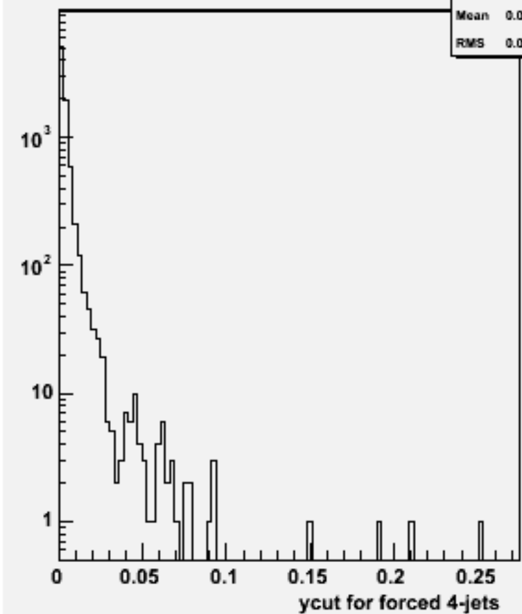
Ycut for 4-jets :w103919 ae1_e1e3e3ss_o
