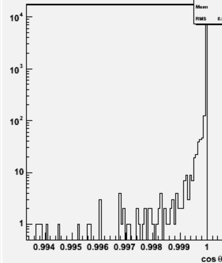
Jet cos \theta (All jets)w103919 ae1_e1e3e3ss_o
