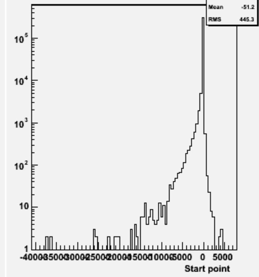
Start point Z : w103919 ae1_e1e3e3ss_o
