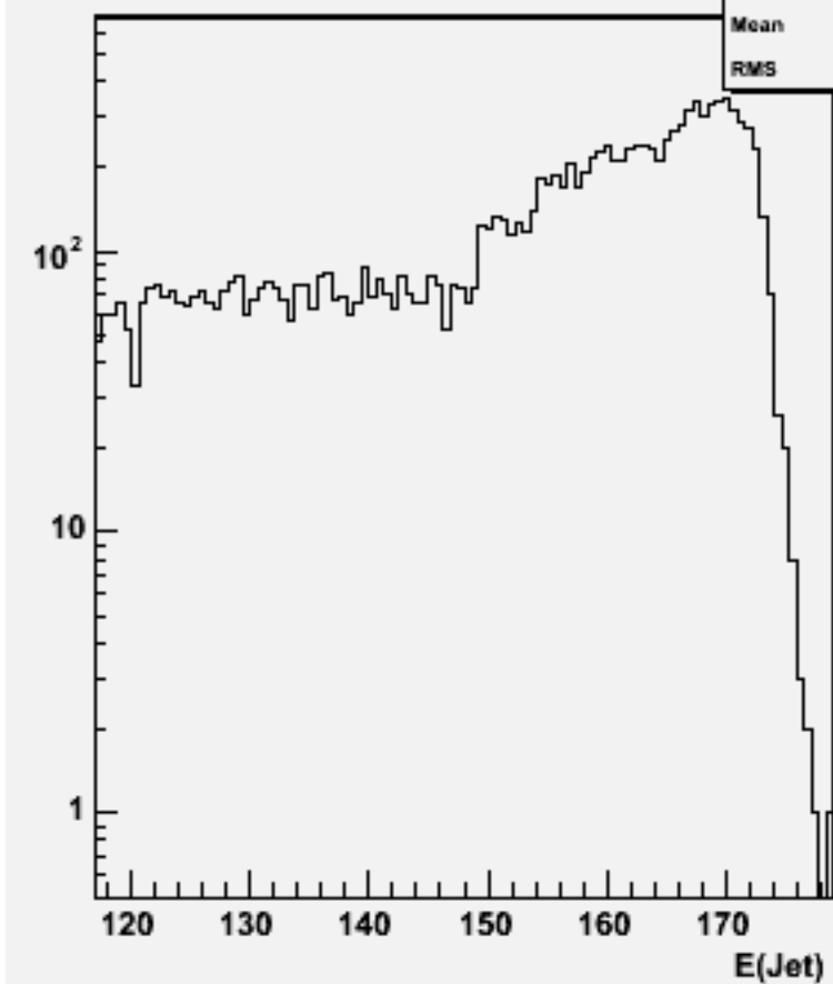
Jet energies(All jets)w103919 ae1_e1e3e3ss_o
