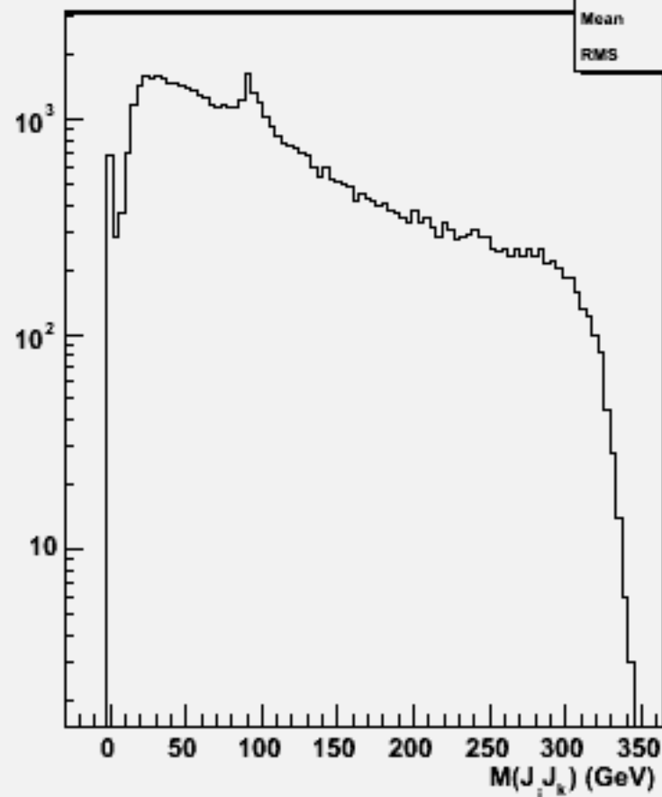
2jets mass(All comb)w103918 ae1_e1e3e3ss_o
