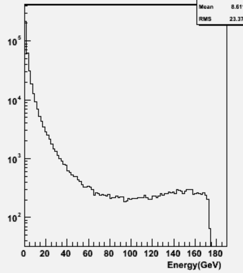
Start point R : w103918 ae1_e1e3e3ss_o
