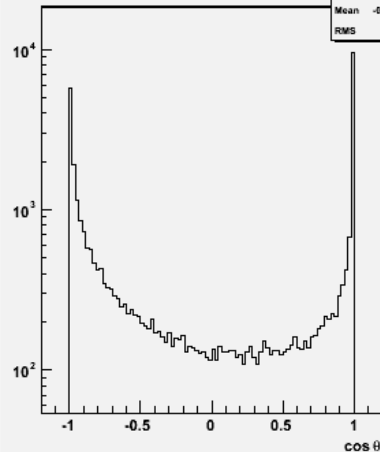
Jet cos \theta (All jets)w103918 ae1_e1e3e3ss_o
