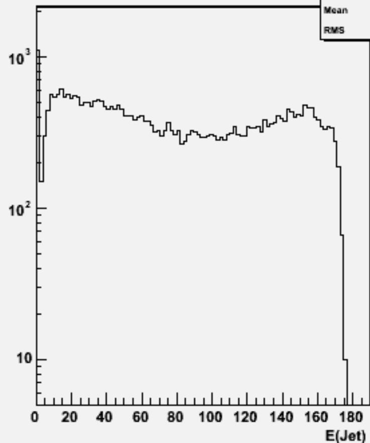
Jet energies(All jets)w103918 ae1_e1e3e3ss_o
