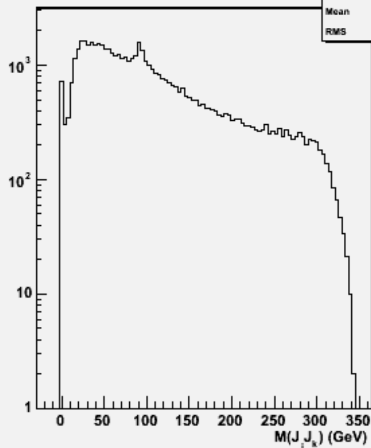
2jets mass(All comb)w103914 ae1_e1e3e3dd_o
