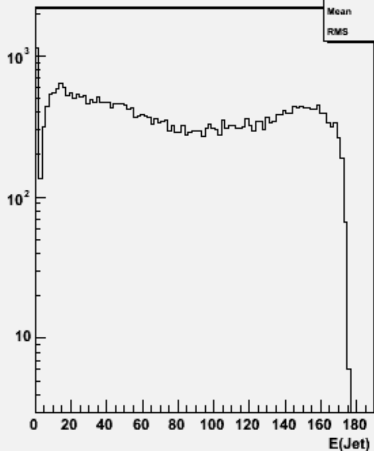
Jet energies(All jets)w103914 ae1_e1e3e3dd_o
