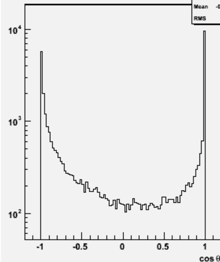
Jet cos \theta (All jets)w103914 ae1_e1e3e3dd_o
