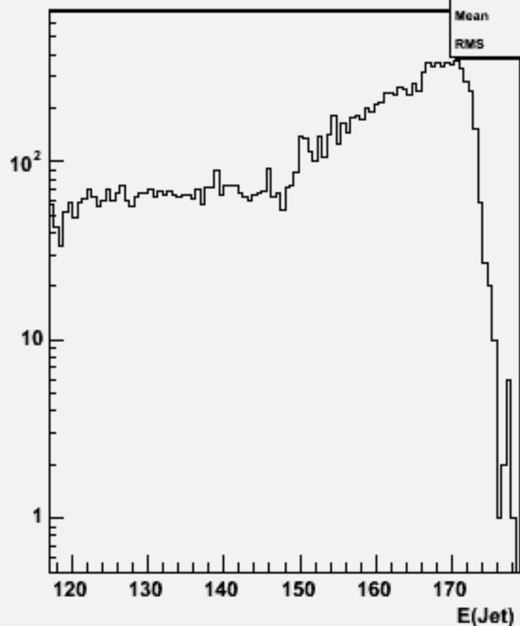
Jet energies(All jets)w103913 ae1_e1e3e3dd_o
