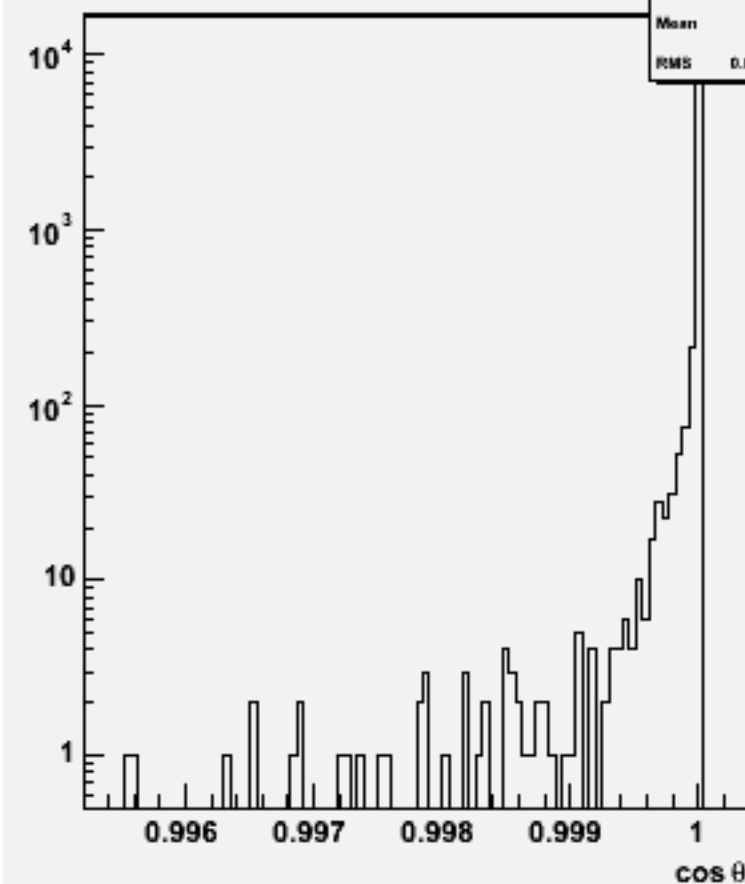
Jet cos \theta (All jets)w103913 ae1_e1e3e3dd_o
