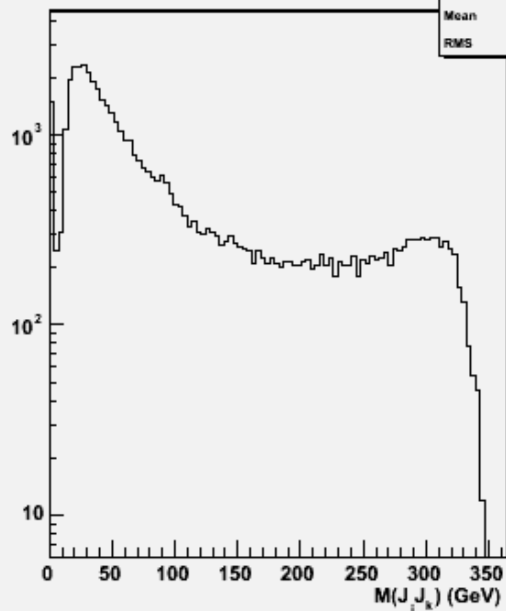
2jets mass(All comb)w103913 ae1_e1e3e3dd_o
