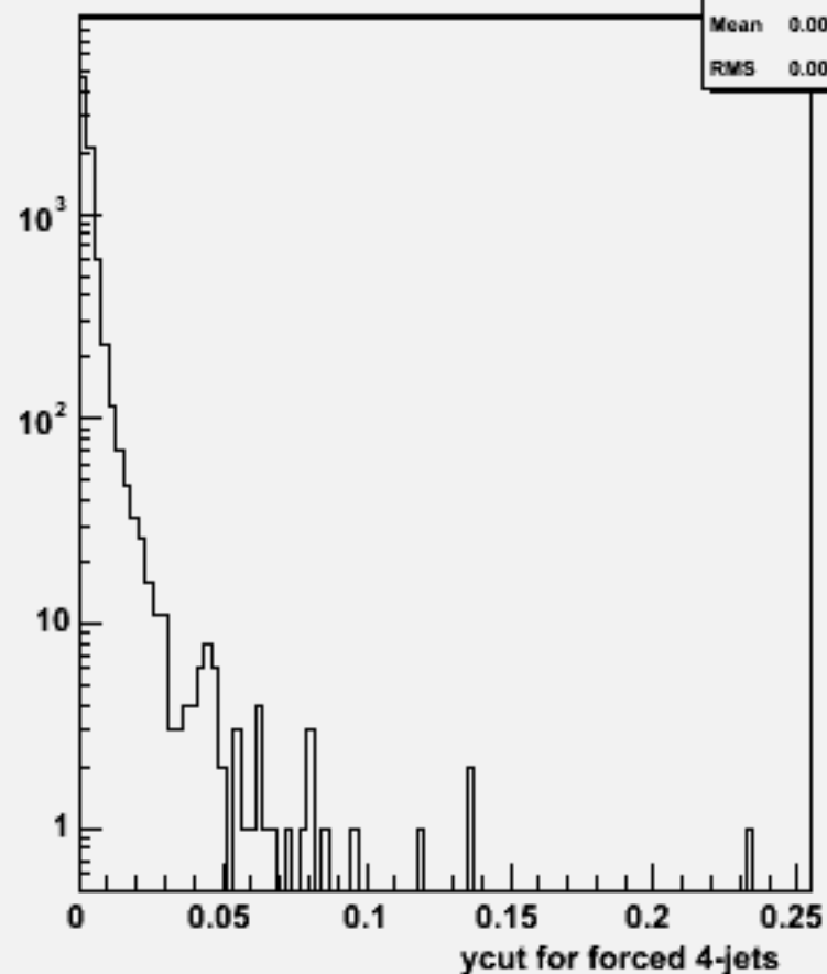
Ycut for 4-jets :w103913 ae1_e1e3e3dd_o
