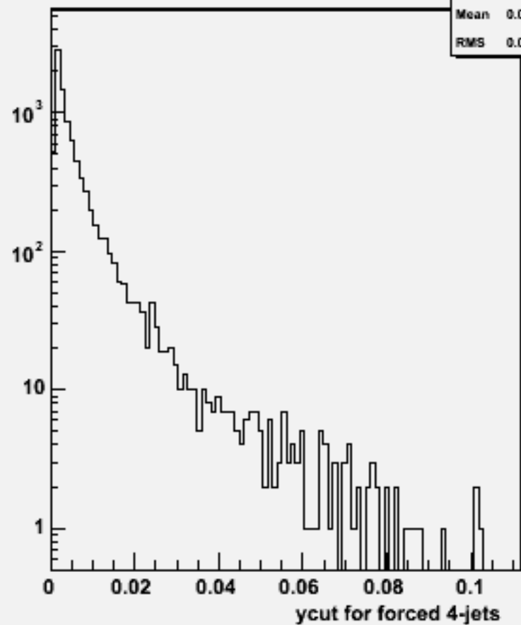
Ycut for 4-jets :w103912 ae1_e1e3e3dd_o
