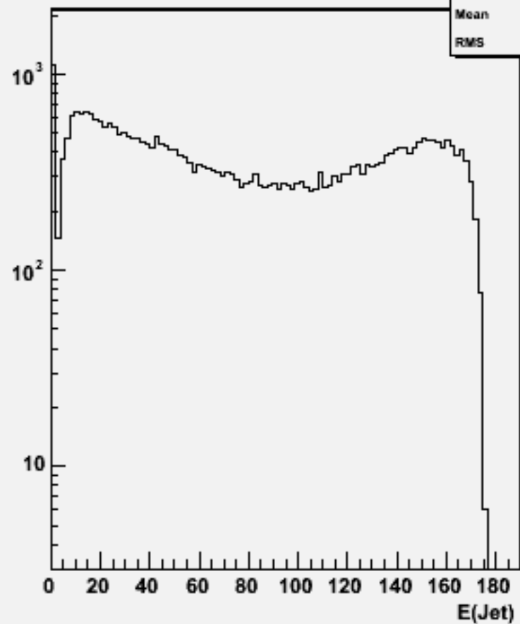
Jet energies(All jets)w103912 ae1_e1e3e3dd_o
