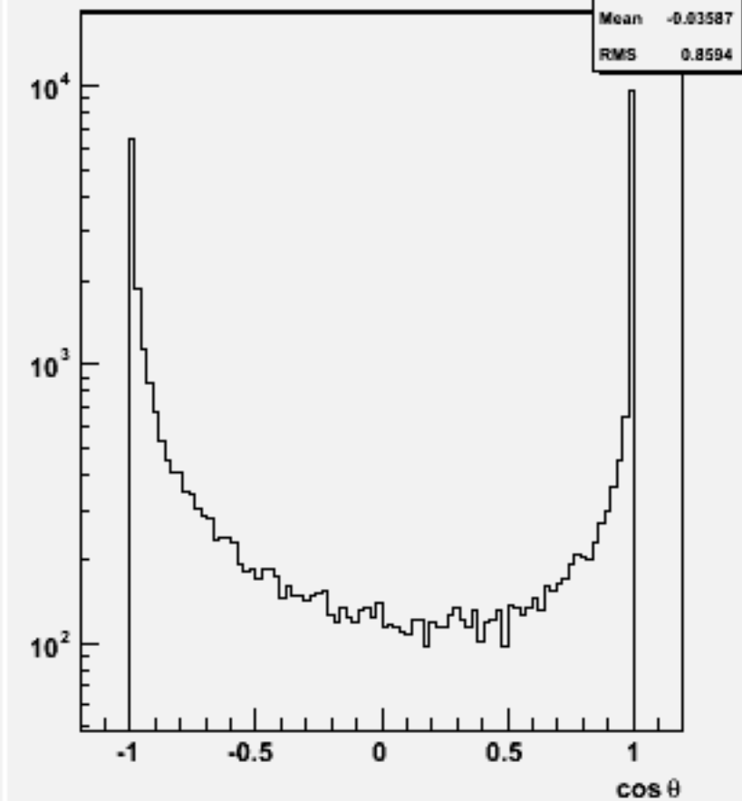
Jet cos theta (All jets)w103912 ae1_e1e3e3dd_o
