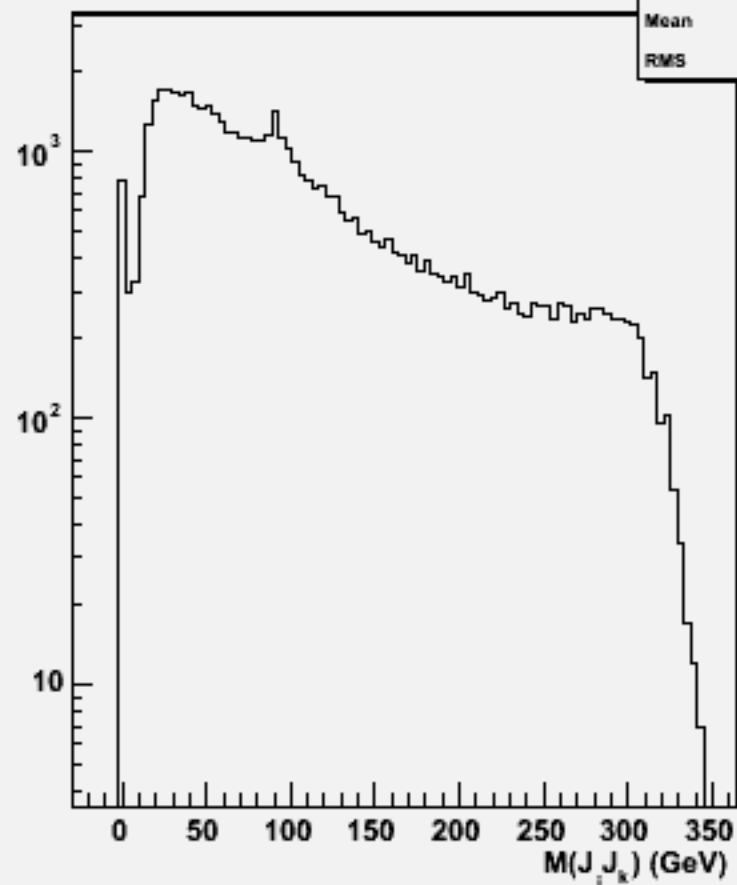
2jets mass(All comb)w103912 ae1_e1e3e3dd_o
