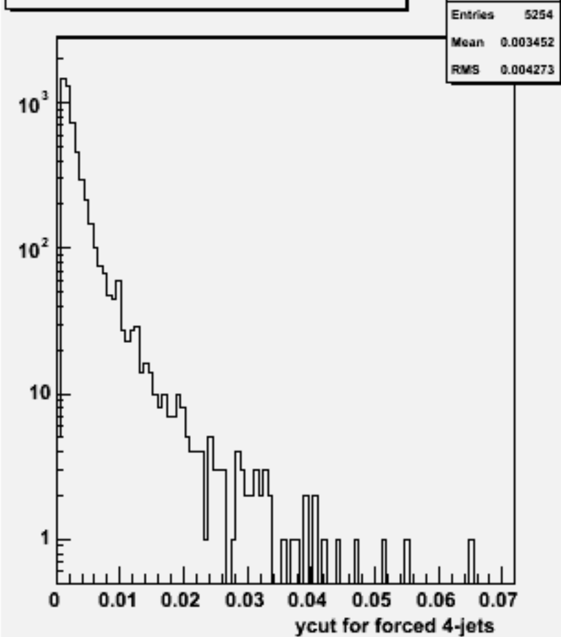
Ycut for 4-jets :w103908 ae1_e1e3e3e3e3_o
