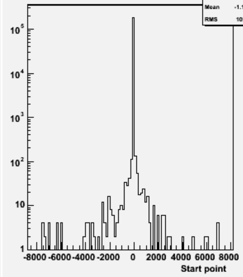
Start point Z : w103908 ae1_e1e3e3e3e3_o
