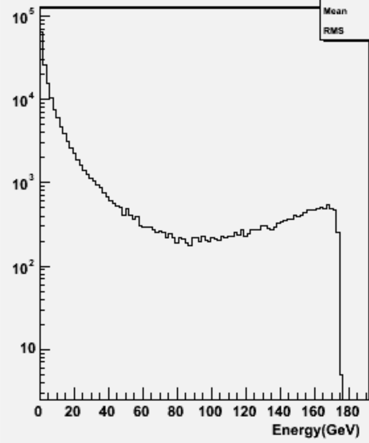
Start point R : w103908 ae1_e1e3e3e3e3_o
