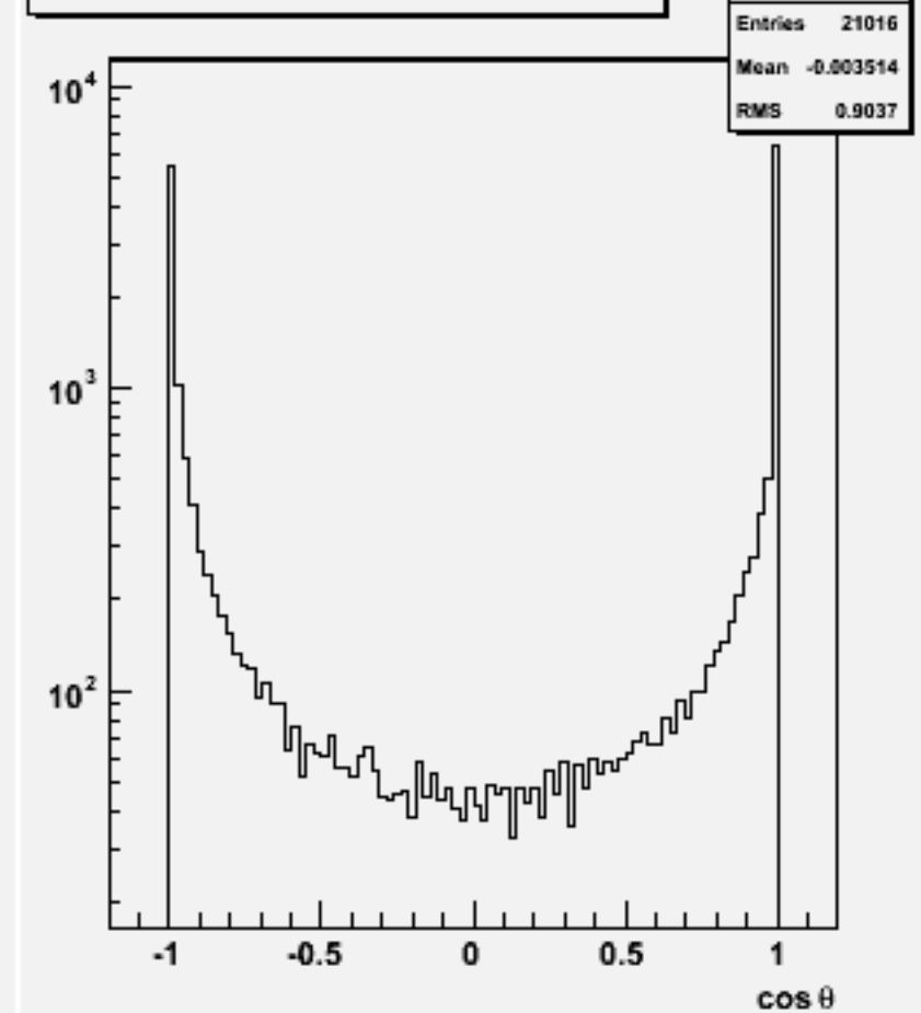
Jet cos \theta (All jets)w103908 ae1_e1e3e3e3e3_o
