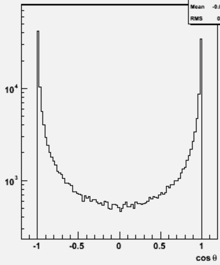
Particle cos θ : w103908 ae1_e1e3e3e3e3_o
