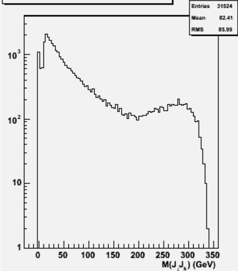
2jets mass(All comb)w103908 ae1_e1e3e3e3e3_o
