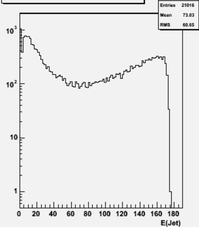
Jet energies(All jets)w103908 ae1_e1e3e3e3e3_o
