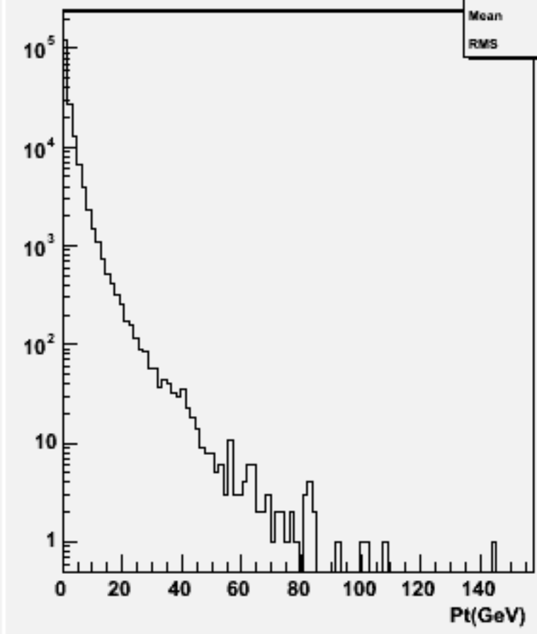
Start point Z : w103908 ae1_e1e3e3e3e3_o
