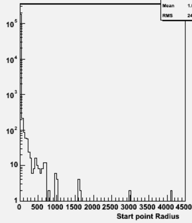
Start point R : w103908 ae1_e1e3e3e3e3_o
