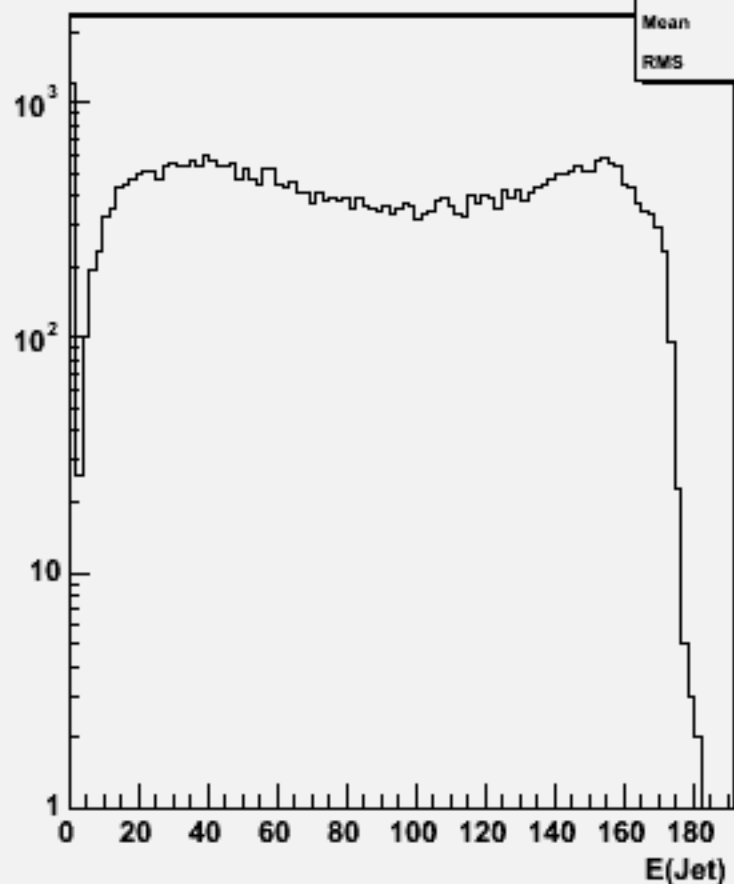
Jet energies(All jets)w103906 ae1_e1e2e2bb_o
