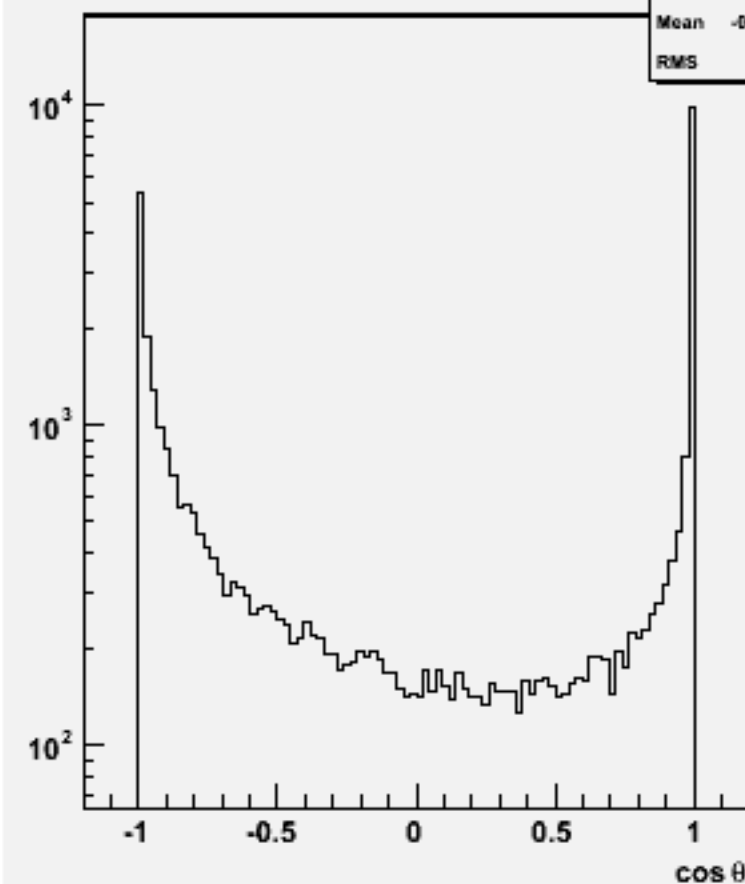
Jet cos \theta (All jets)w103906 ae1_e1e2e2bb_o
