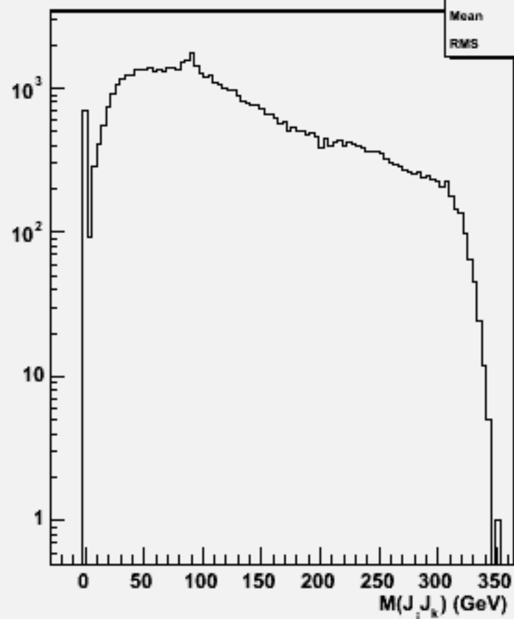
2jets mass(All comb)w103906 ae1_e1e2e2bb_o
