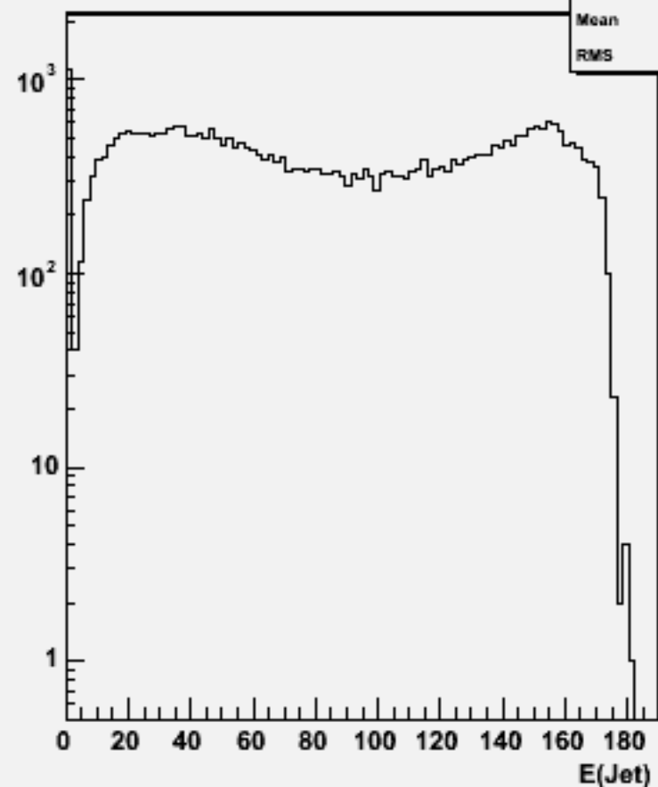
Jet energies(All jets)w103904 ae1_e1e2e2bb_o
