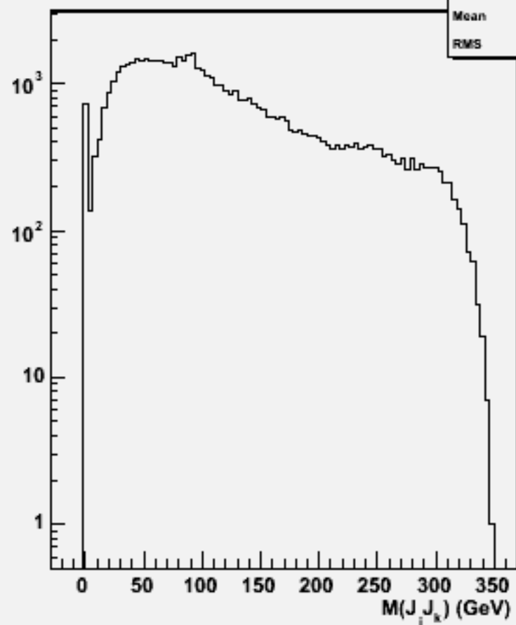
2jets mass(All comb)w103904 ae1_e1e2e2bb_o
