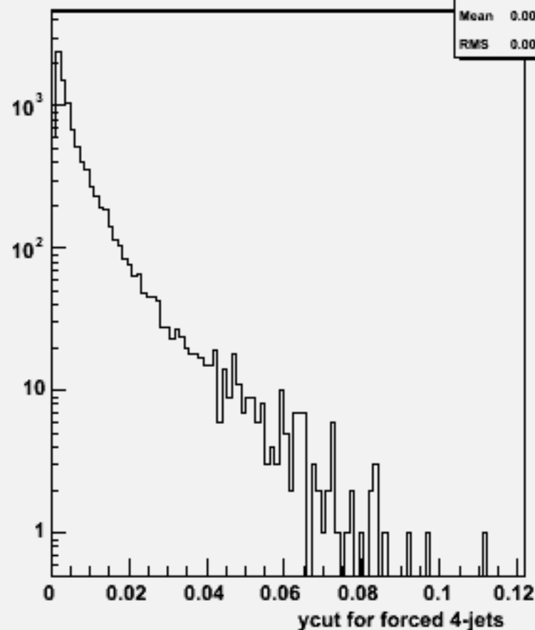
Ycut for 4-jets :w103904 ae1_e1e2e2bb_o
