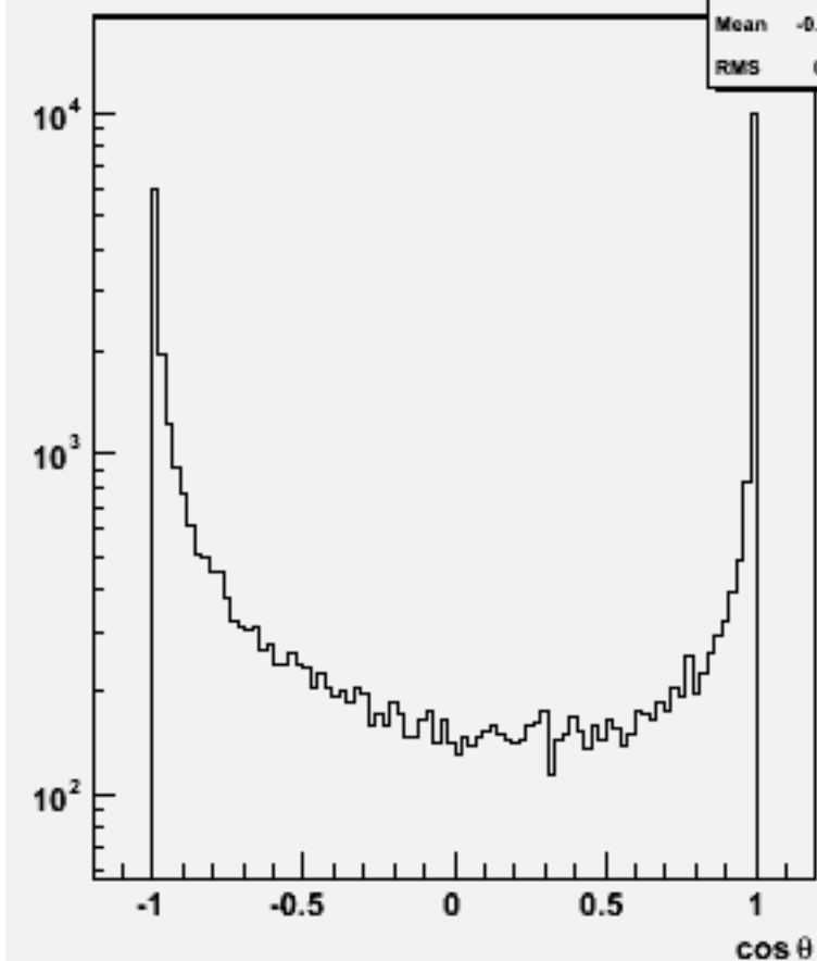
Jet cos \theta (All jets)w103904 ae1_e1e2e2bb_o
